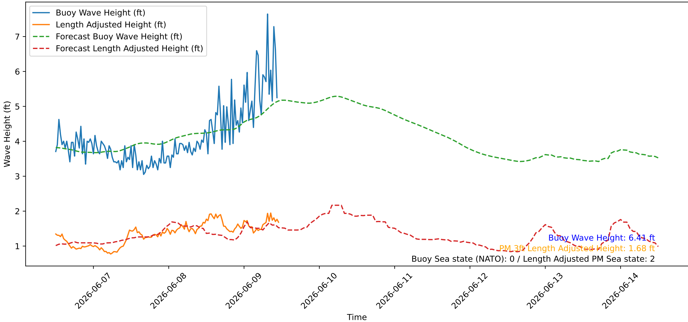
Wave Heights over Time for Red Beach at 2026-06-09 11:40:45
