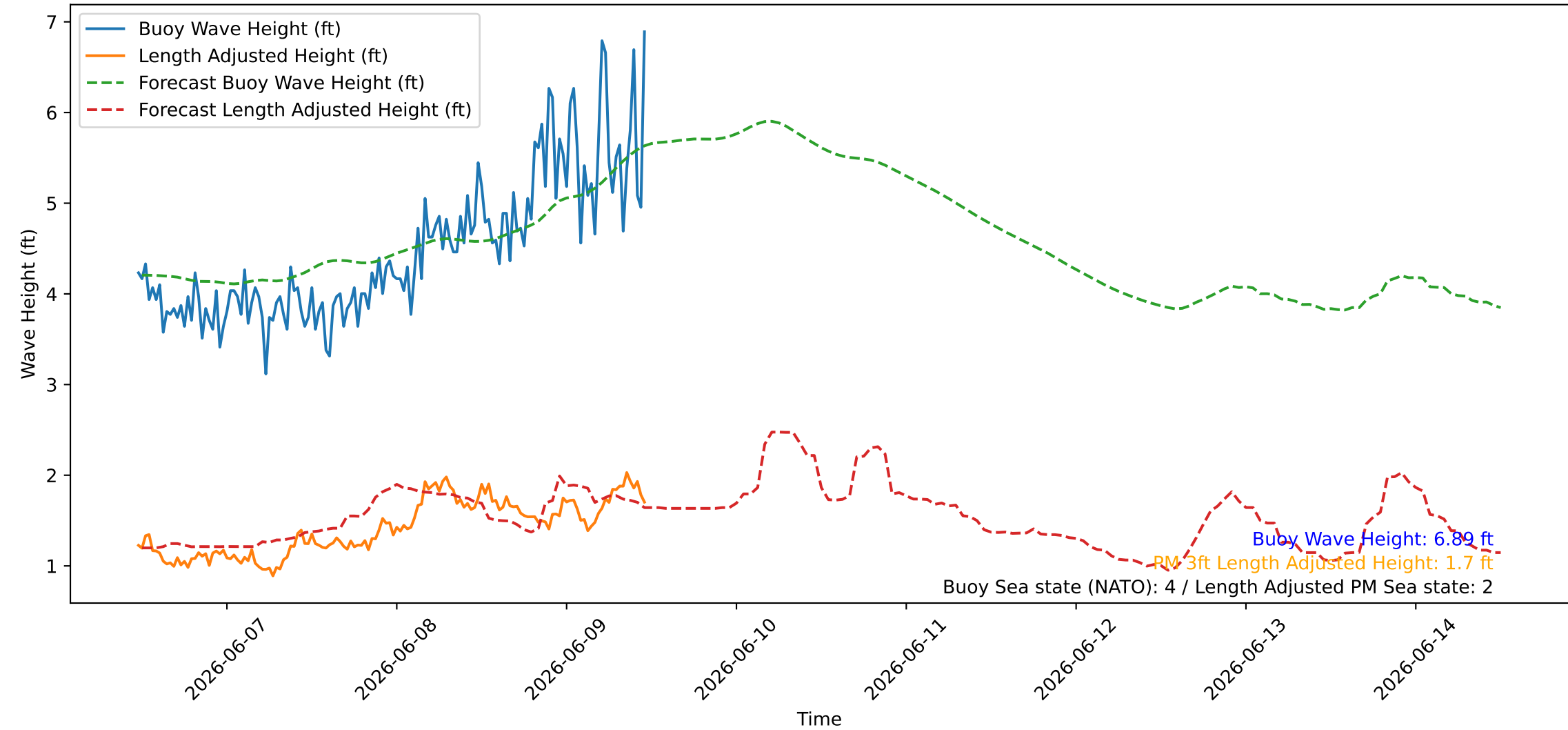
Wave Heights over Time for Green Beach at 2026-06-09 11:41:07
