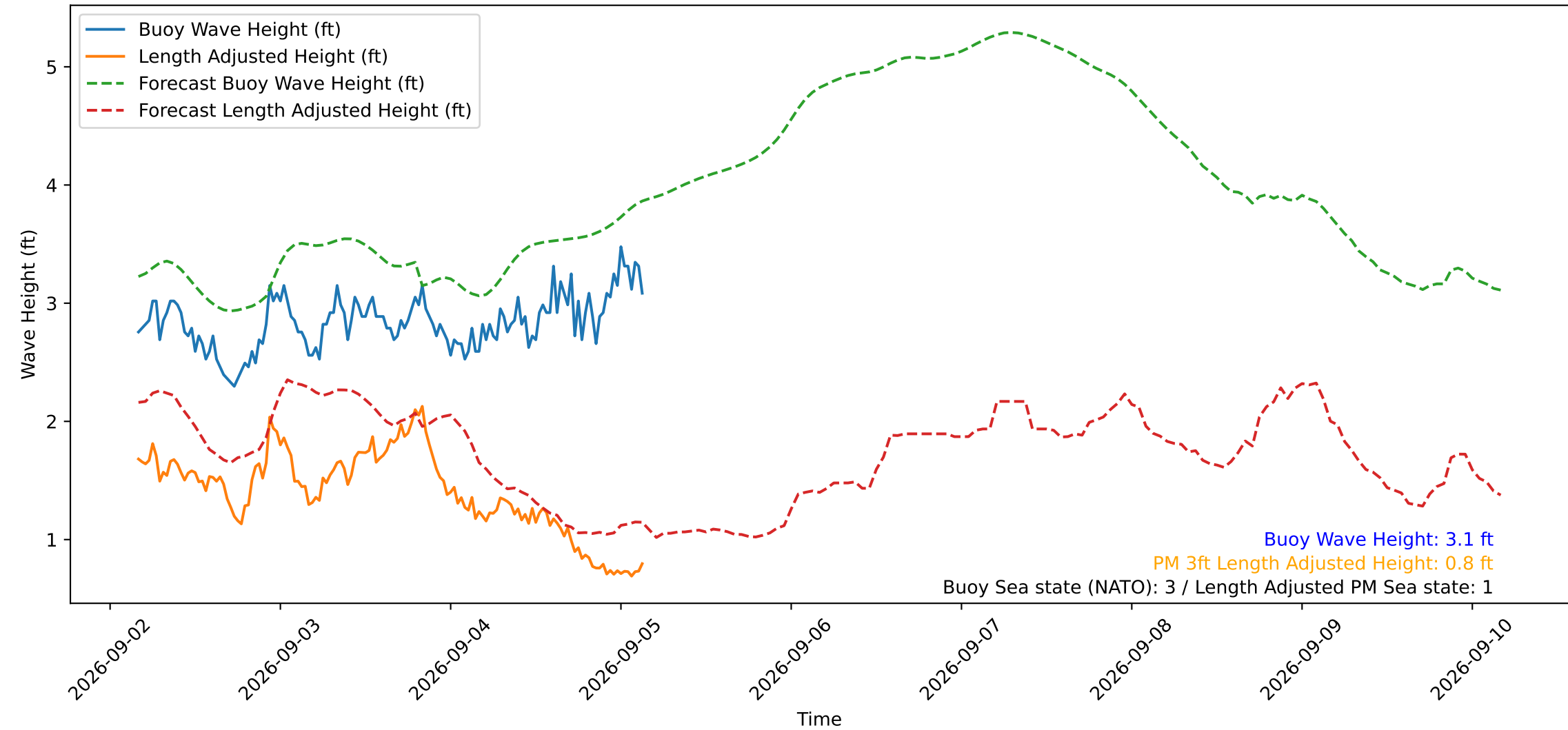
Wave Heights over Time for Red Beach at 2026-09-05 03:50:51
