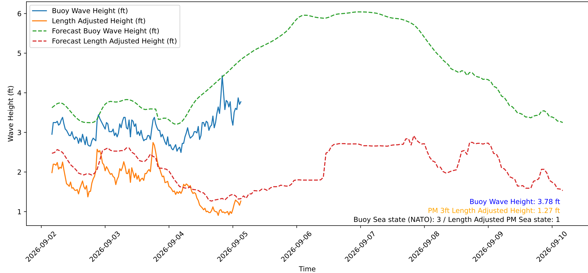
Wave Heights over Time for Green Beach at 2026-09-05 03:51:15
