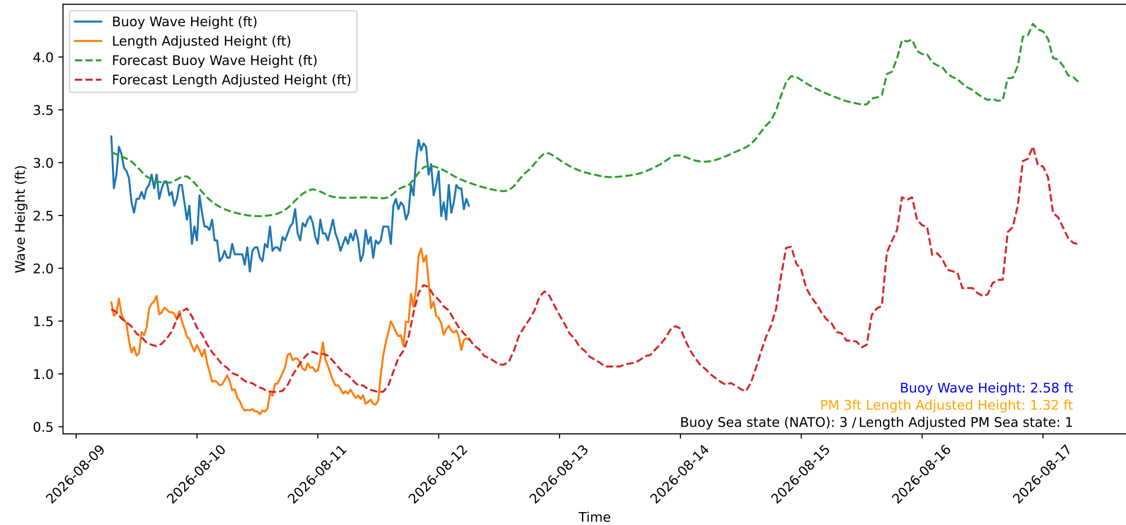
Wave Heights over Time for Green Beach at 2026-08-12 06:51:08
