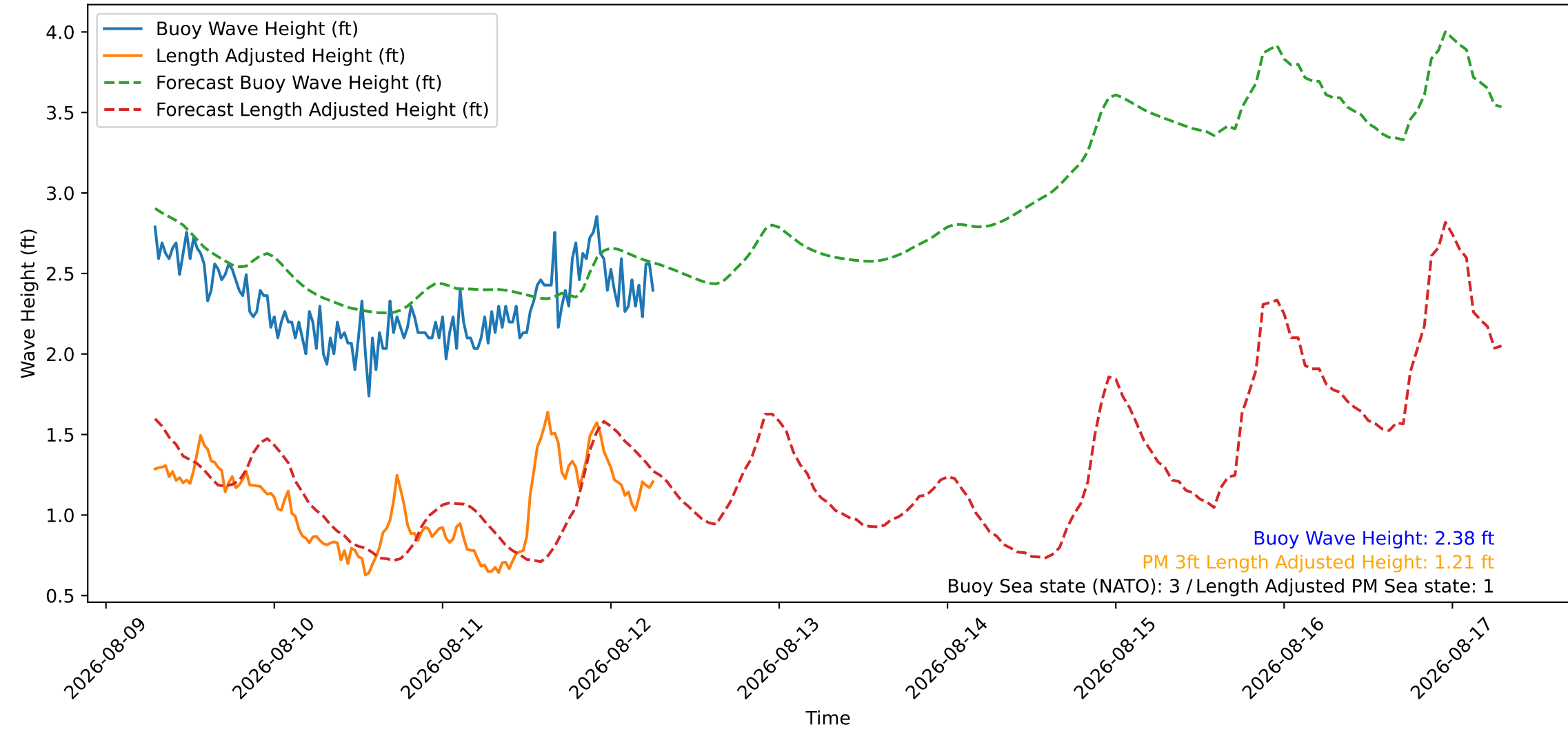
Wave Heights over Time for Red Beach at 2026-08-12 06:50:46
