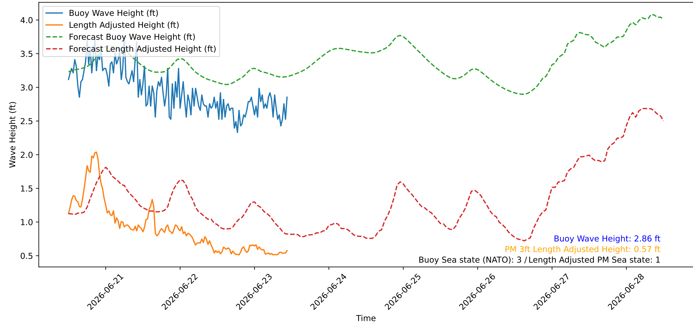
Wave Heights over Time for Red Beach at 2026-06-23 11:30:45
