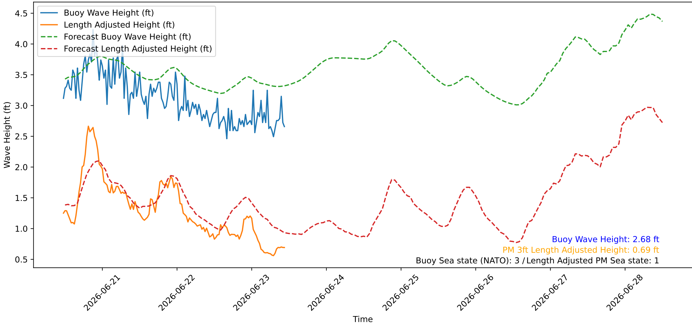
Wave Heights over Time for Green Beach at 2026-06-23 11:31:08
