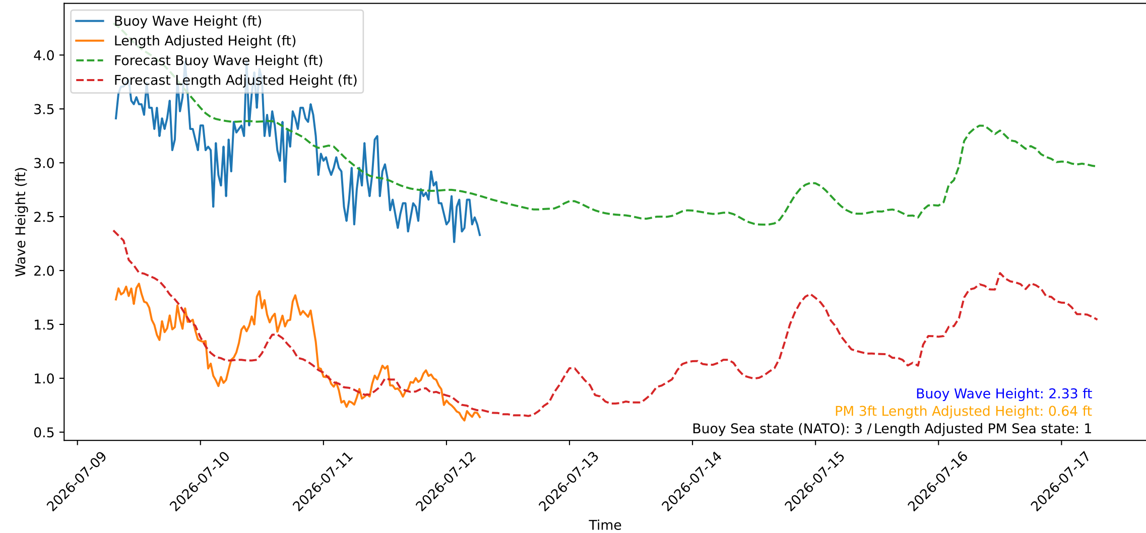
Wave Heights over Time for Red Beach at 2026-07-12 07:20:47
