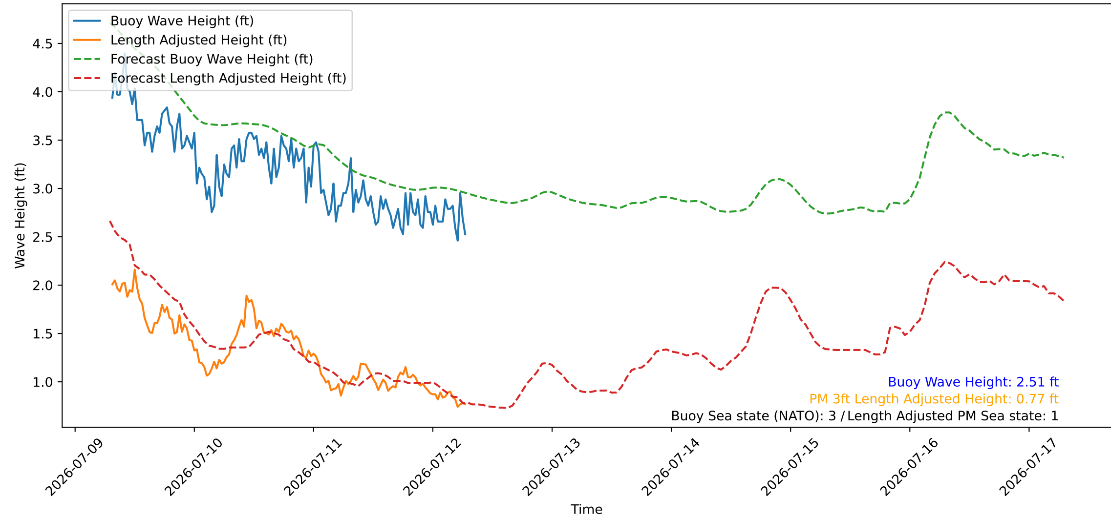
Wave Heights over Time for Green Beach at 2026-07-12 07:21:09
