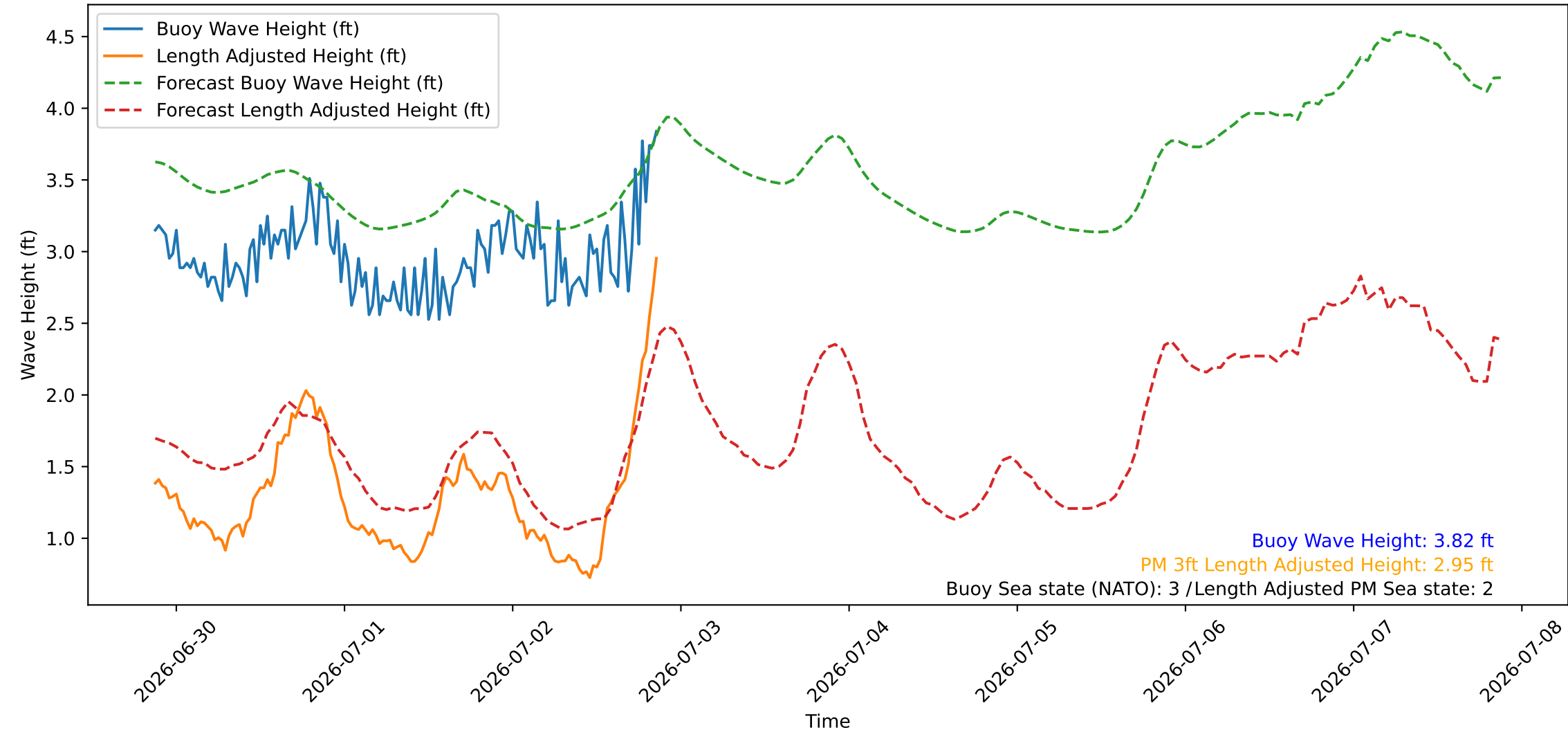
Wave Heights over Time for Green Beach at 2026-07-02 21:11:09
