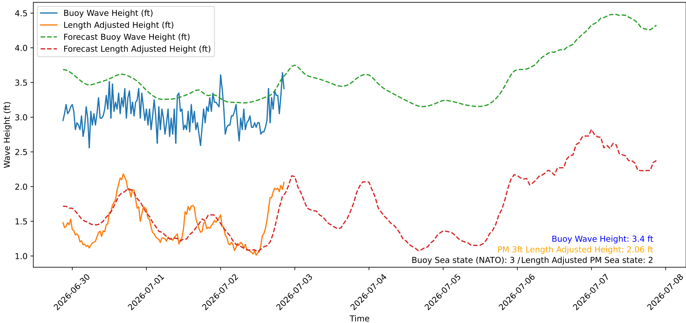
Wave Heights over Time for Oceanside Harbor at 2026-07-02 21:10:27
