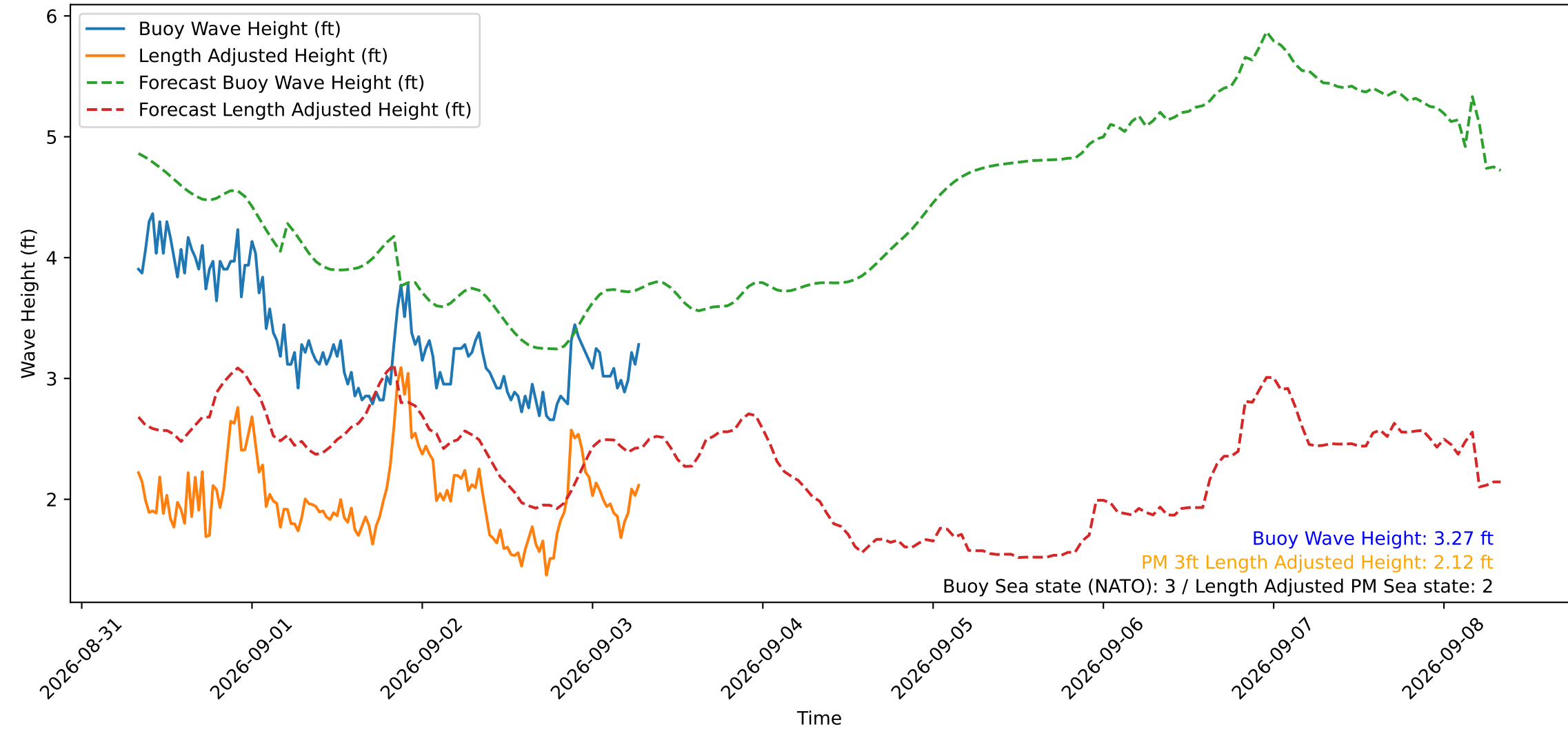
Wave Heights over Time for Green Beach at 2026-09-03 07:31:11
