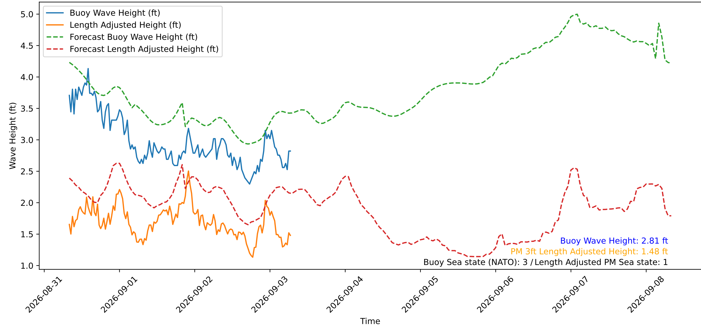
Wave Heights over Time for Red Beach at 2026-09-03 07:30:49
