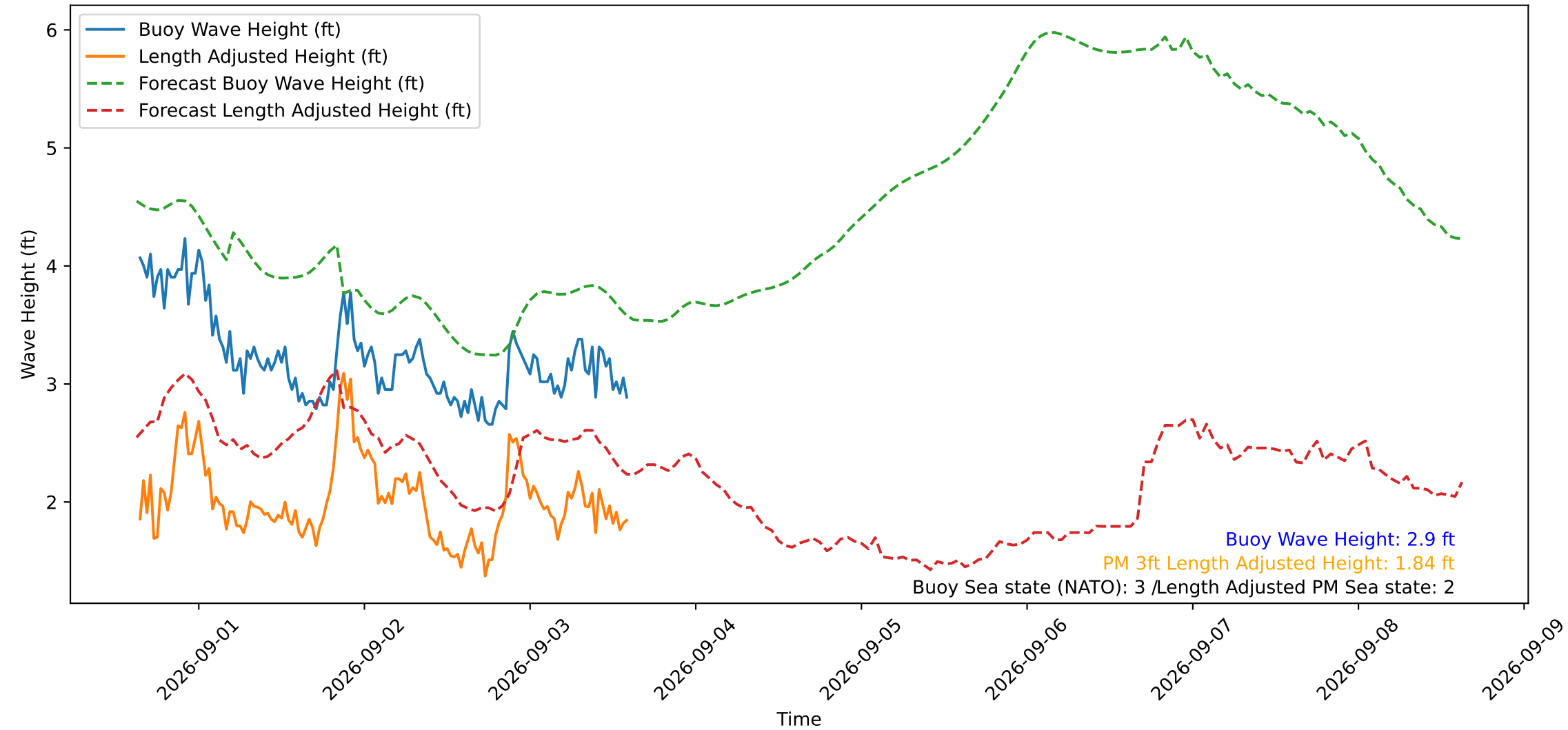
Wave Heights over Time for Green Beach at 2026-09-03 15:01:12
