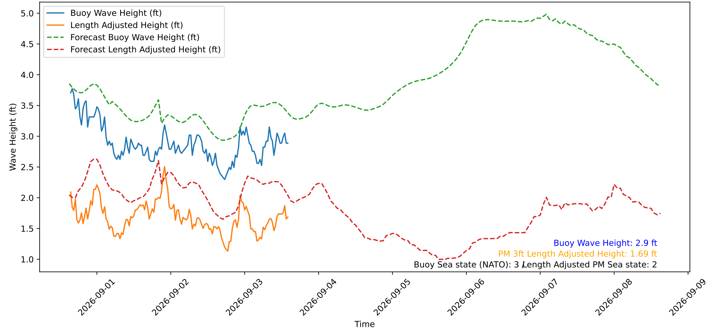
Wave Heights over Time for Red Beach at 2026-09-03 15:00:49
