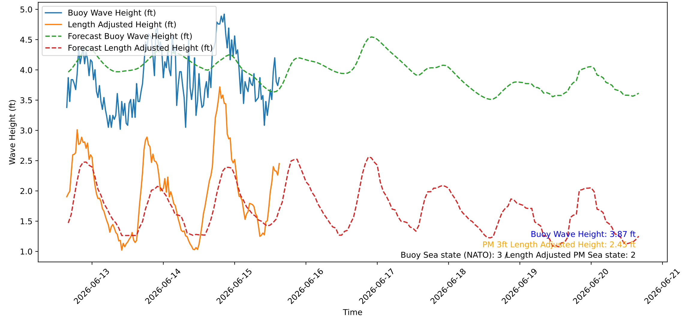
Wave Heights over Time for Green Beach at 2026-06-15 15:41:08
