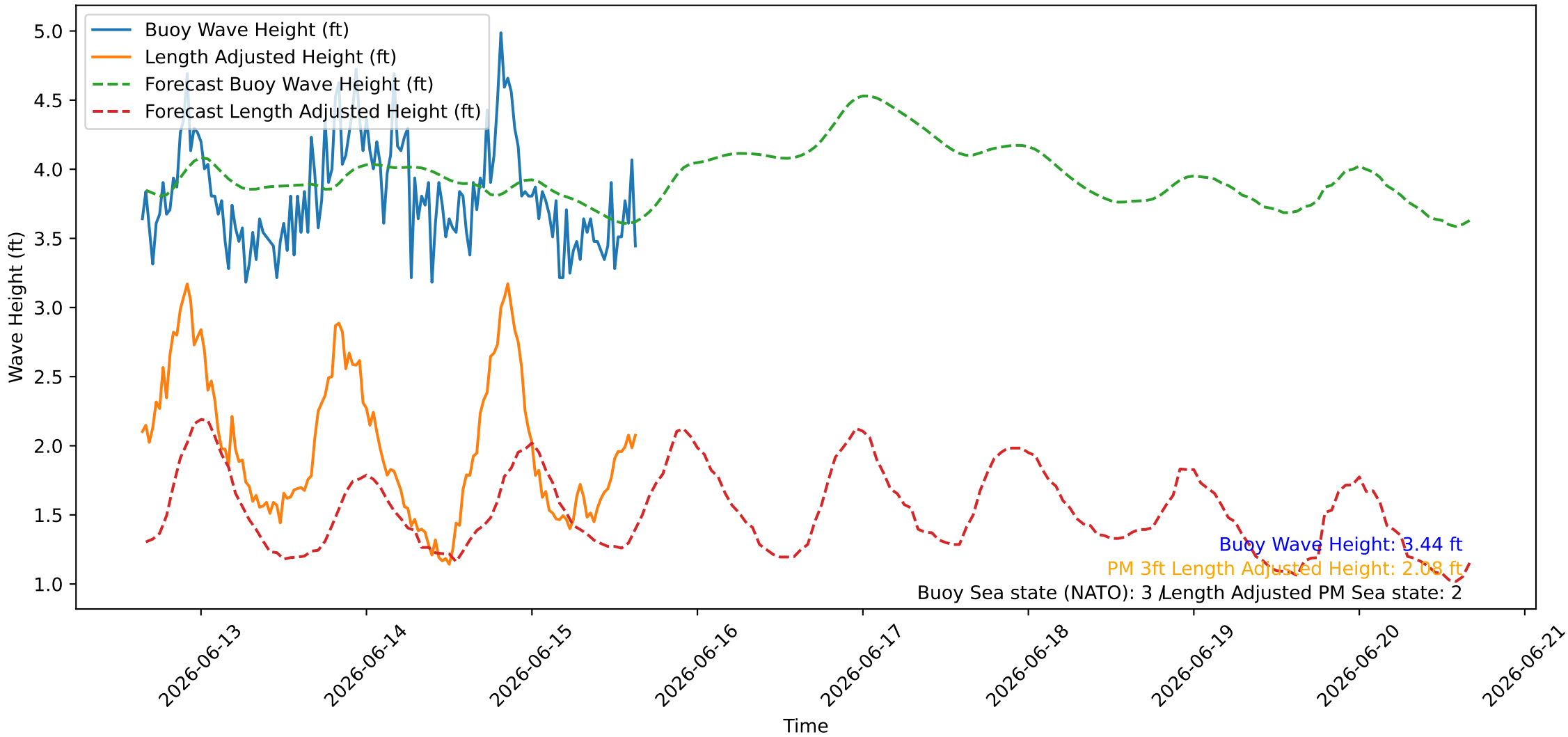
Wave Heights over Time for Oceanside Harbor at 2026-06-15 15:40:26
