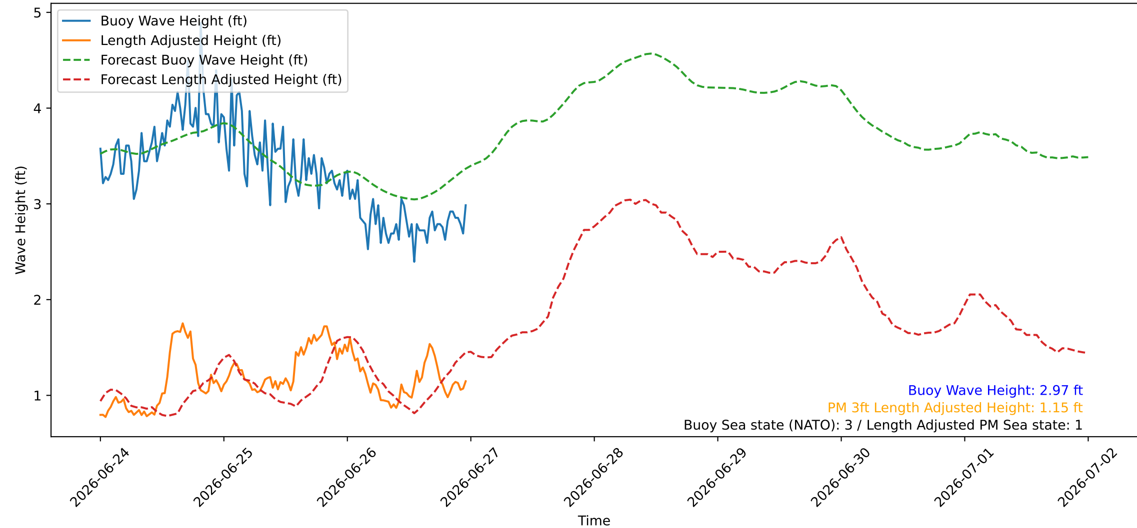
Wave Heights over Time for Oceanside Harbor at 2026-06-27 00:00:26
