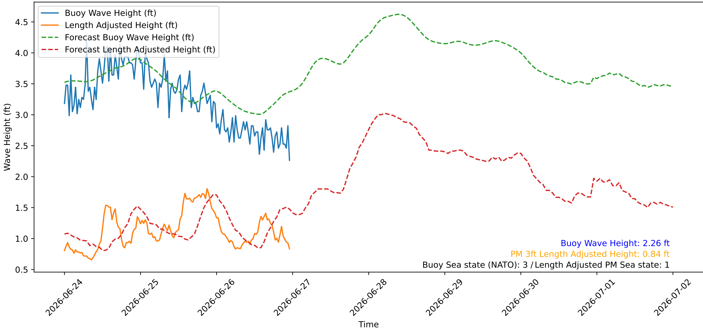
Wave Heights over Time for Green Beach at 2026-06-27 00:01:07
