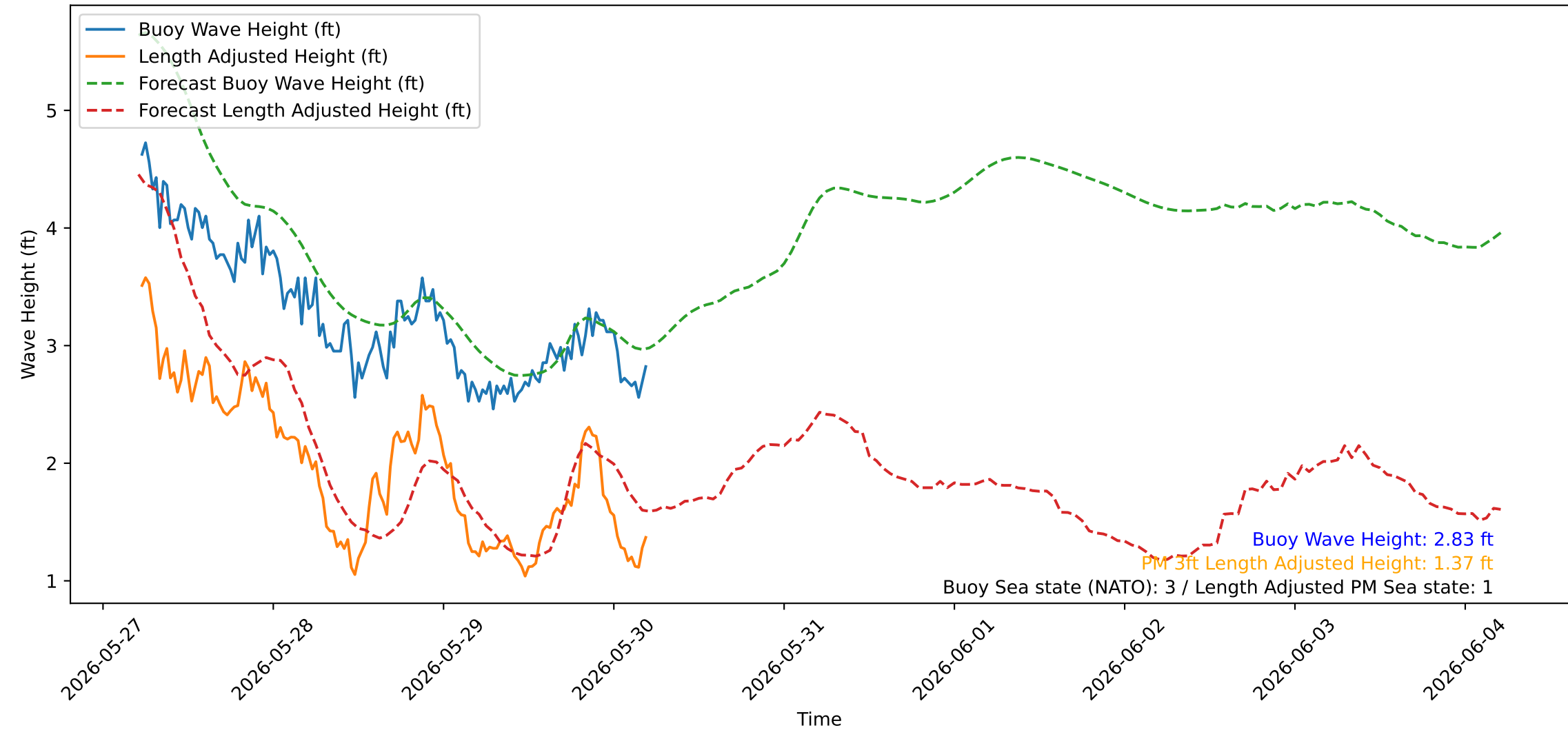
Wave Heights over Time for Green Beach at 2026-05-30 05:21:06
