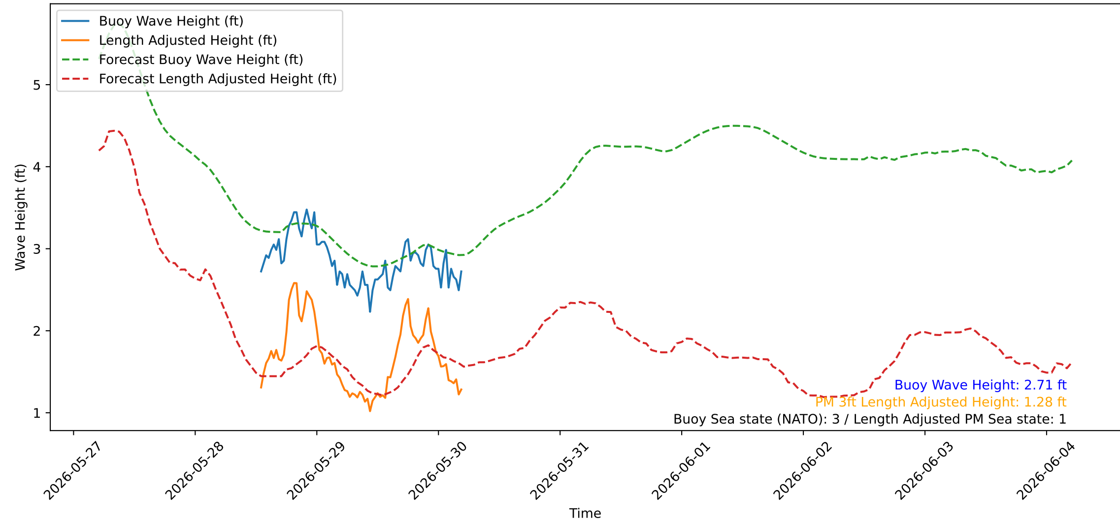
Wave Heights over Time for Oceanside Harbor at 2026-05-30 05:20:23
