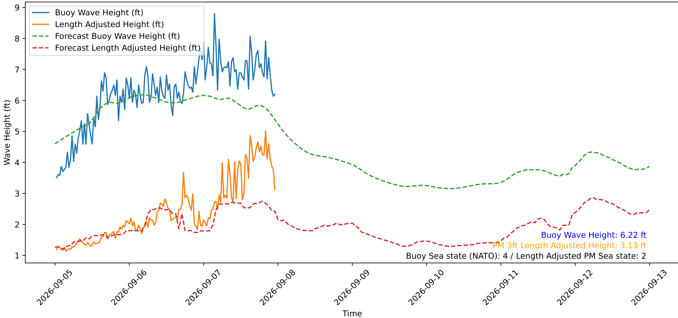
Wave Heights over Time for Green Beach at 2026-09-08 00:01:12
