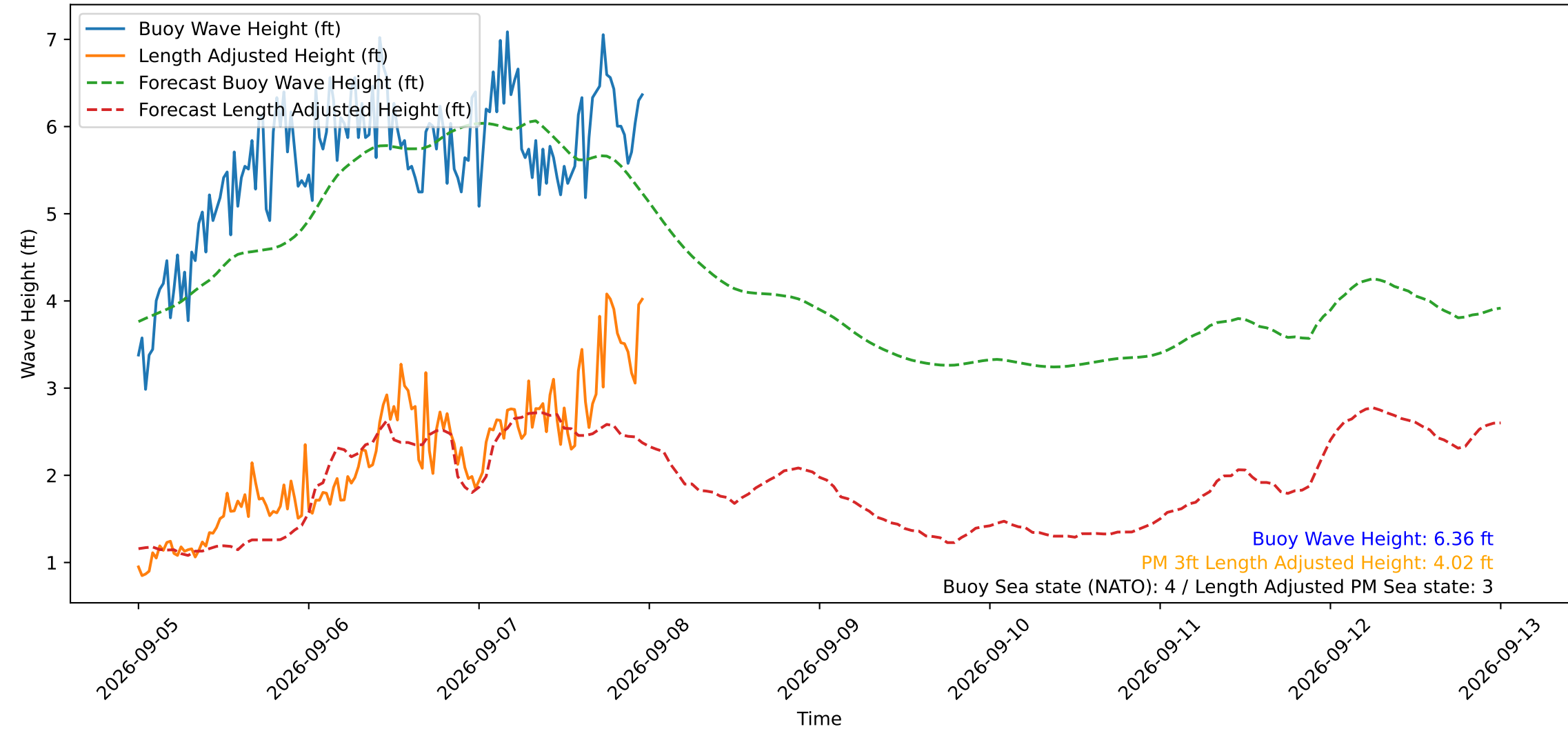
Wave Heights over Time for Oceanside Harbor at 2026-09-08 00:00:29
