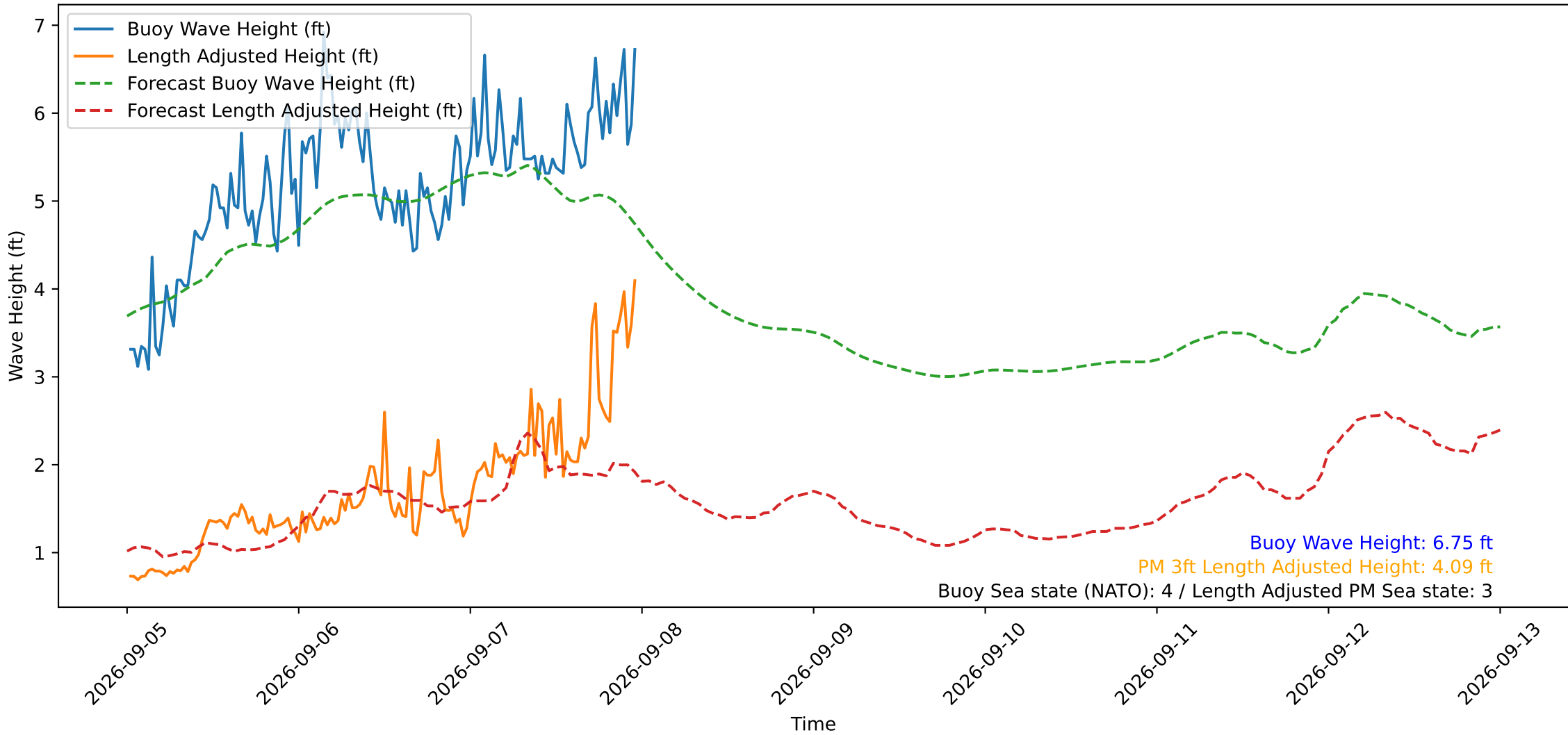
Wave Heights over Time for Red Beach at 2026-09-08 00:00:49
