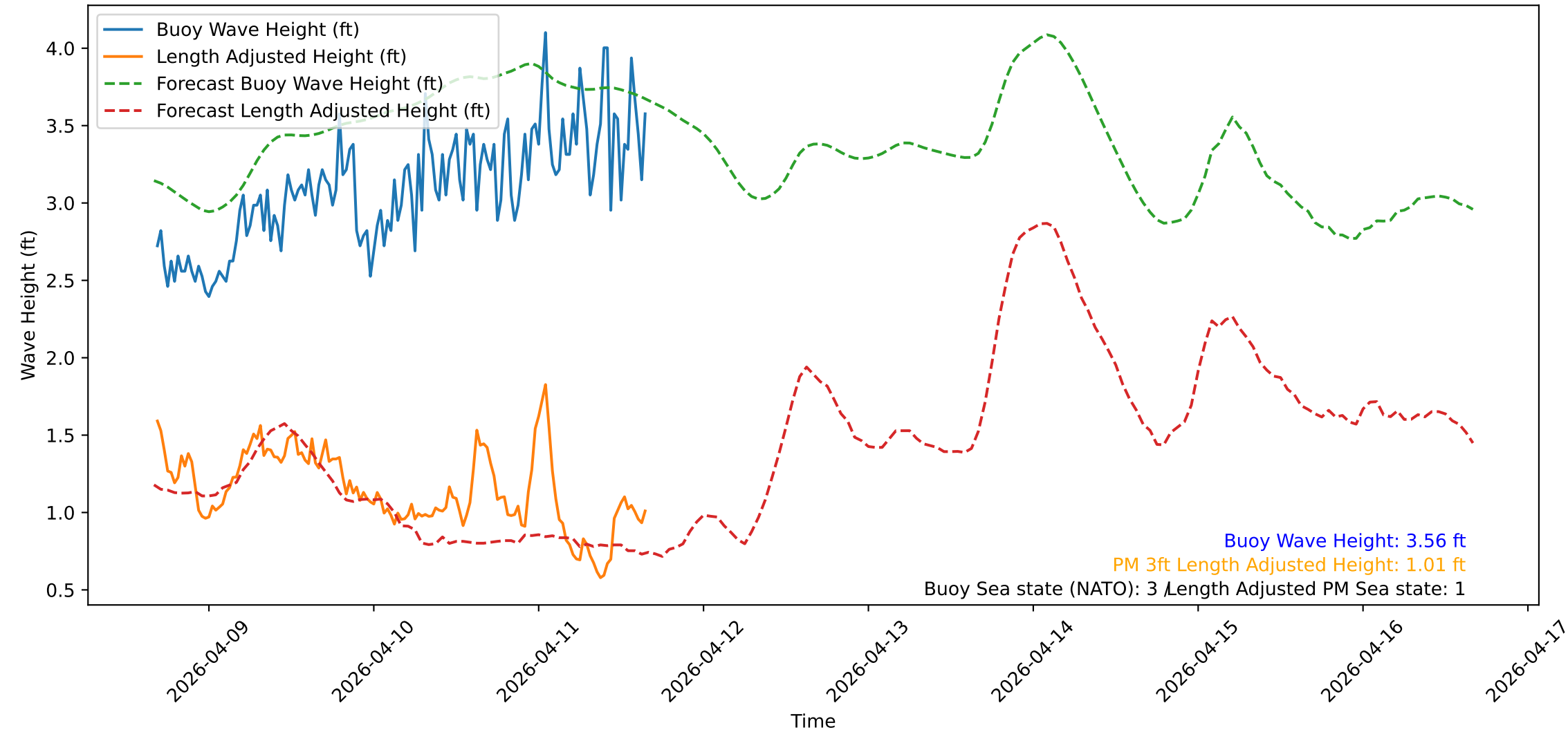
Wave Heights over Time for Red Beach at 2026-04-11 16:20:52
