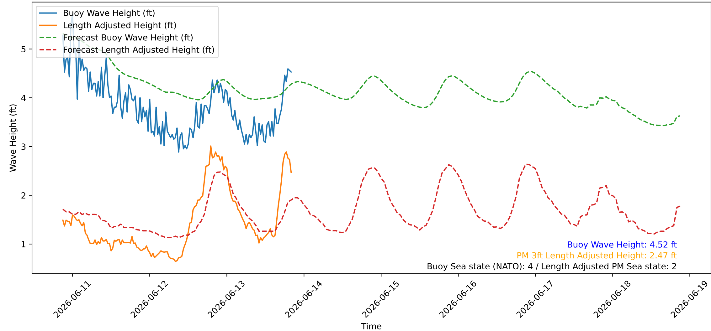
Wave Heights over Time for Green Beach at 2026-06-13 20:51:10
