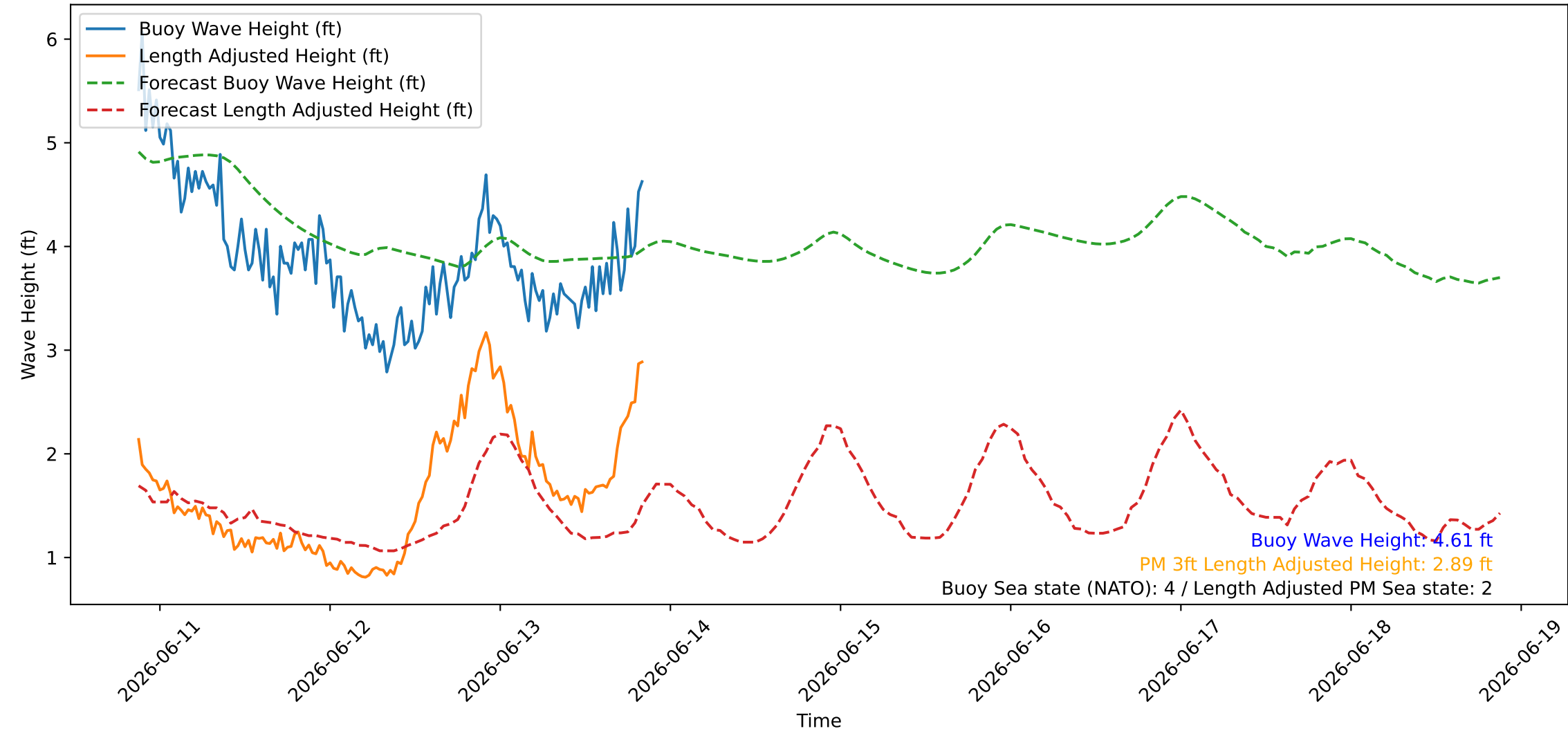
Wave Heights over Time for Oceanside Harbor at 2026-06-13 20:50:26
