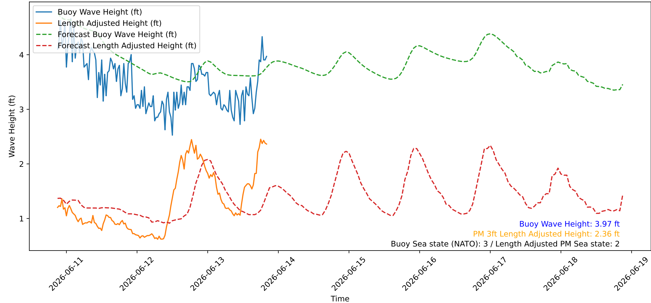
Wave Heights over Time for Red Beach at 2026-06-13 20:50:47
