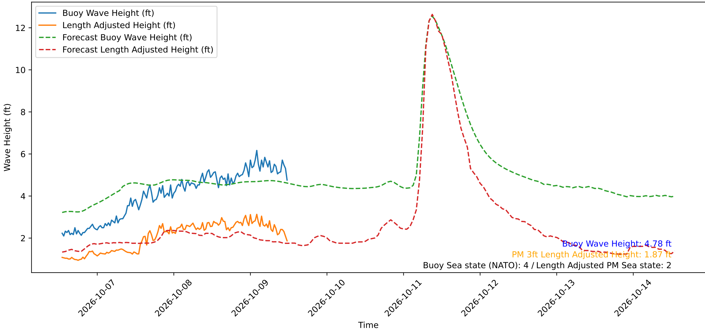
Wave Heights over Time for Green Beach at 2026-10-09 12:31:13
