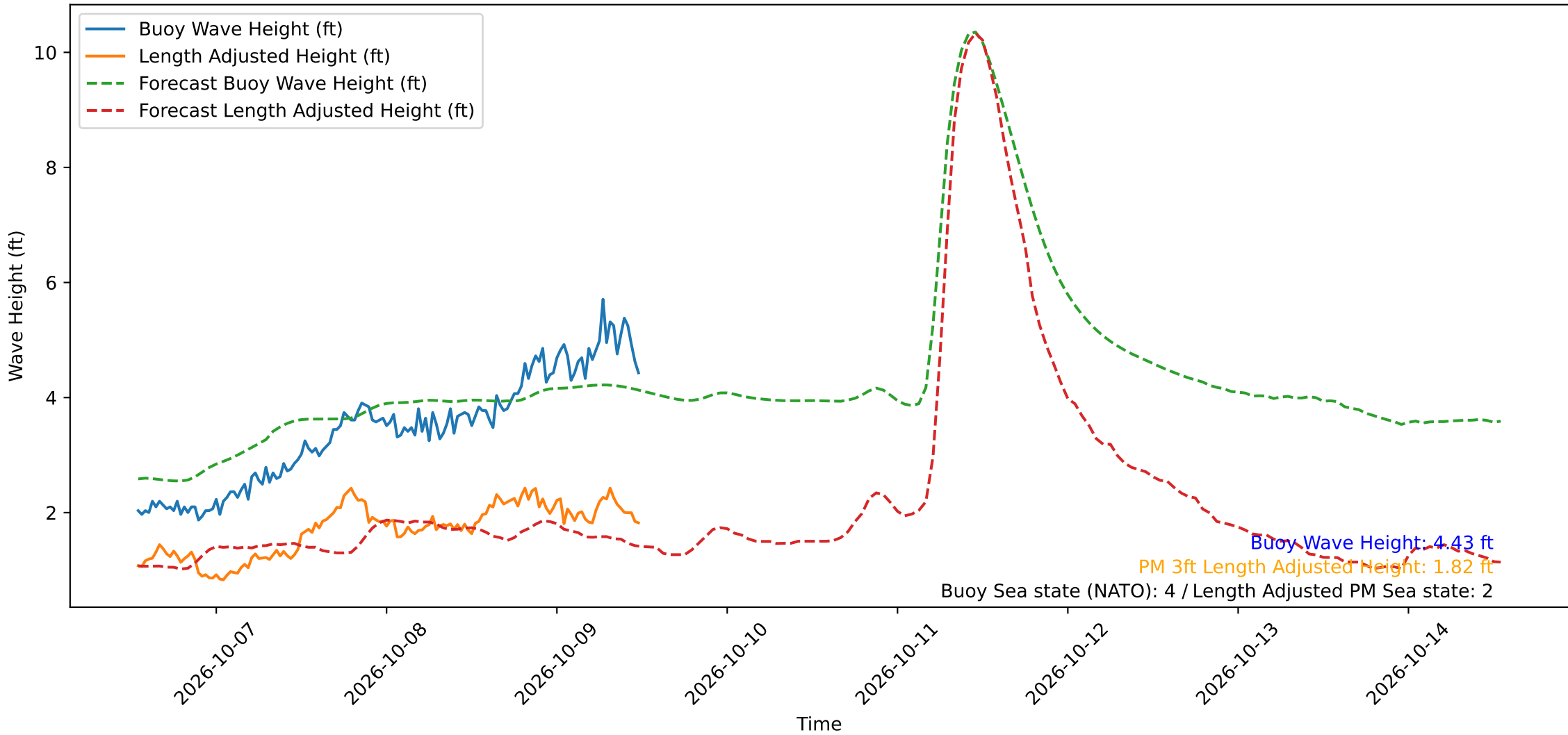
Wave Heights over Time for Red Beach at 2026-10-09 12:30:50
