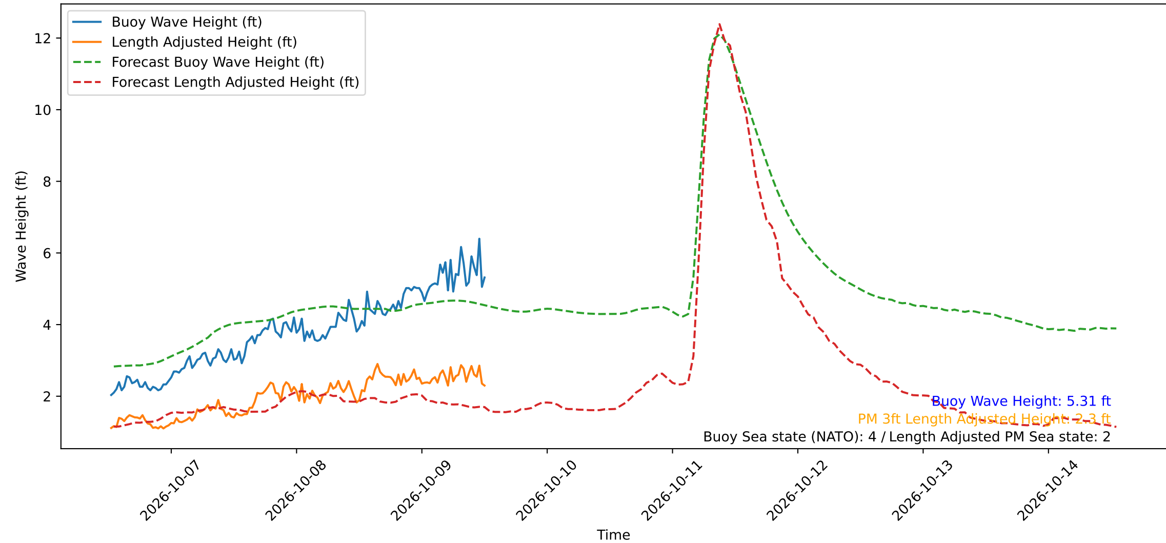
Wave Heights over Time for Oceanside Harbor at 2026-10-09 12:30:30
