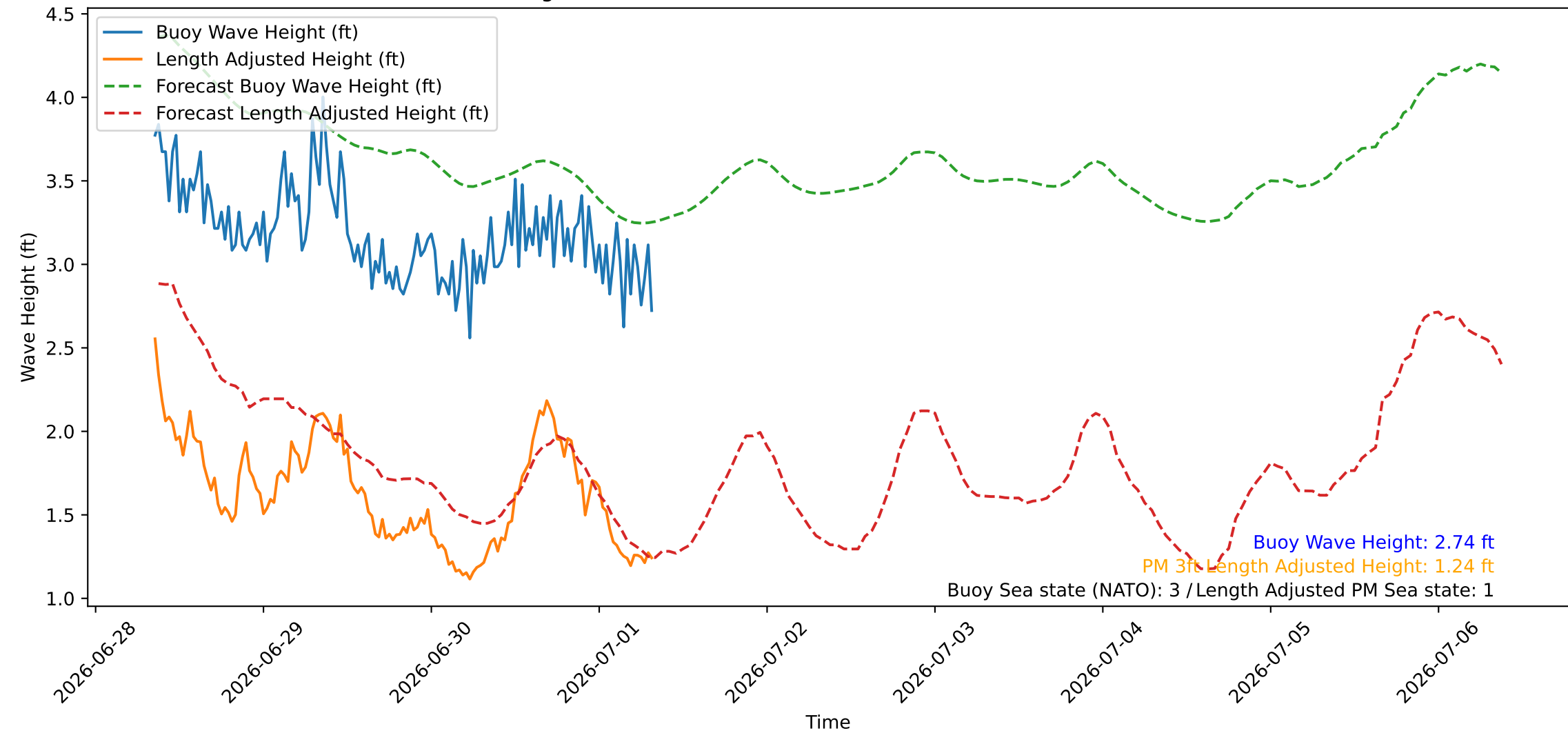
Wave Heights over Time for Oceanside Harbor at 2026-07-01 08:30:26
