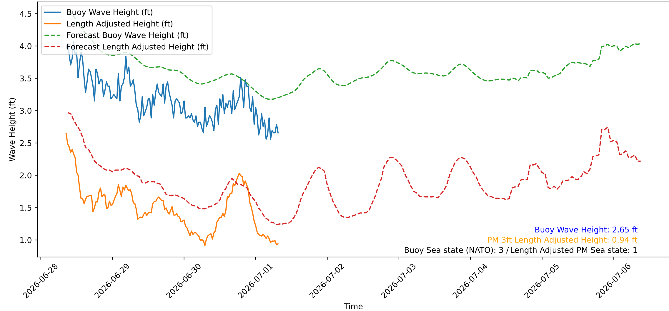
Wave Heights over Time for Green Beach at 2026-07-01 08:31:08
