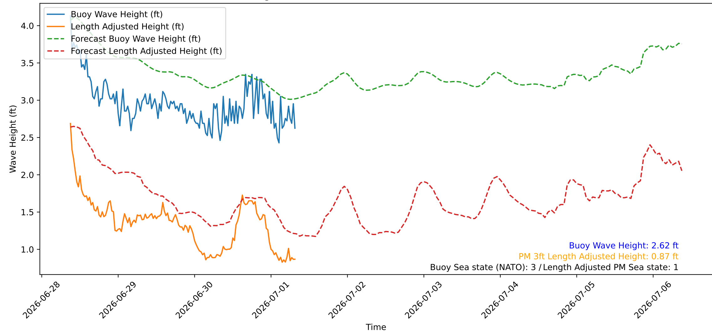
Wave Heights over Time for Red Beach at 2026-07-01 08:30:46
