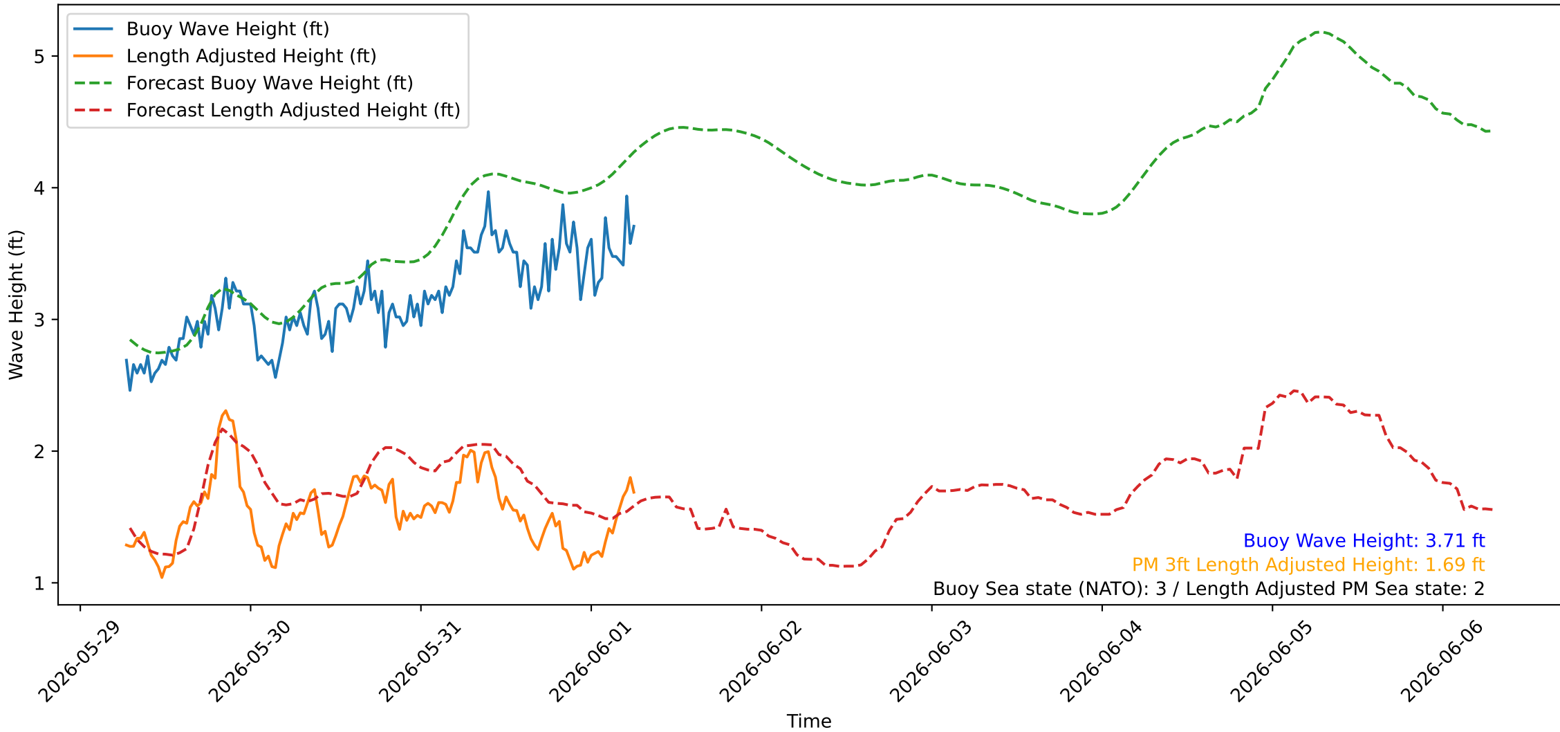
Wave Heights over Time for Green Beach at 2026-06-01 06:41:07
