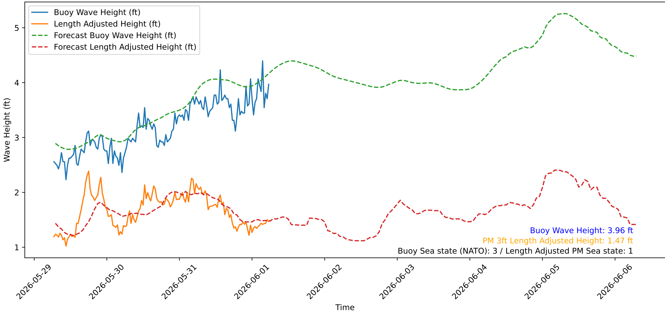
Wave Heights over Time for Oceanside Harbor at 2026-06-01 06:40:25
