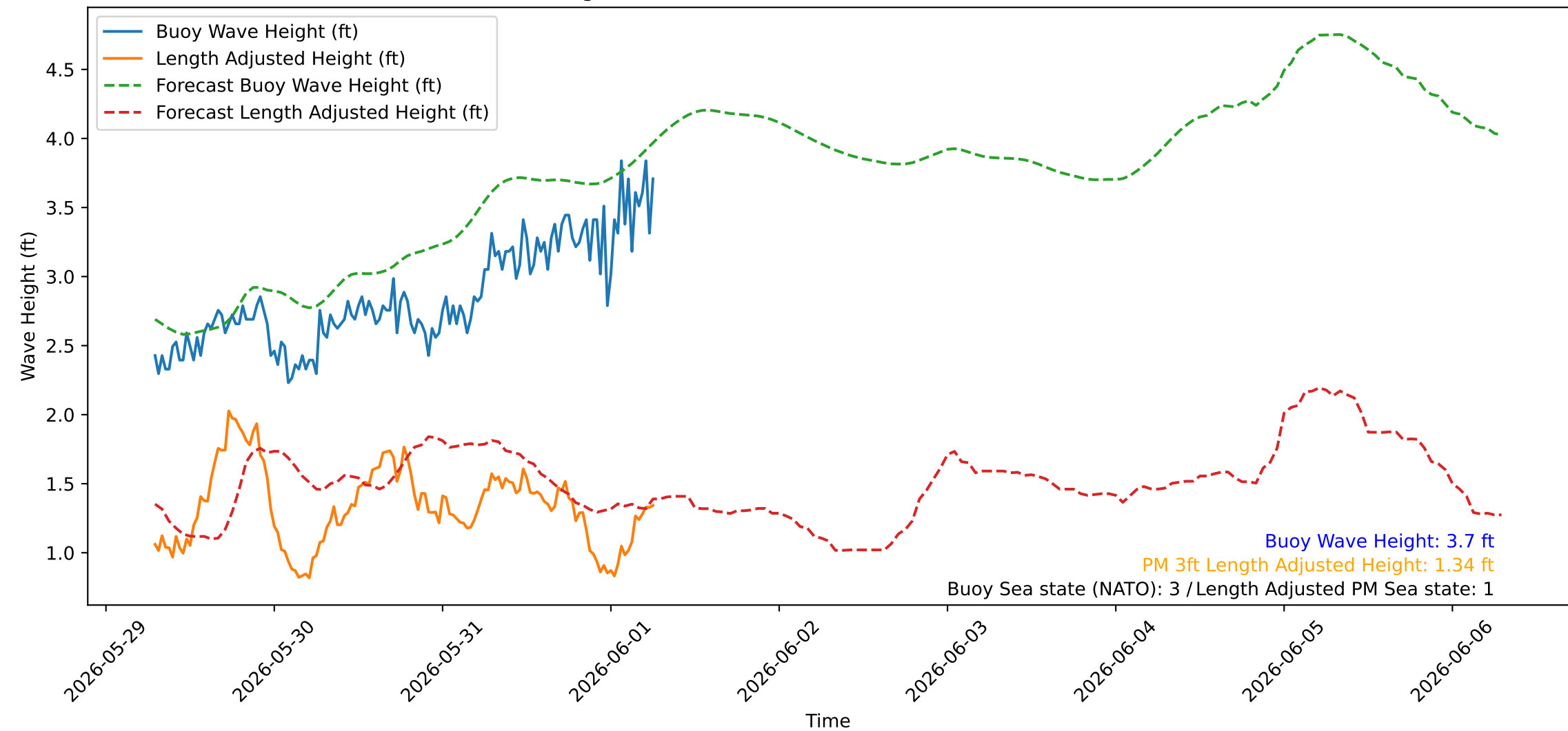
Wave Heights over Time for Red Beach at 2026-06-01 06:40:44
