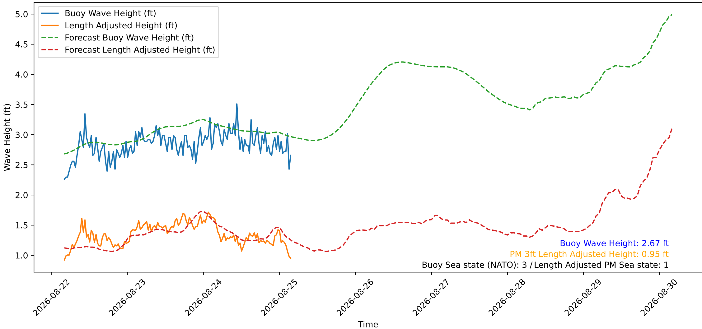
Wave Heights over Time for Oceanside Harbor at 2026-08-25 04:10:30
