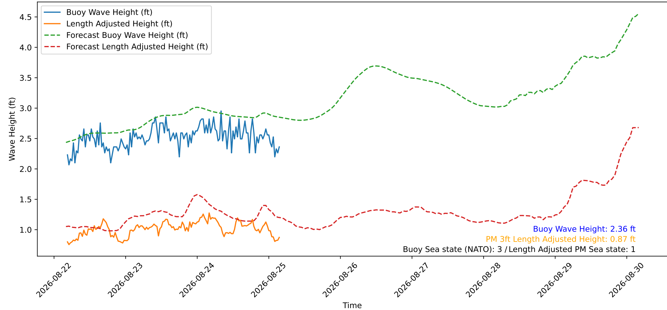
Wave Heights over Time for Red Beach at 2026-08-25 04:10:49
