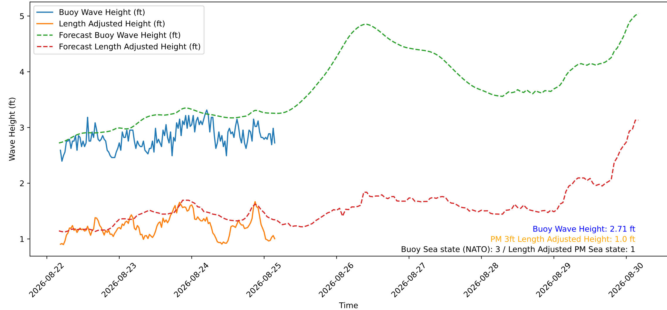
Wave Heights over Time for Green Beach at 2026-08-25 04:11:11
