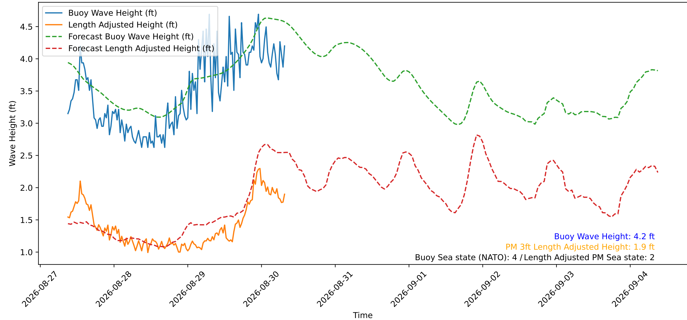
Wave Heights over Time for Red Beach at 2026-08-30 08:30:49
