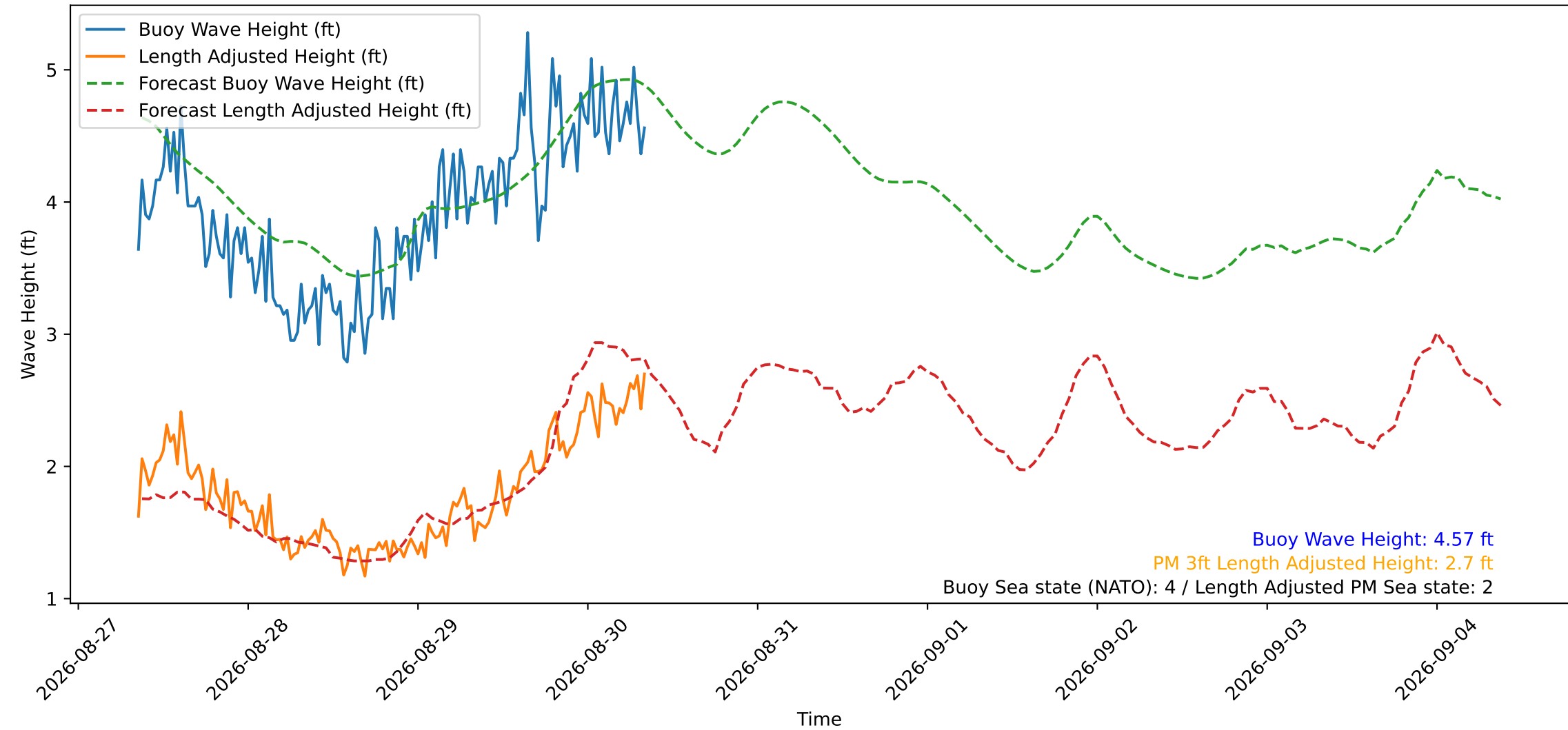
Wave Heights over Time for Oceanside Harbor at 2026-08-30 08:30:29
