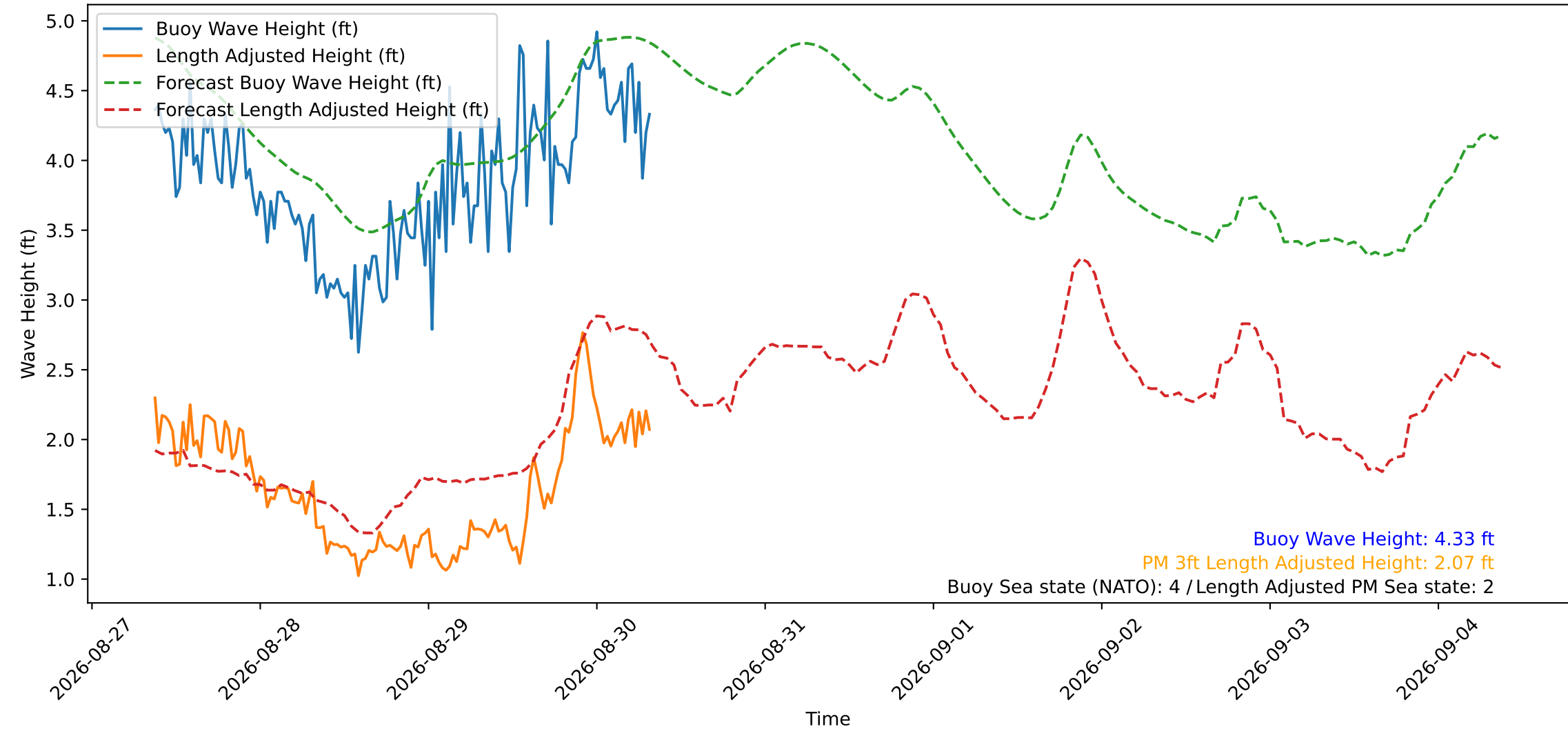
Wave Heights over Time for Green Beach at 2026-08-30 08:31:12
