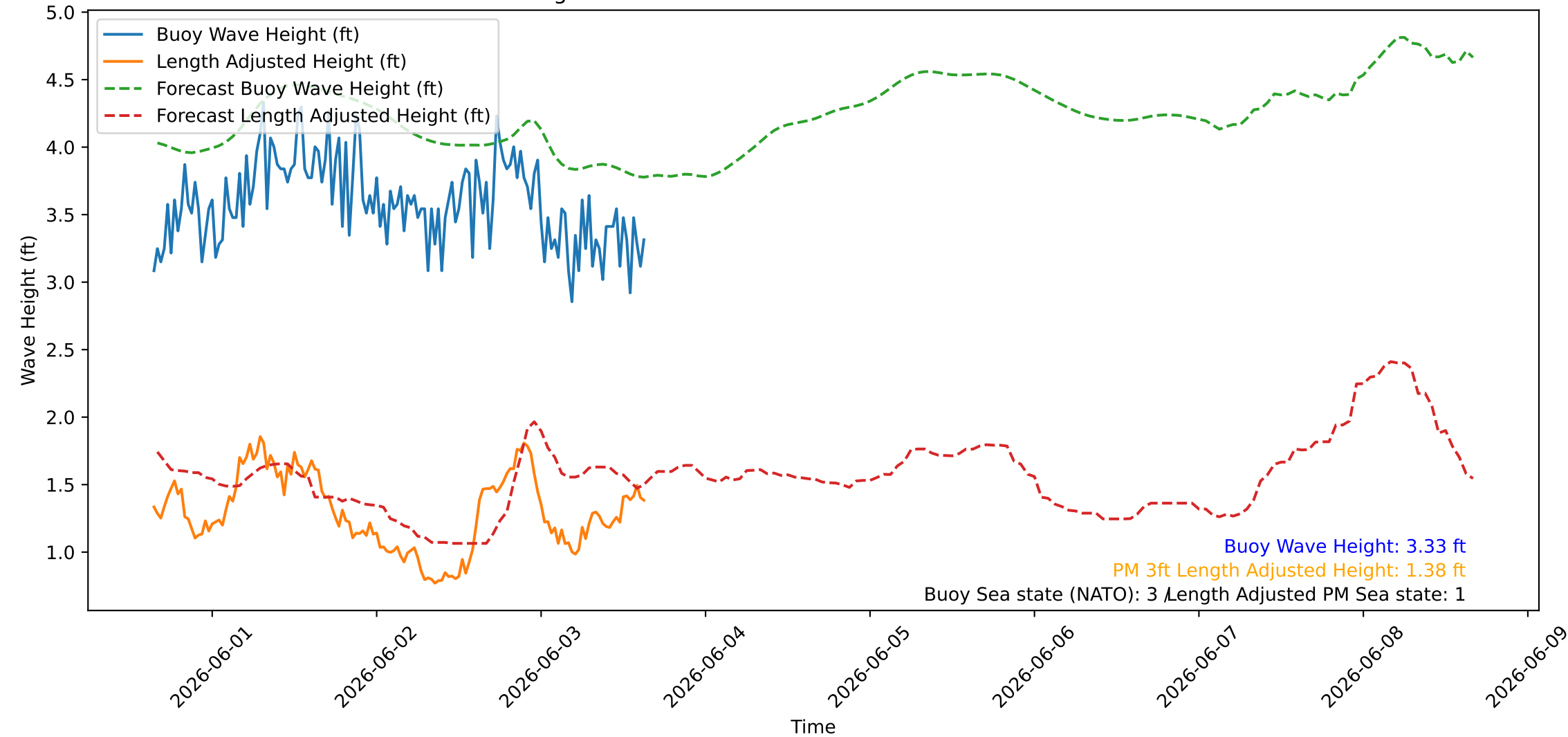
Wave Heights over Time for Green Beach at 2026-06-03 15:41:08
