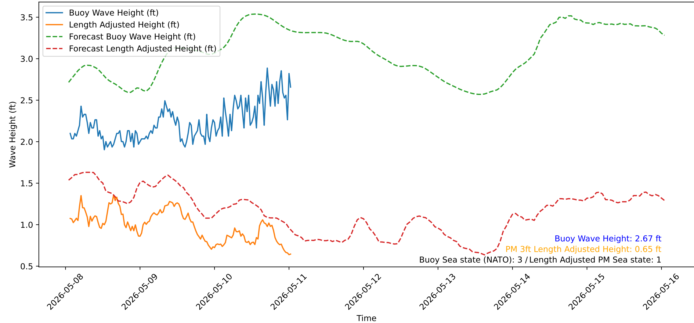
Wave Heights over Time for Red Beach at 2026-05-11 01:20:51
