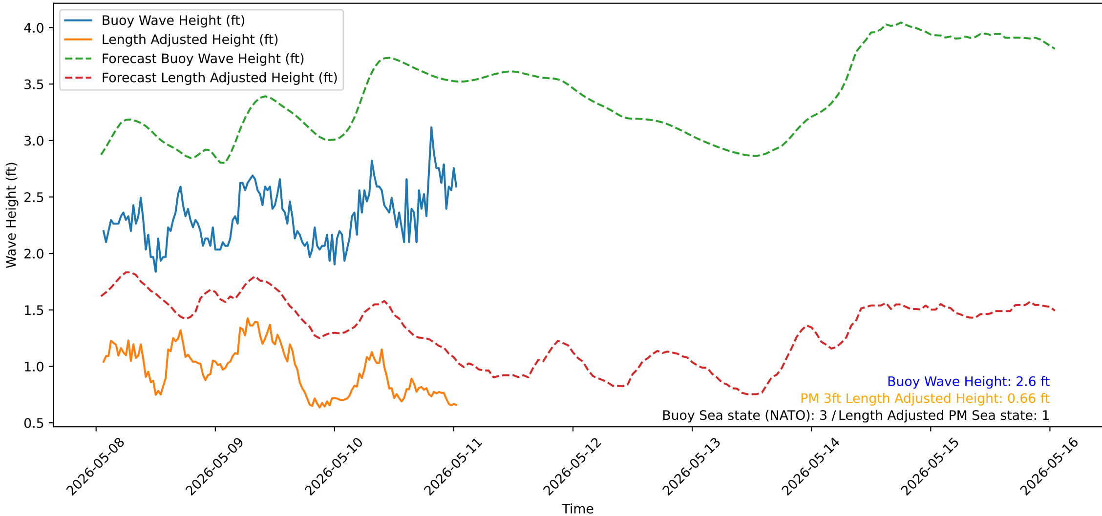
Wave Heights over Time for Green Beach at 2026-05-11 01:21:13
