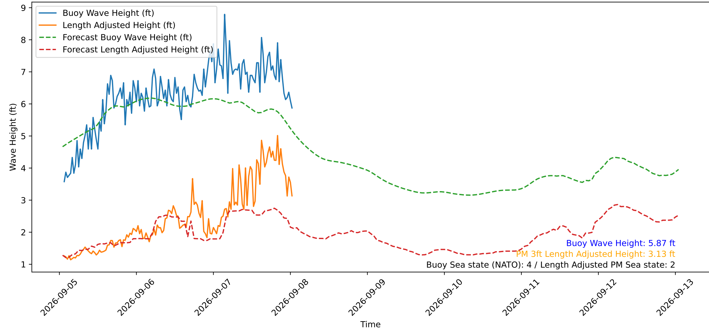
Wave Heights over Time for Green Beach at 2026-09-08 01:21:13
