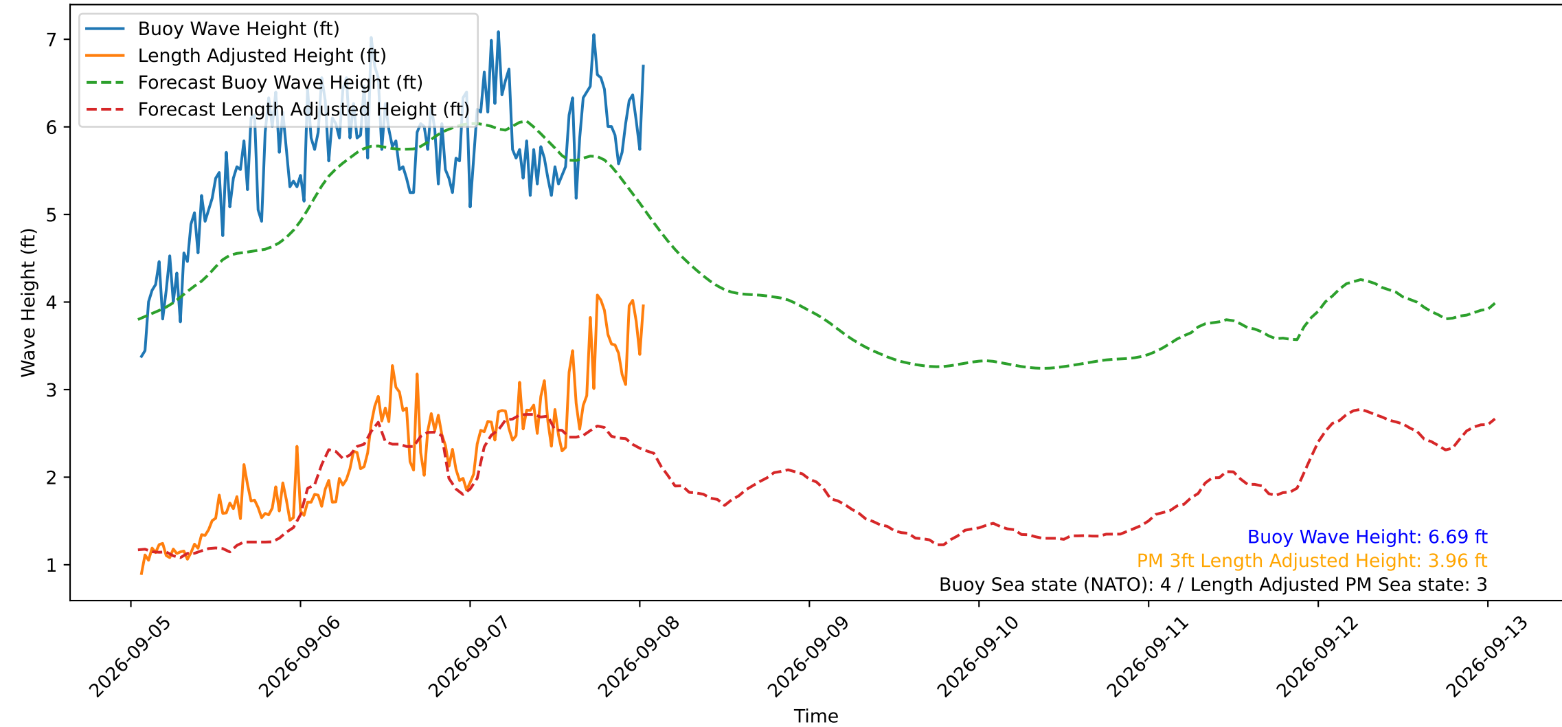
Wave Heights over Time for Oceanside Harbor at 2026-09-08 01:20:30
