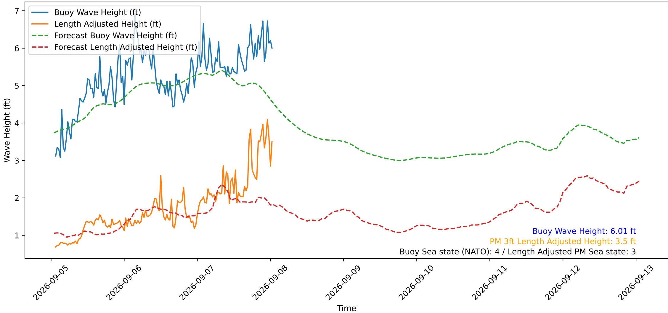
Wave Heights over Time for Red Beach at 2026-09-08 01:20:50
