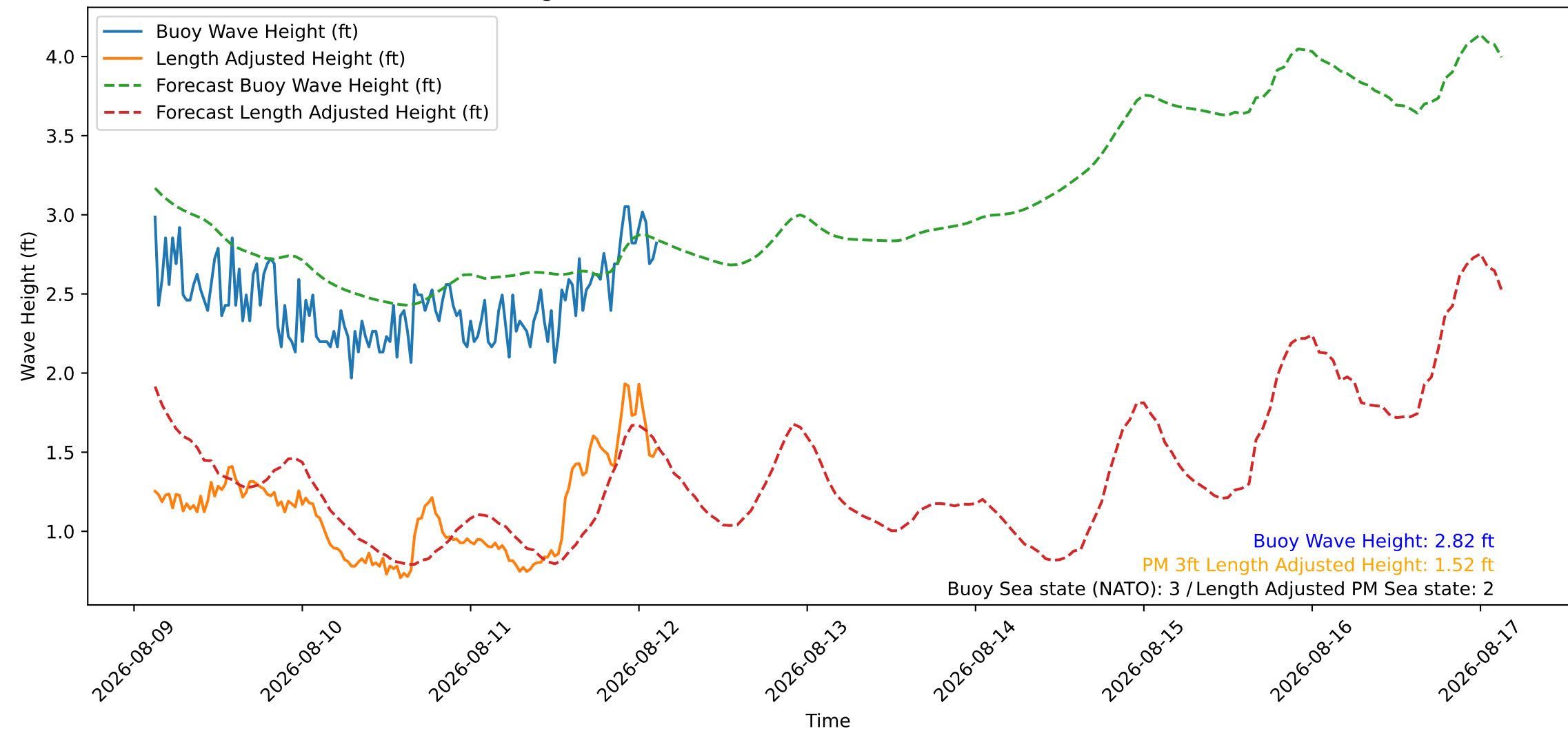
Wave Heights over Time for Oceanside Harbor at 2026-08-12 03:00:27
