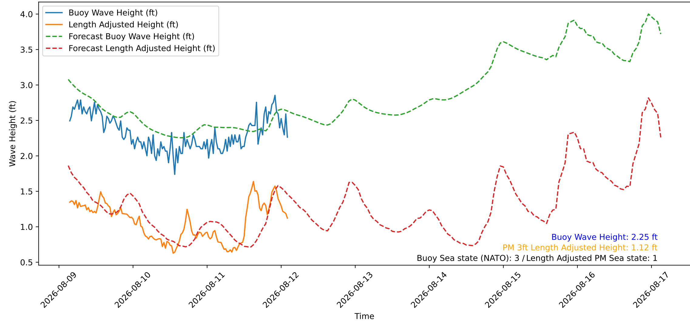
Wave Heights over Time for Red Beach at 2026-08-12 03:00:46
