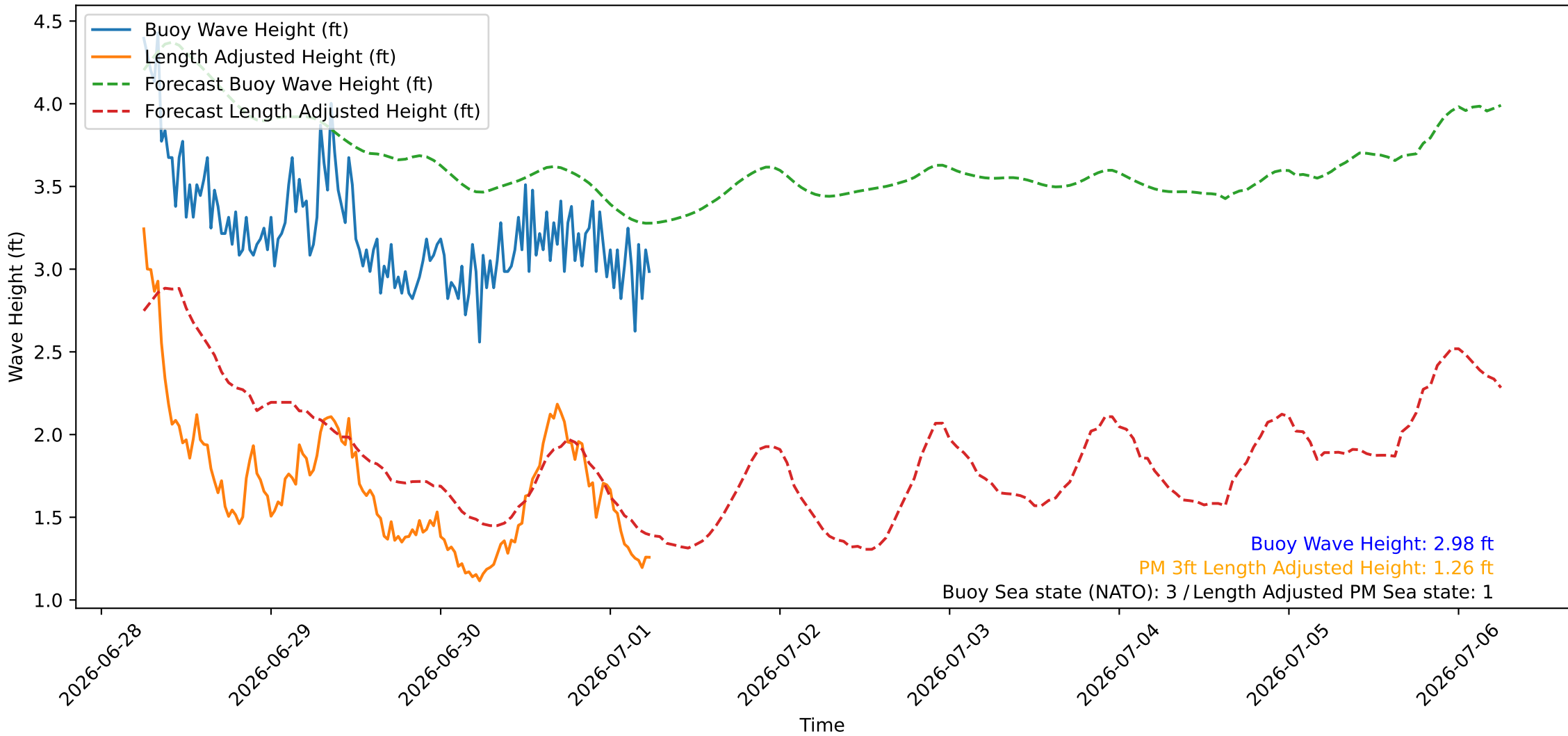
Wave Heights over Time for Oceanside Harbor at 2026-07-01 06:10:26
