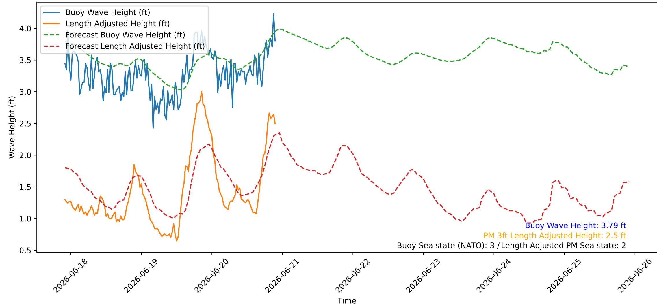
Wave Heights over Time for Green Beach at 2026-06-20 22:11:08
