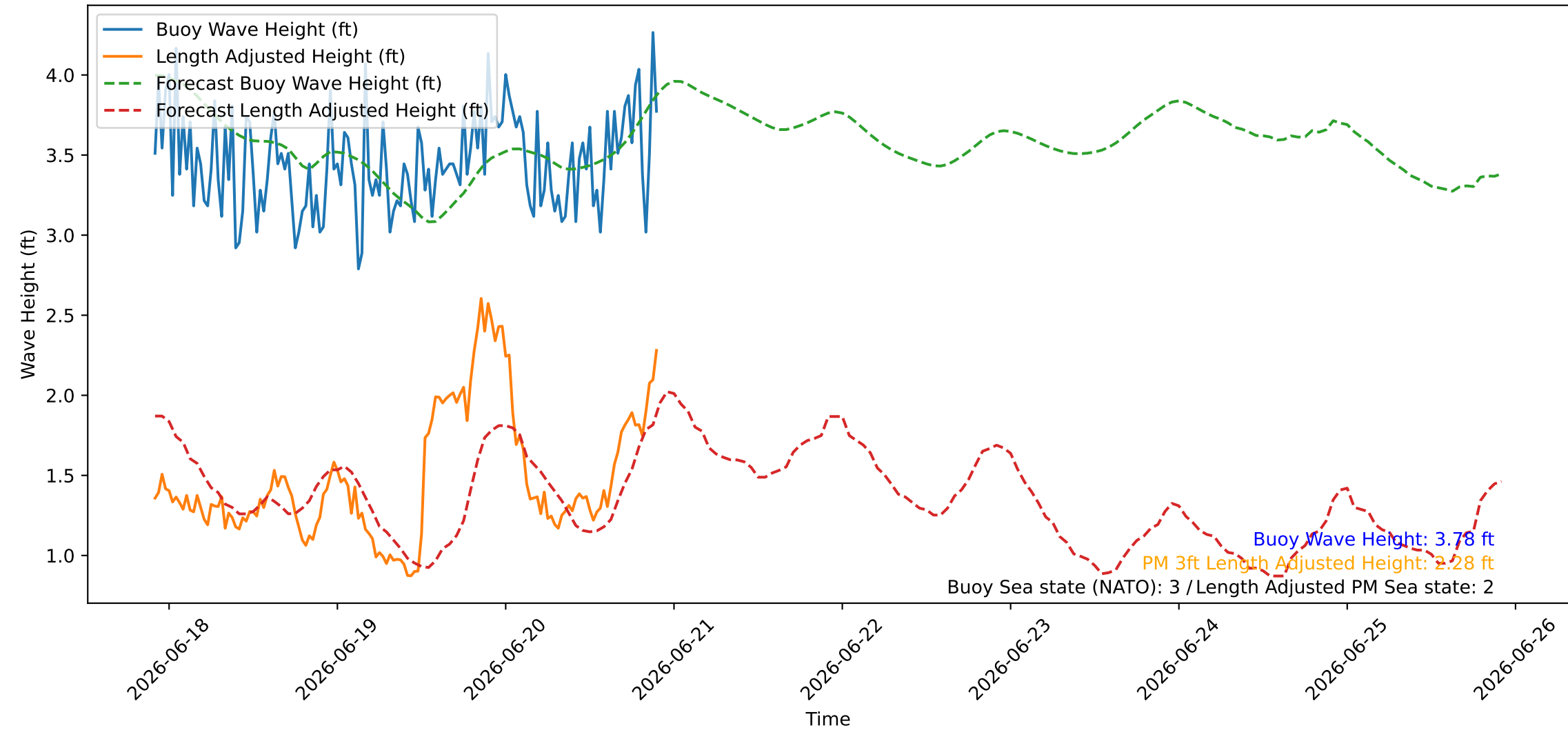
Wave Heights over Time for Oceanside Harbor at 2026-06-20 22:10:26
