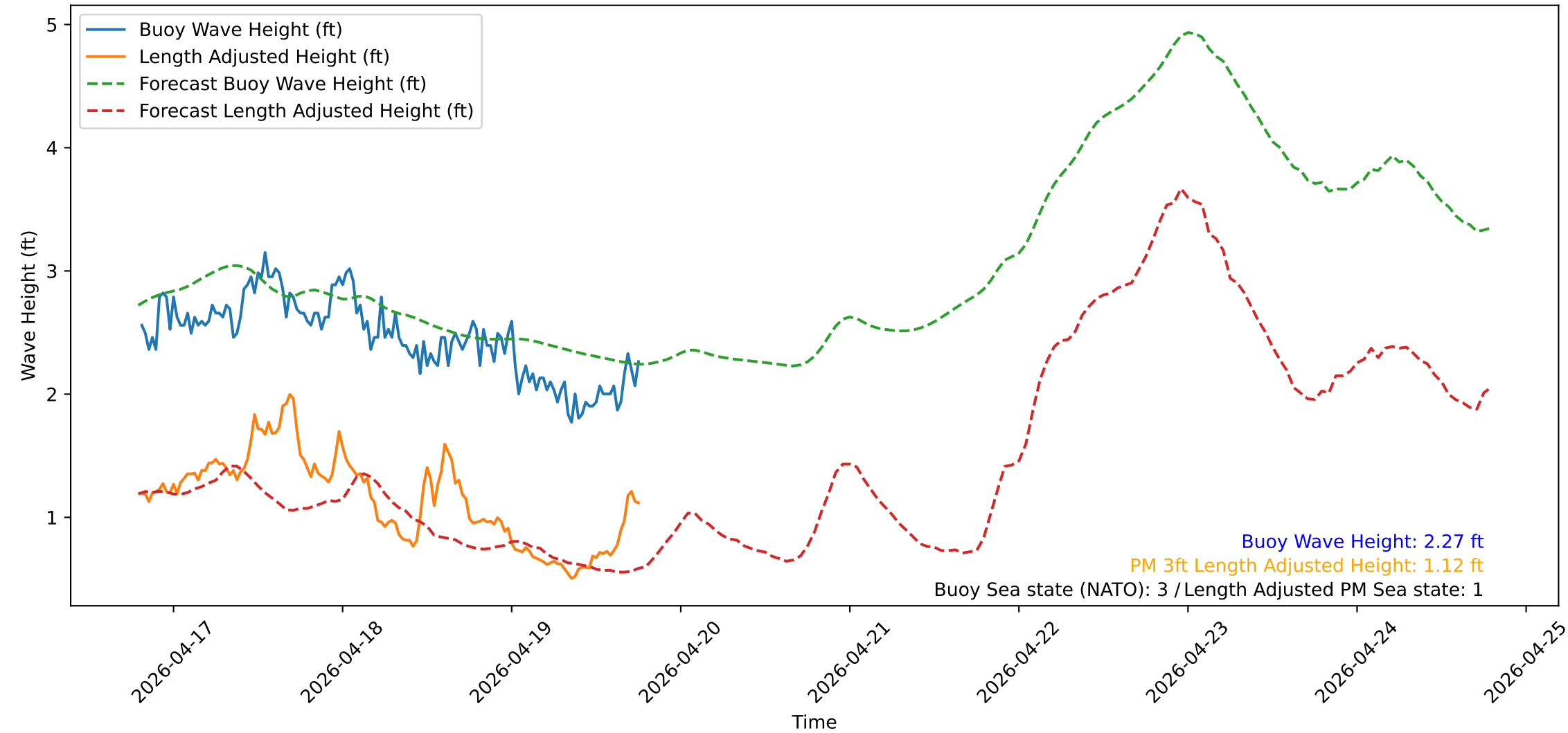
Wave Heights over Time for Red Beach at 2026-04-19 19:00:59
