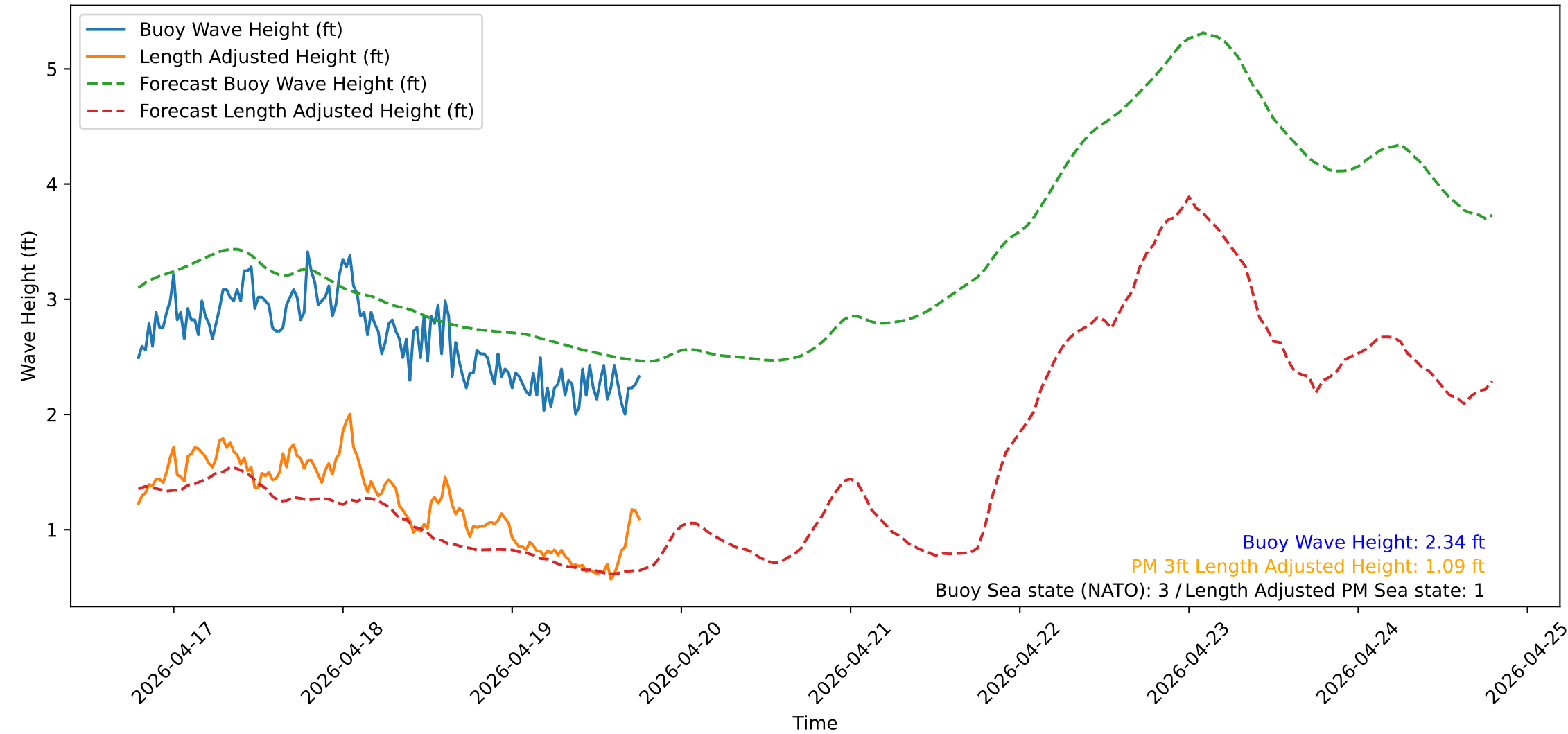
Wave Heights over Time for Oceanside Harbor at 2026-04-19 19:00:39
