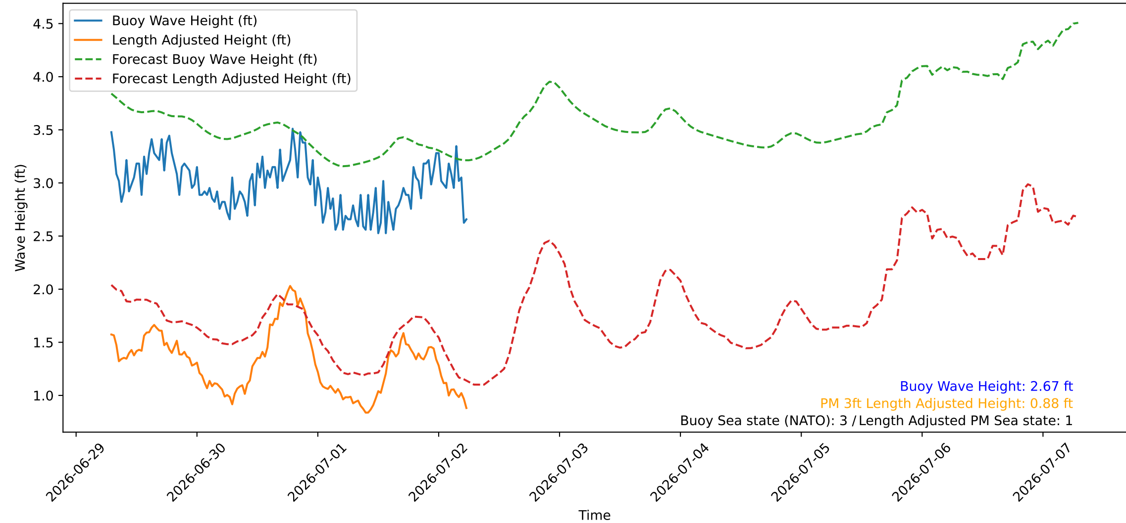
Wave Heights over Time for Green Beach at 2026-07-02 07:01:08
