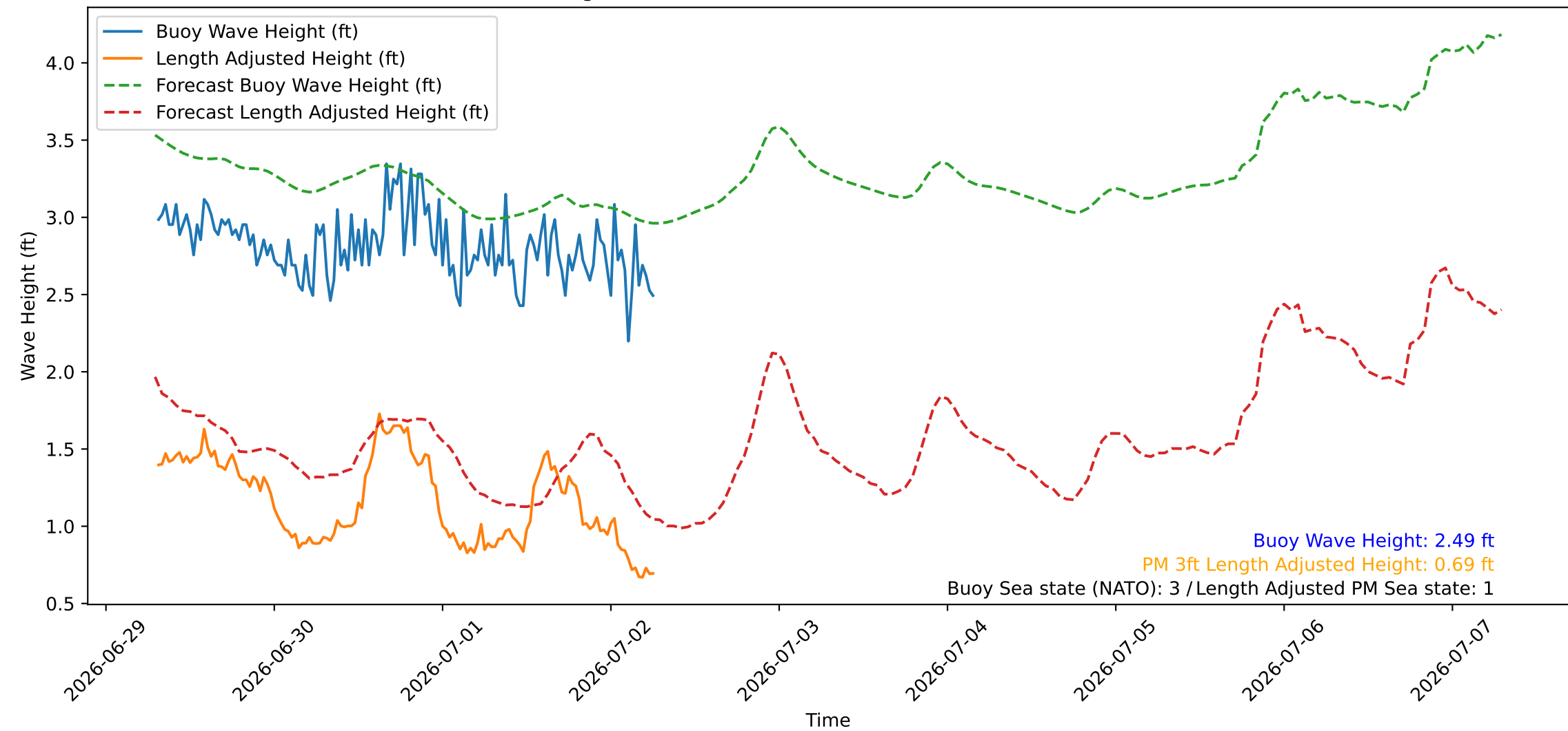
Wave Heights over Time for Red Beach at 2026-07-02 07:00:46
