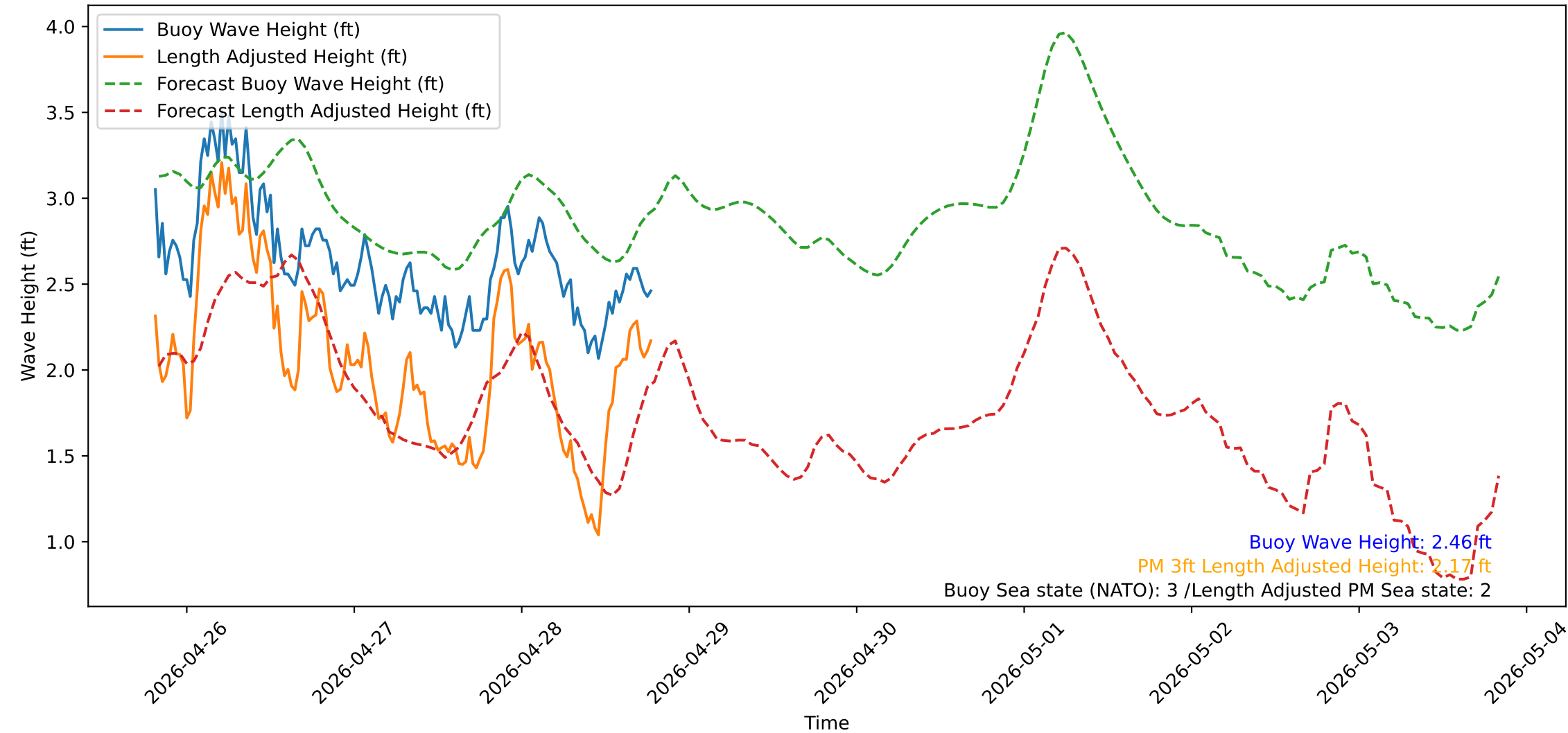
Wave Heights over Time for Green Beach at 2026-04-28 19:31:13
