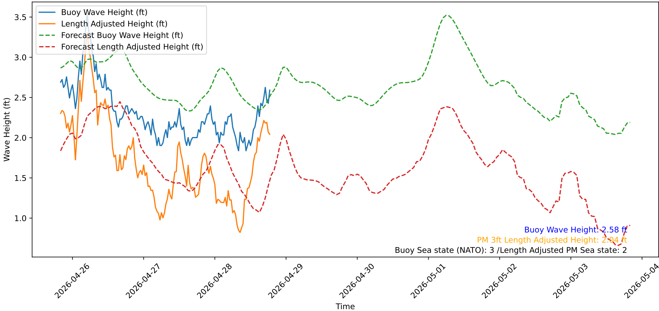
Wave Heights over Time for Red Beach at 2026-04-28 19:30:51
