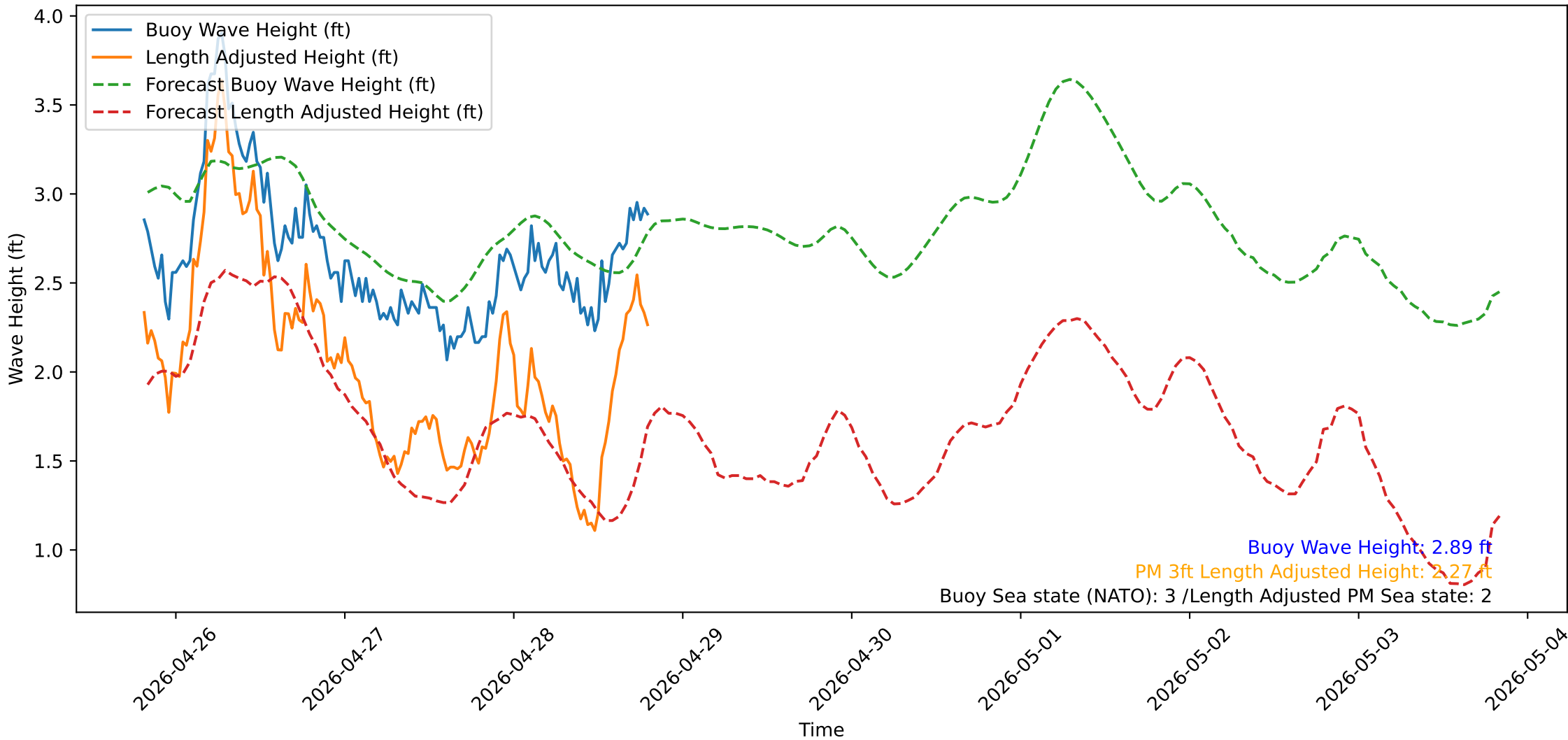
Wave Heights over Time for Oceanside Harbor at 2026-04-28 19:30:32
