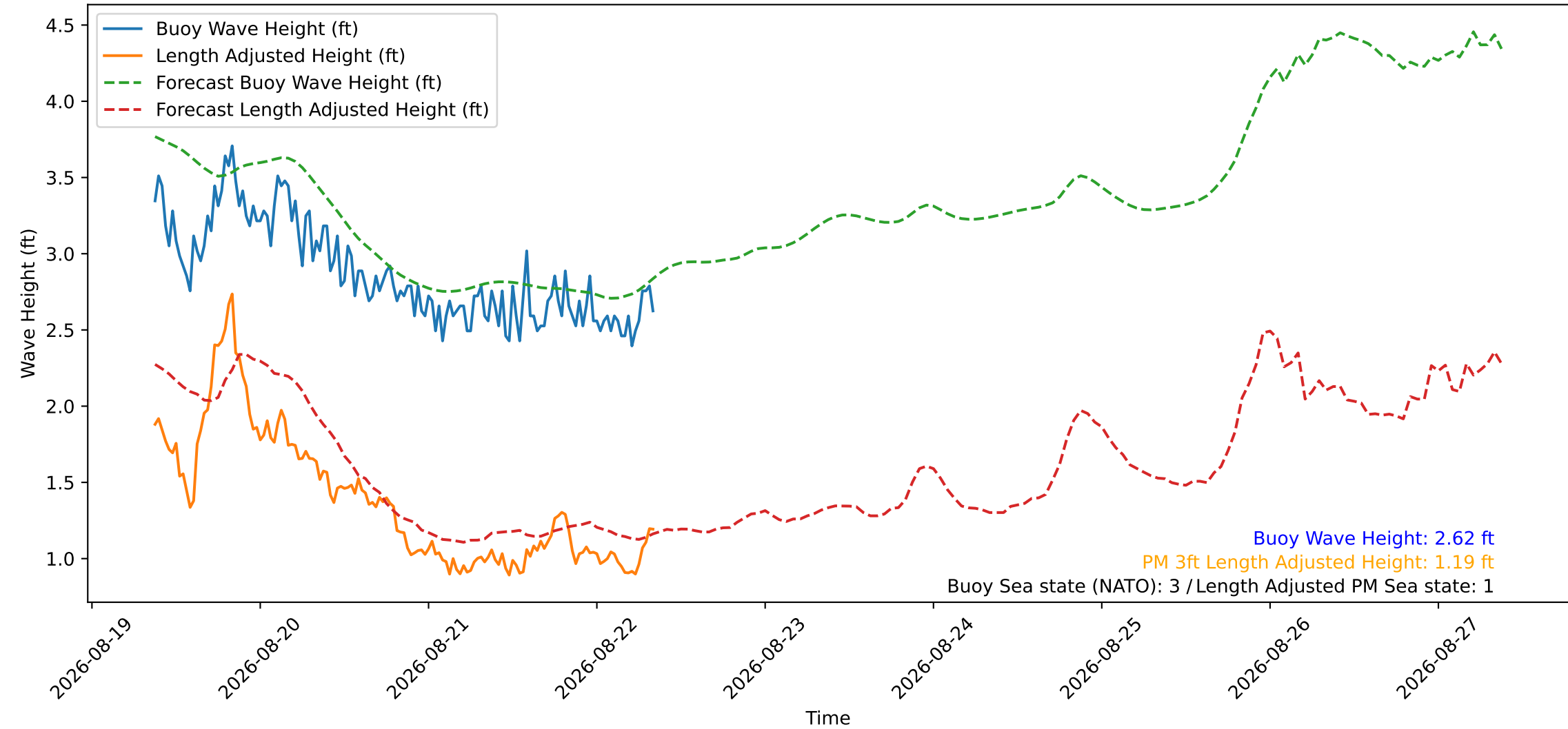
Wave Heights over Time for Green Beach at 2026-08-22 08:51:15
