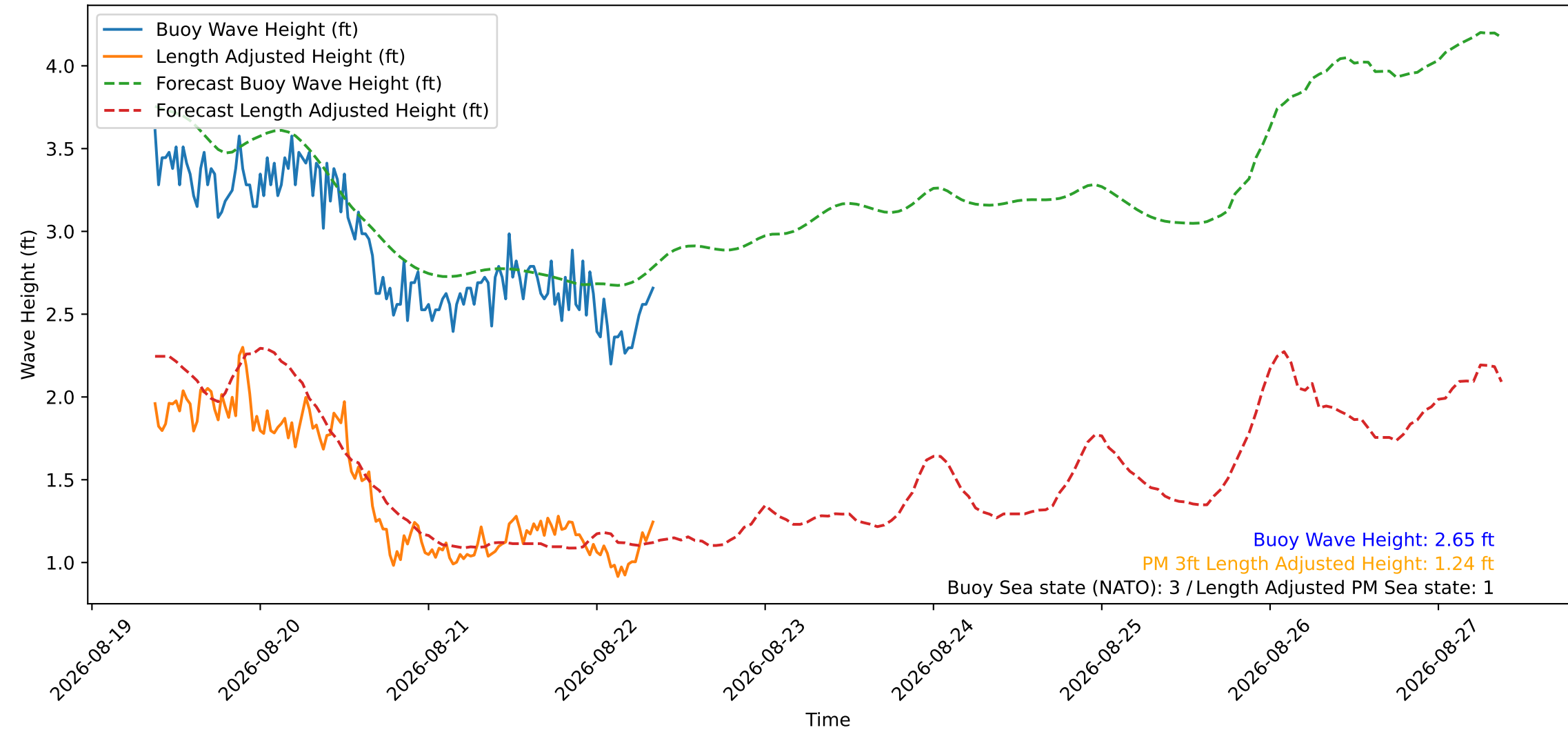
Wave Heights over Time for Oceanside Harbor at 2026-08-22 08:50:30
