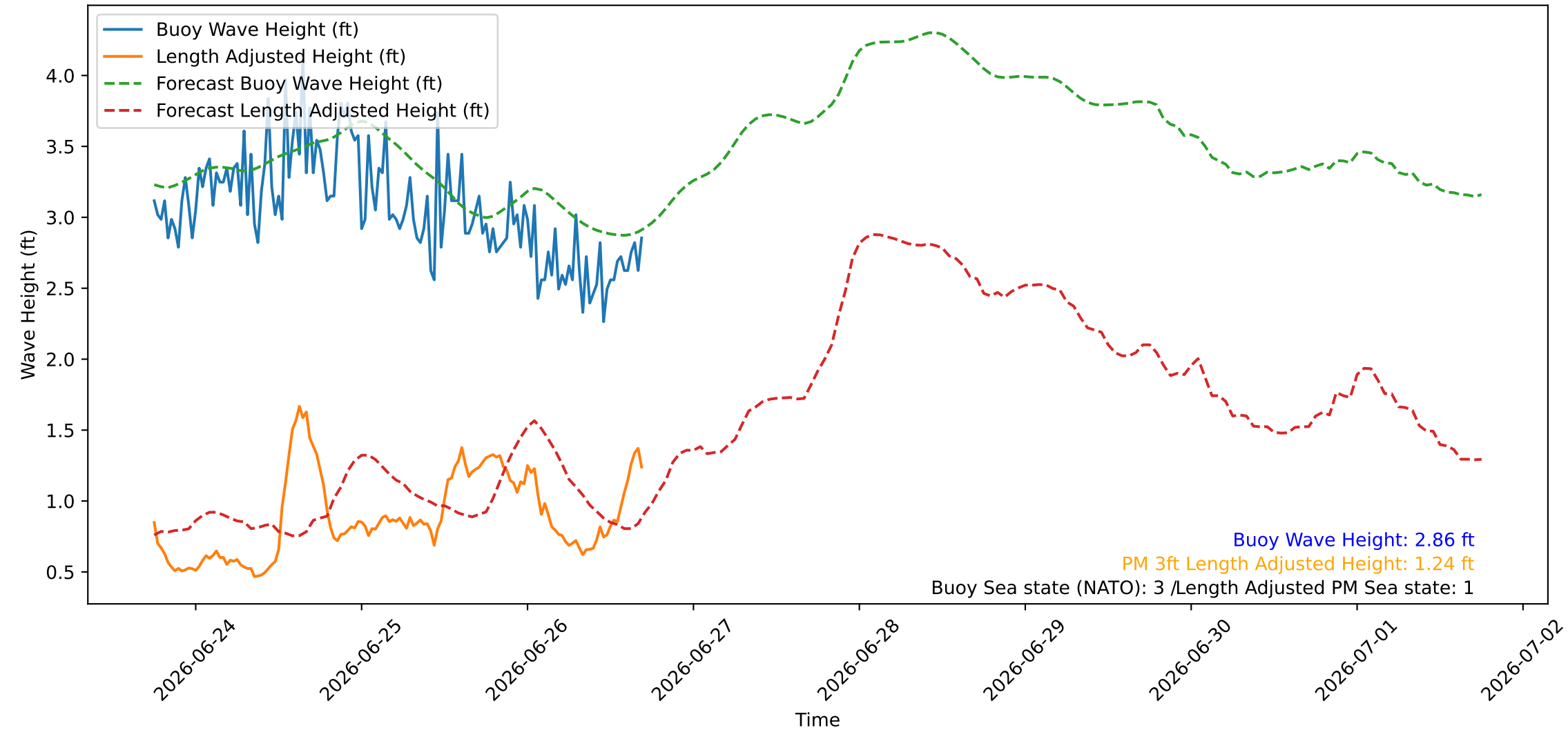
Wave Heights over Time for Red Beach at 2026-06-26 17:50:47
