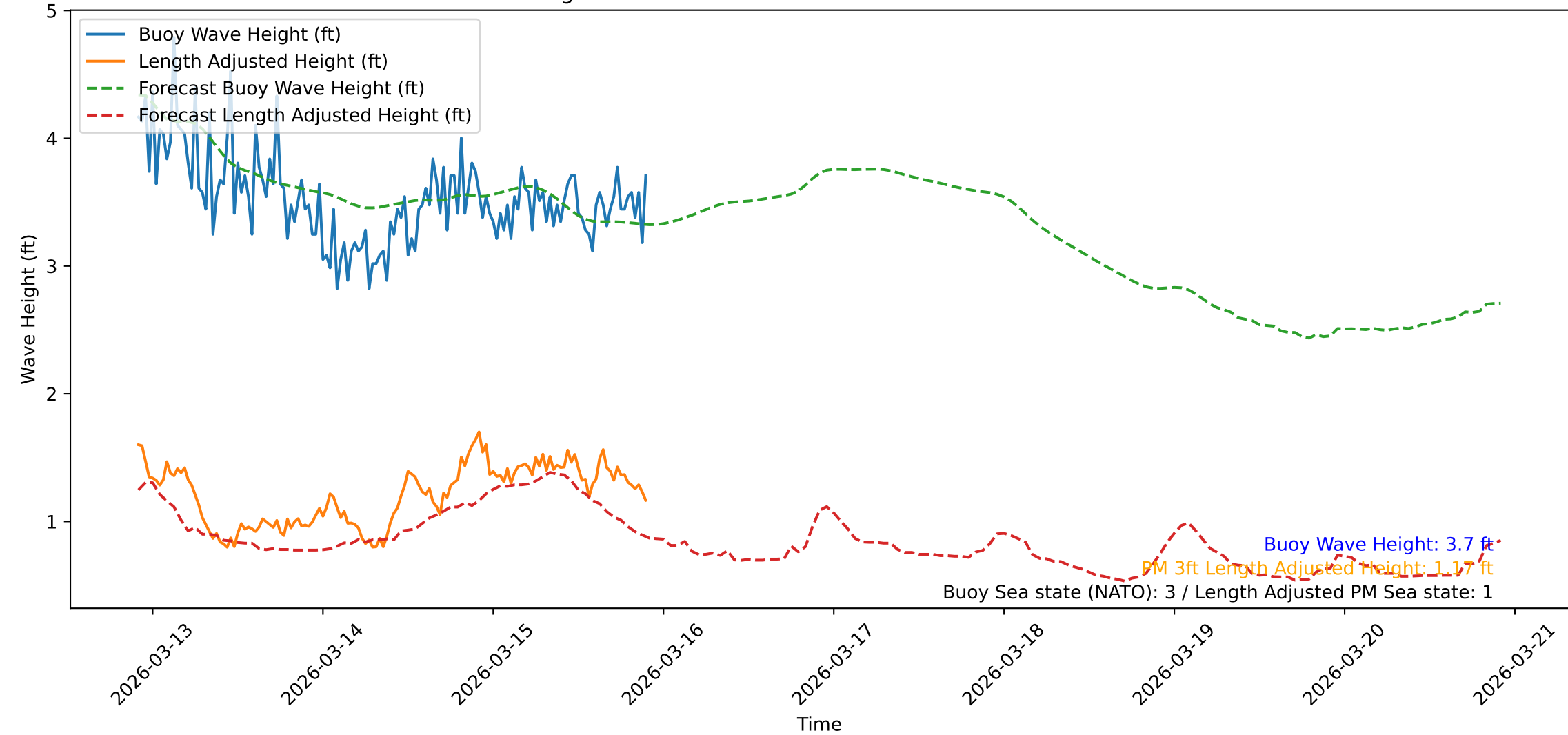
Wave Heights over Time for Green Beach at 2026-03-15 22:11:54
