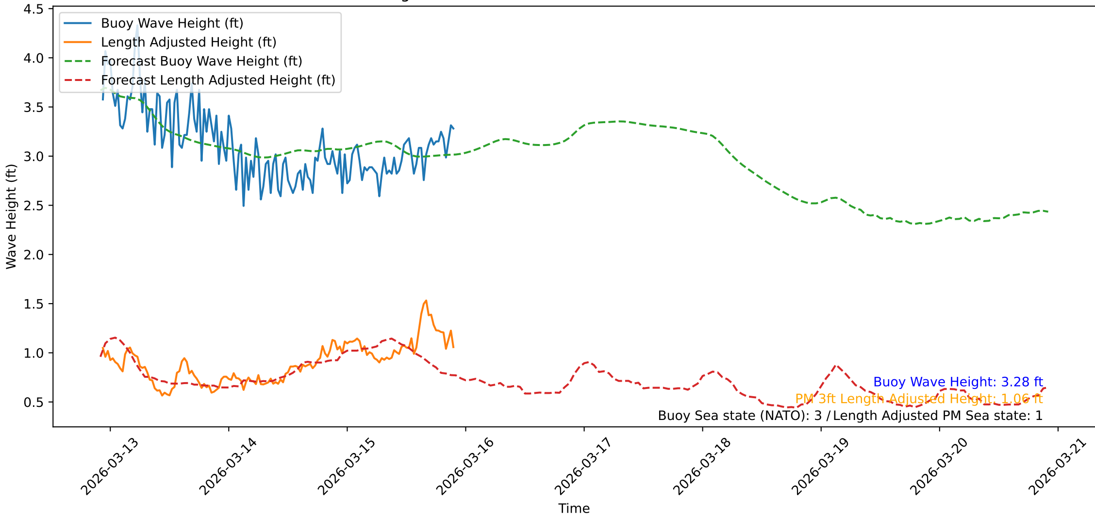
Wave Heights over Time for Red Beach at 2026-03-15 22:11:19
