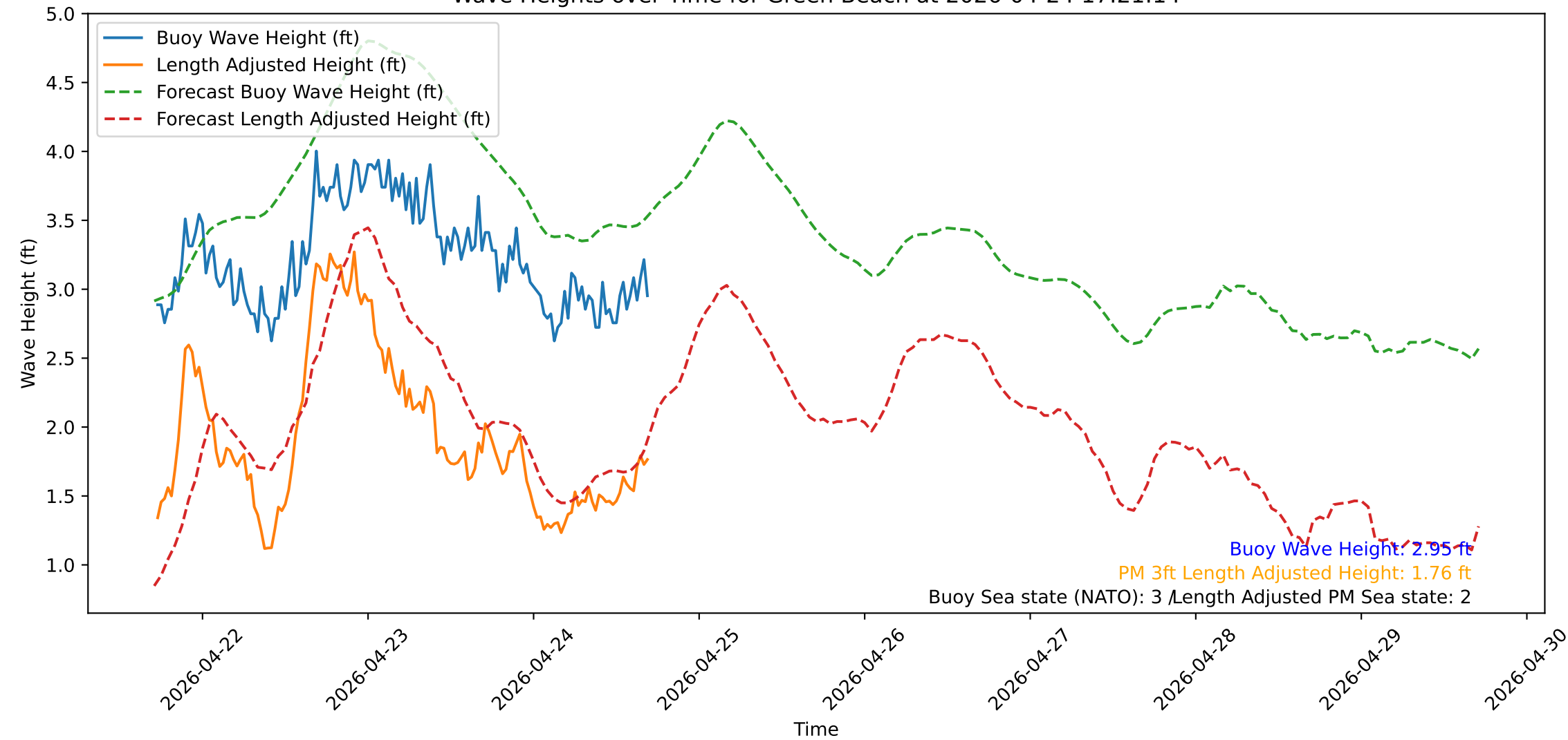
Wave Heights over Time for Green Beach at 2026-04-24 17:21:14
