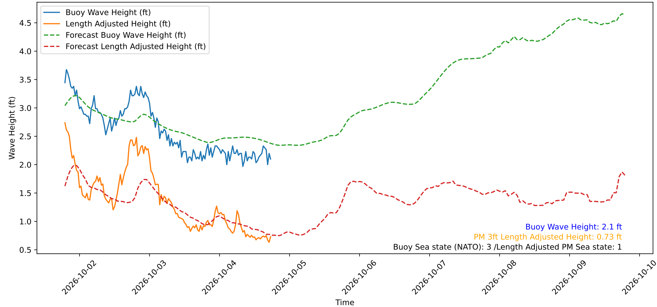
Wave Heights over Time for Green Beach at 2026-10-04 18:31:13
