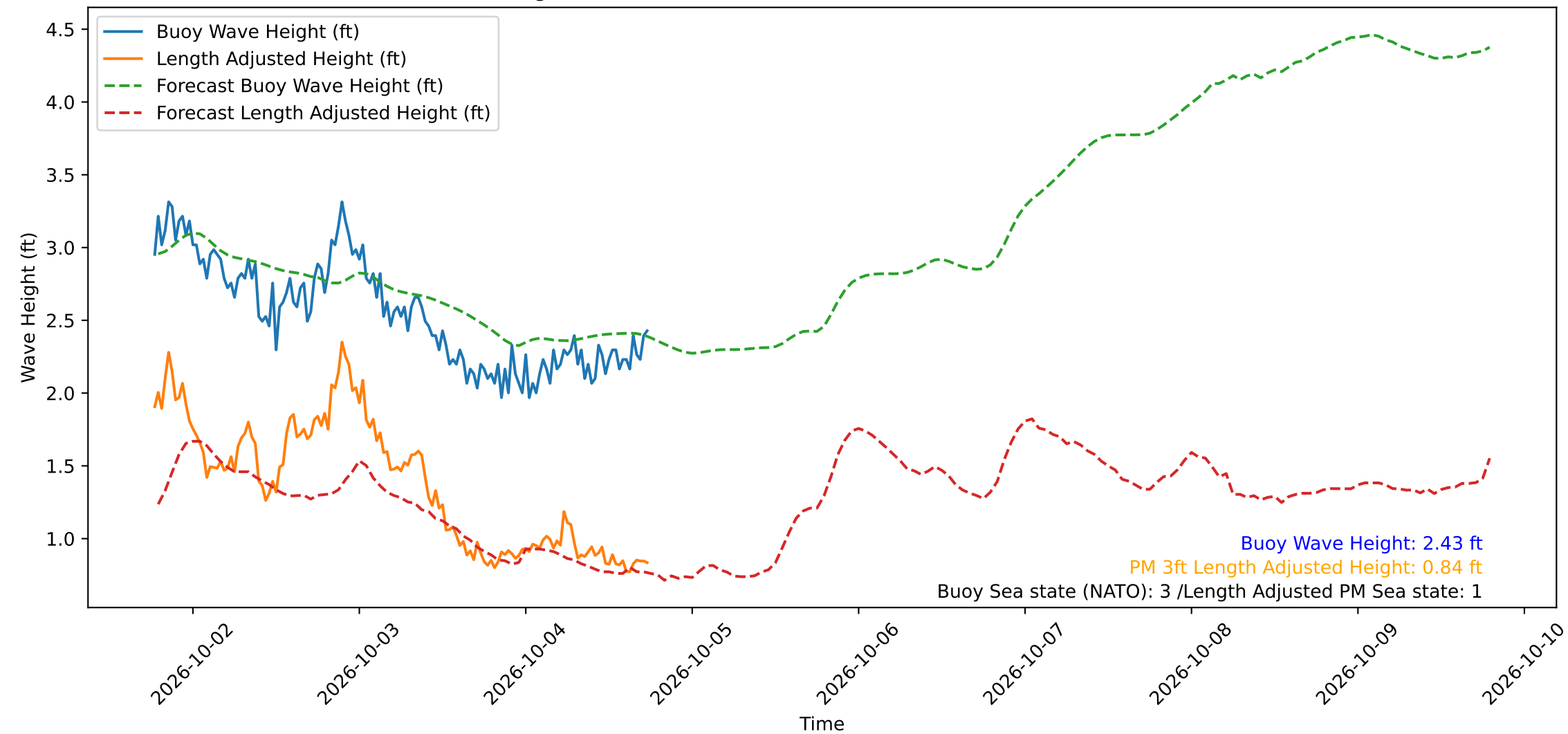
Wave Heights over Time for Oceanside Harbor at 2026-10-04 18:30:30
