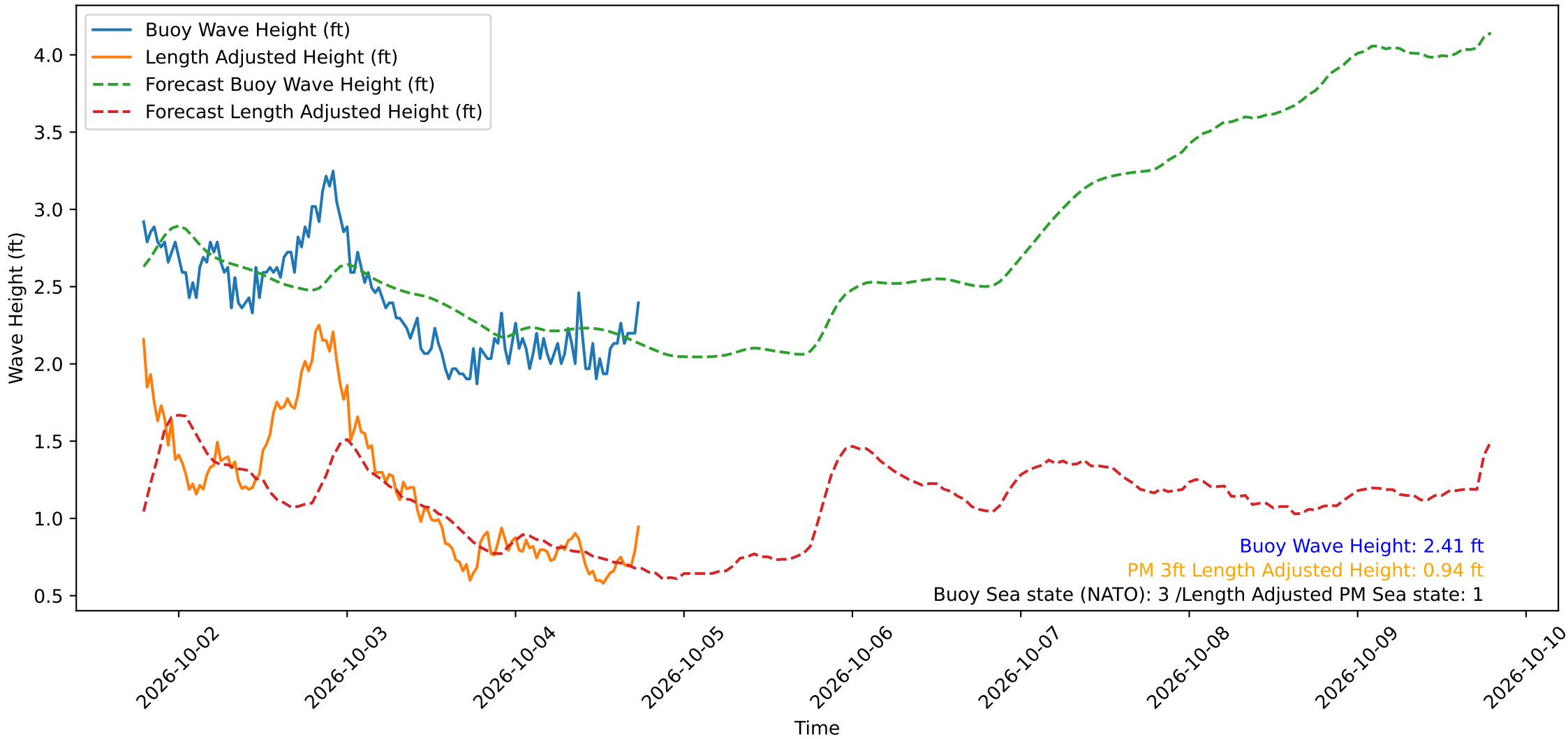
Wave Heights over Time for Red Beach at 2026-10-04 18:30:50
