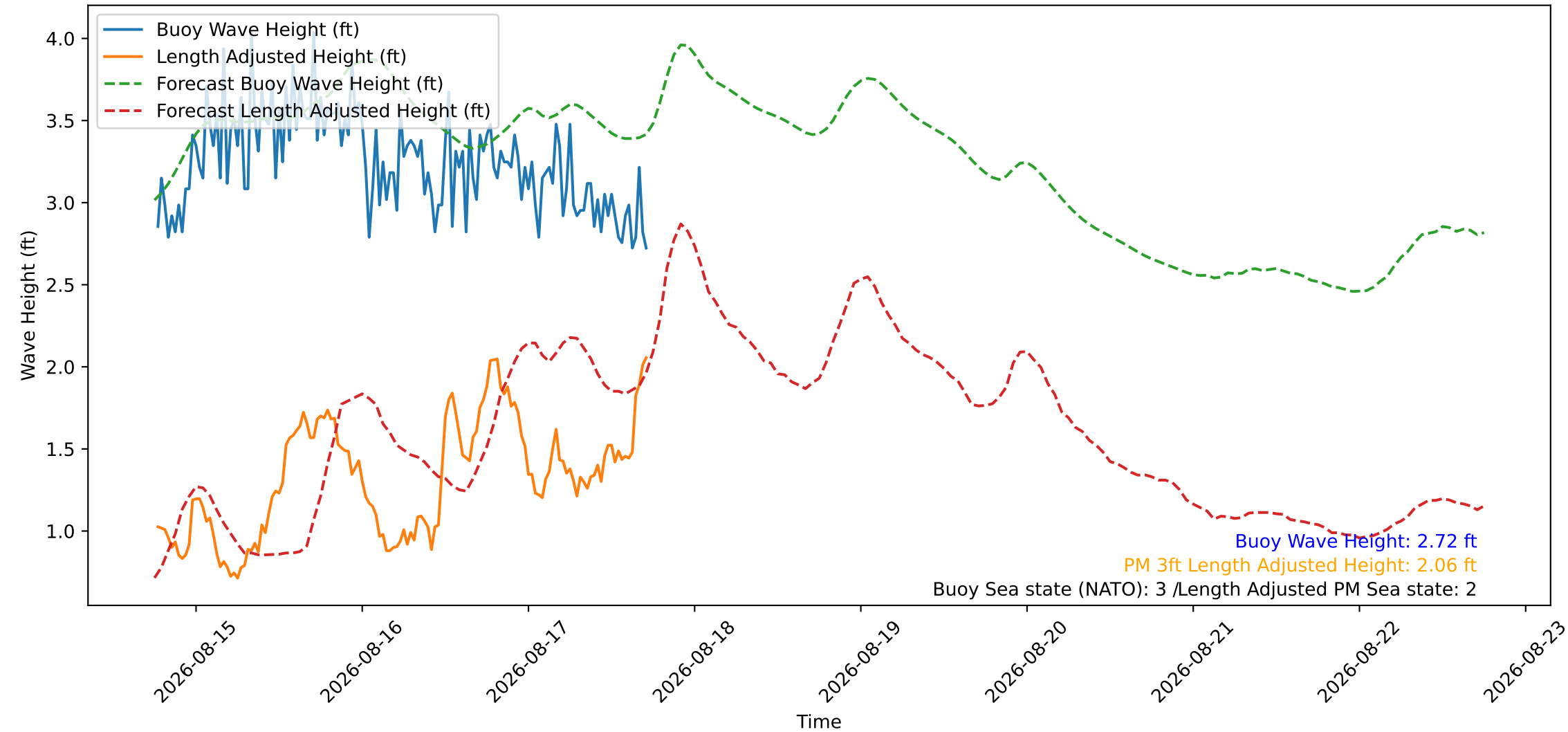
Wave Heights over Time for Red Beach at 2026-08-17 18:00:46
