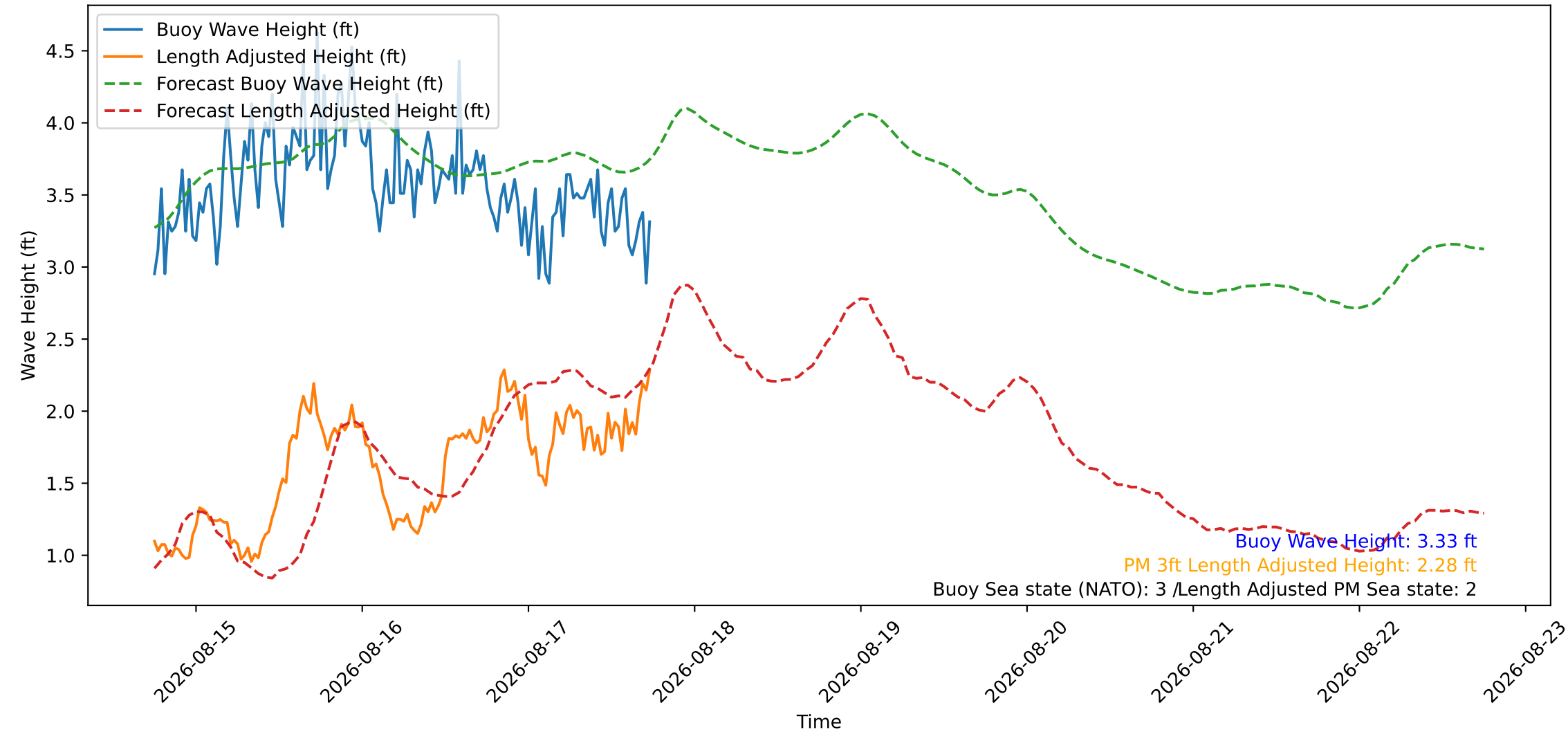
Wave Heights over Time for Oceanside Harbor at 2026-08-17 18:00:26
