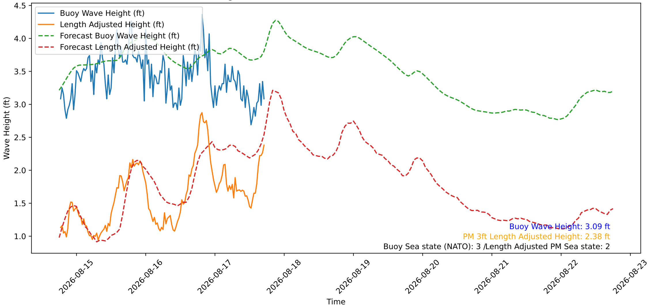
Wave Heights over Time for Green Beach at 2026-08-17 18:01:09
