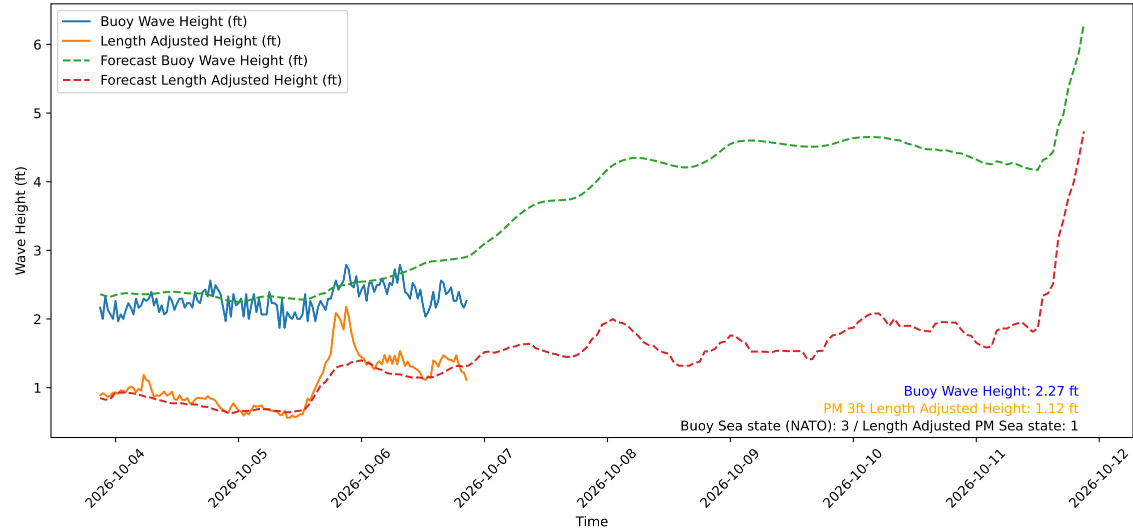
Wave Heights over Time for Oceanside Harbor at 2026-10-06 21:10:30
