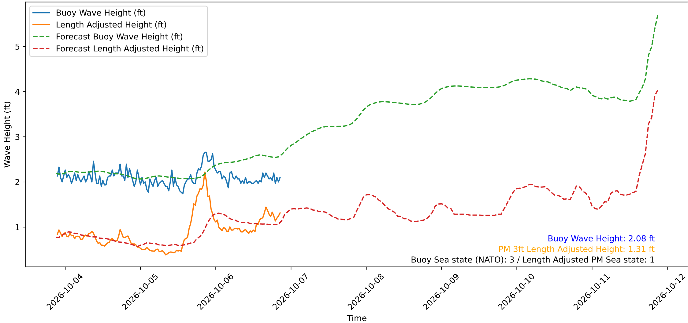
Wave Heights over Time for Red Beach at 2026-10-06 21:10:50
