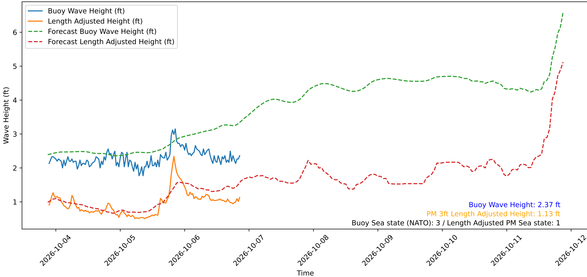
Wave Heights over Time for Green Beach at 2026-10-06 21:11:13
