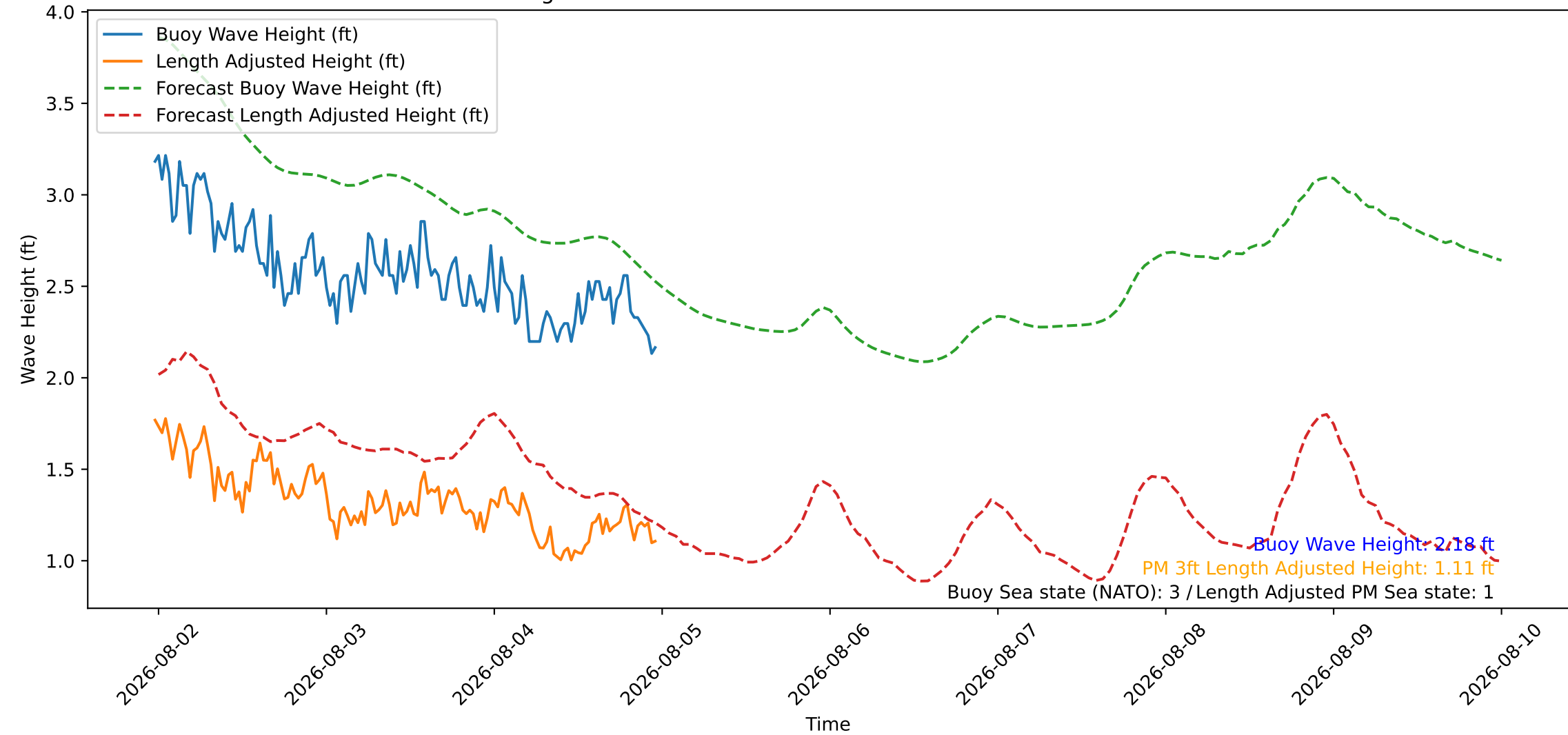
Wave Heights over Time for Oceanside Harbor at 2026-08-04 23:40:26
