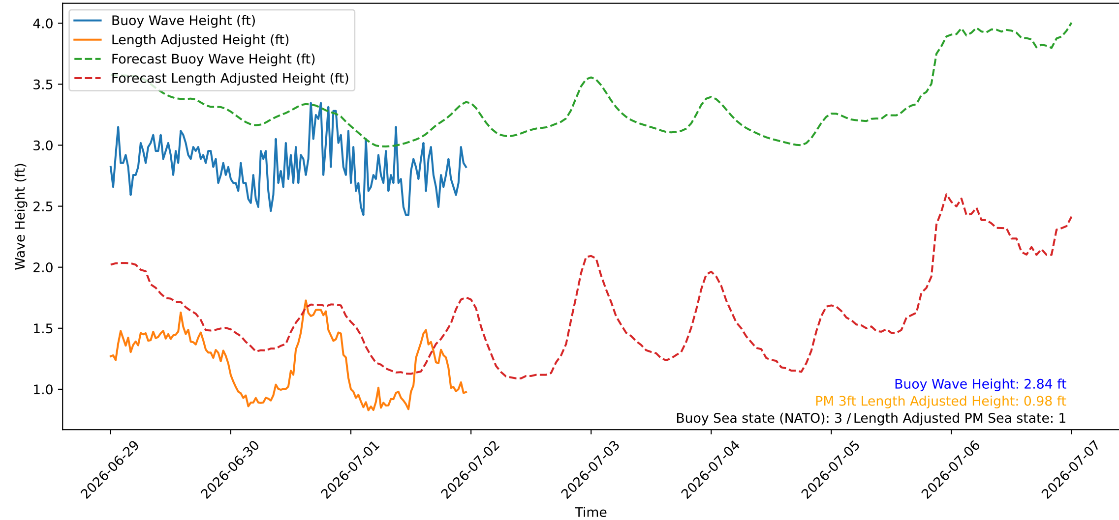
Wave Heights over Time for Red Beach at 2026-07-01 23:50:47
