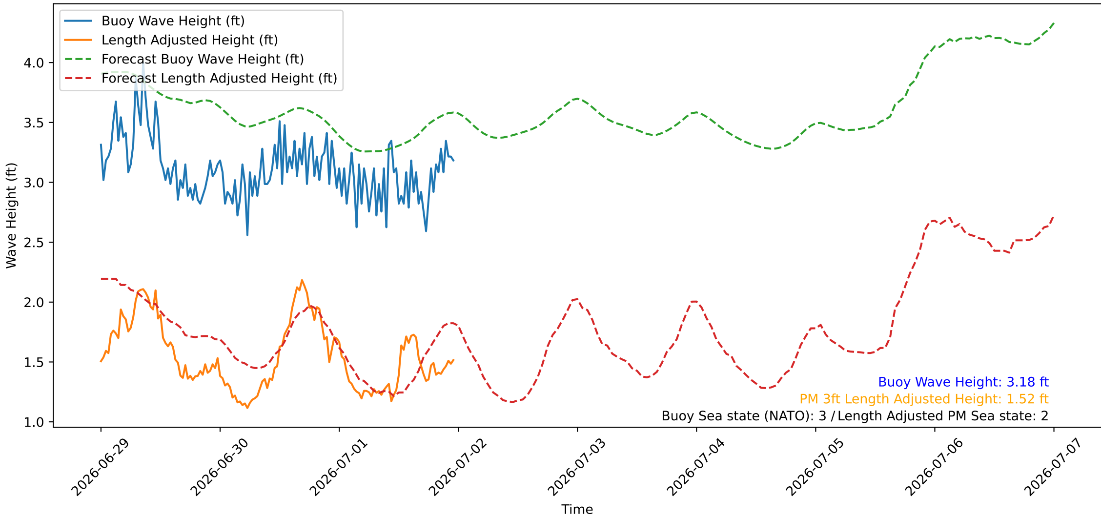
Wave Heights over Time for Oceanside Harbor at 2026-07-01 23:50:26
