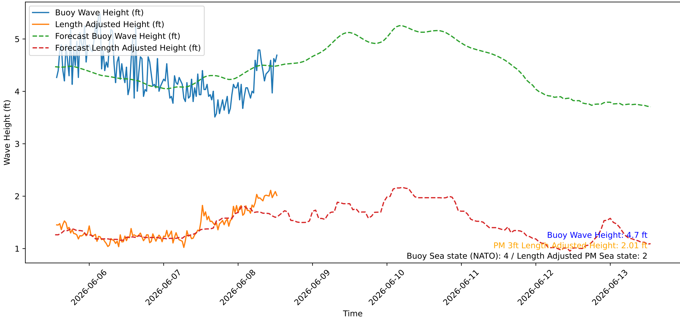
Wave Heights over Time for Oceanside Harbor at 2026-06-08 13:20:25
