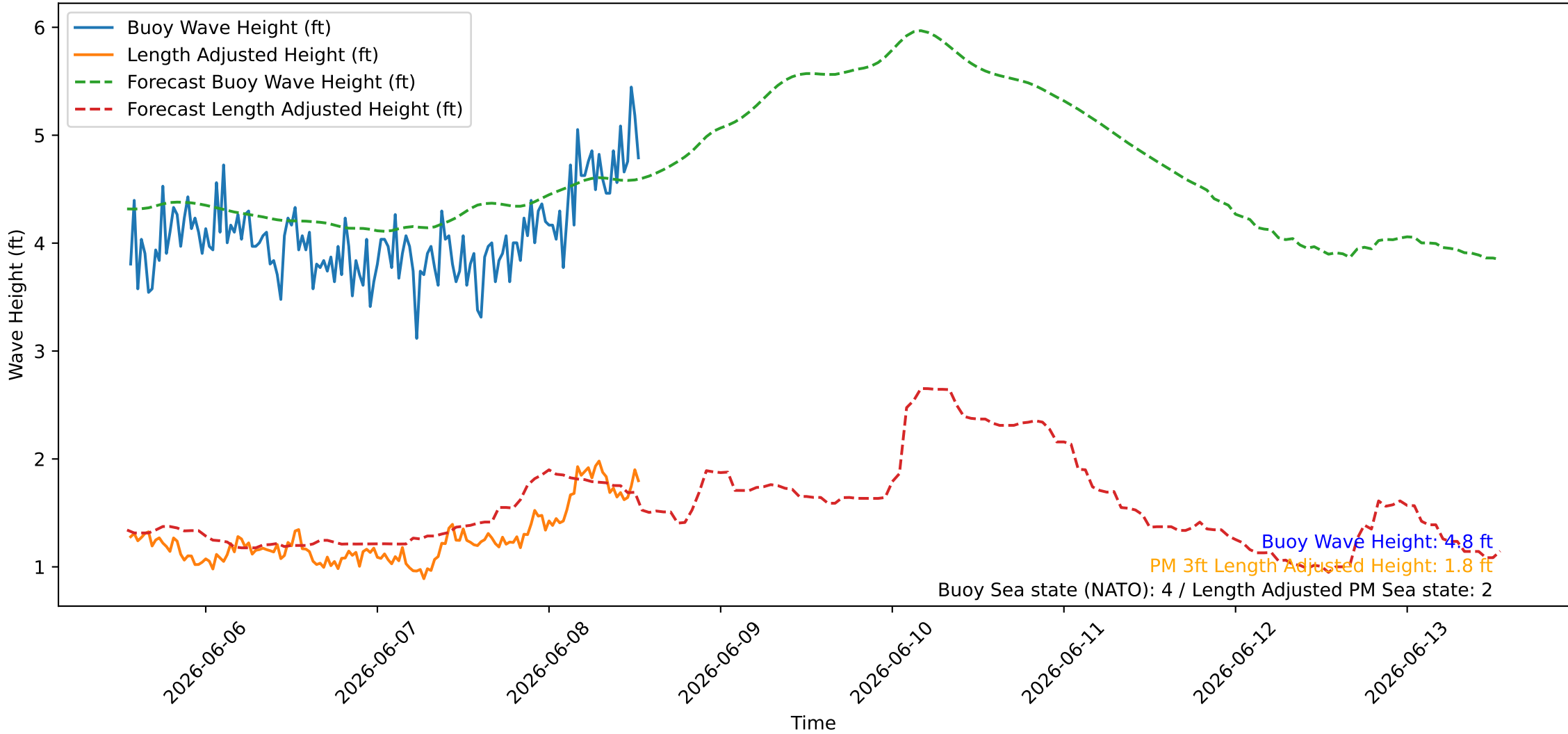
Wave Heights over Time for Green Beach at 2026-06-08 13:21:09
