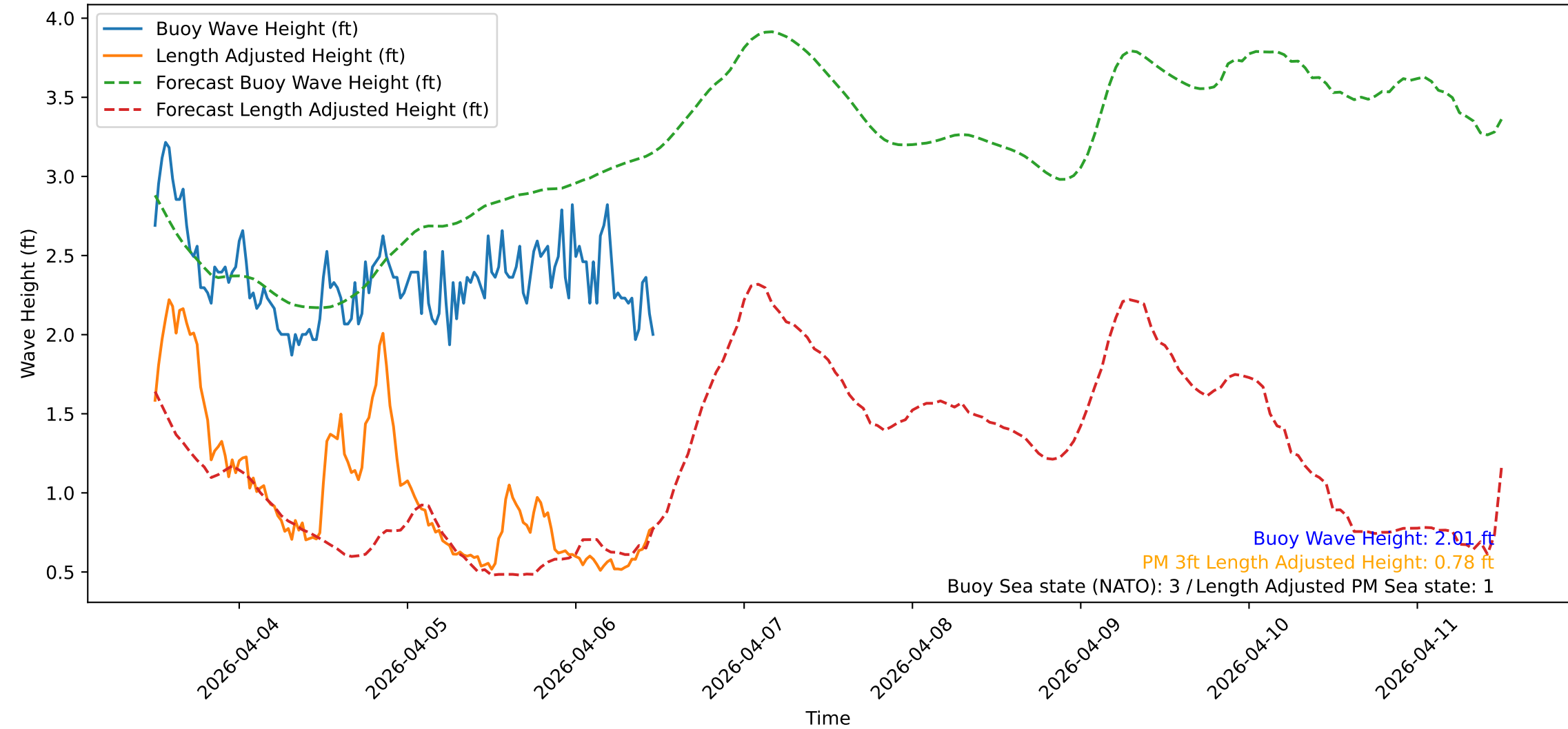
Wave Heights over Time for Red Beach at 2026-04-06 11:50:48
