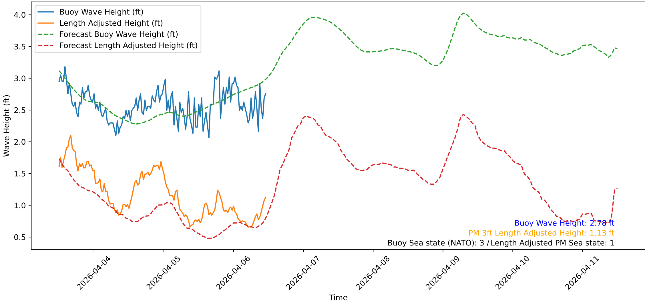
Wave Heights over Time for Oceanside Harbor at 2026-04-06 11:50:32
