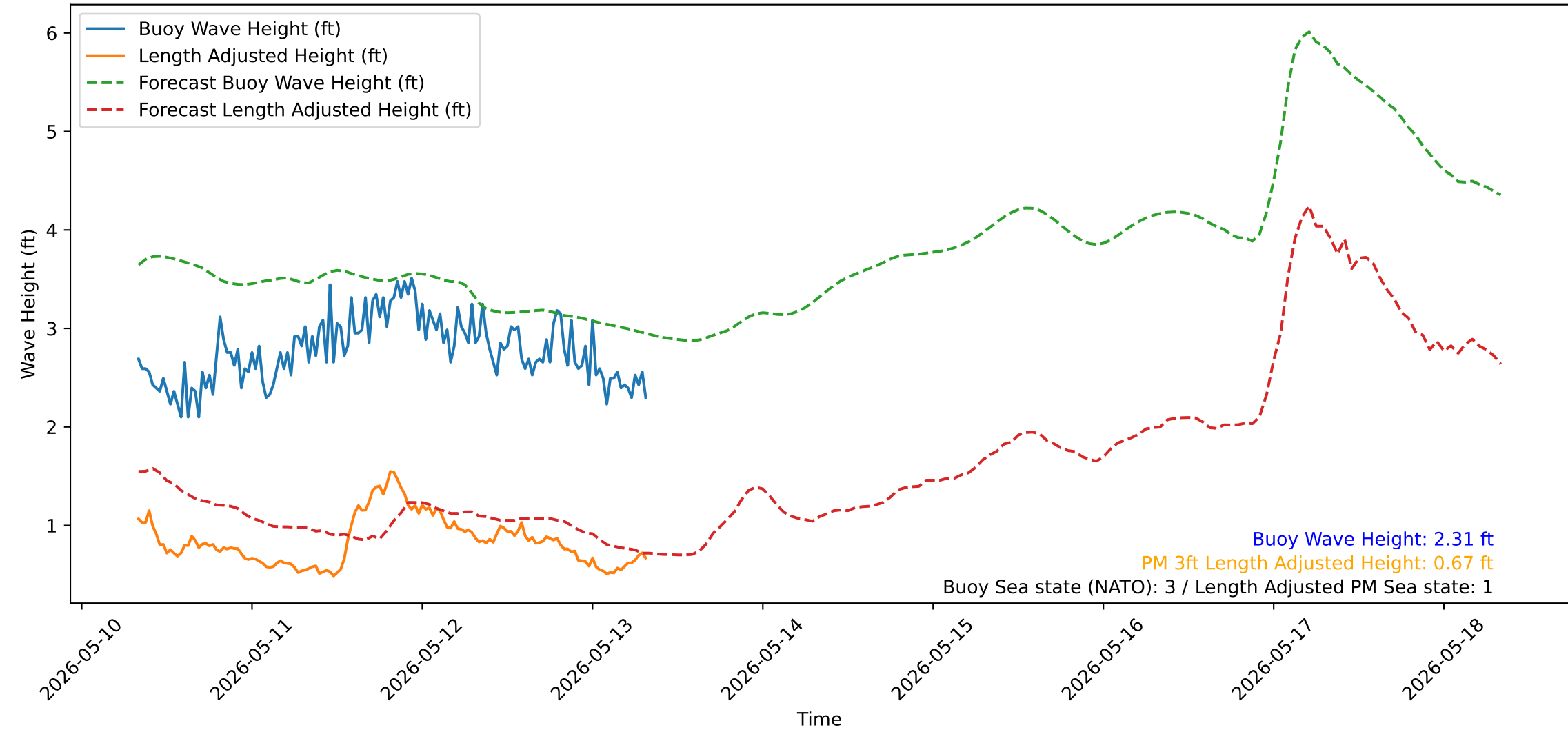
Wave Heights over Time for Green Beach at 2026-05-13 08:11:14
