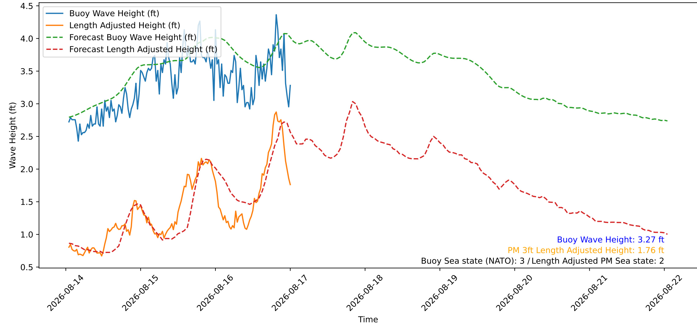
Wave Heights over Time for Green Beach at 2026-08-17 00:41:09
