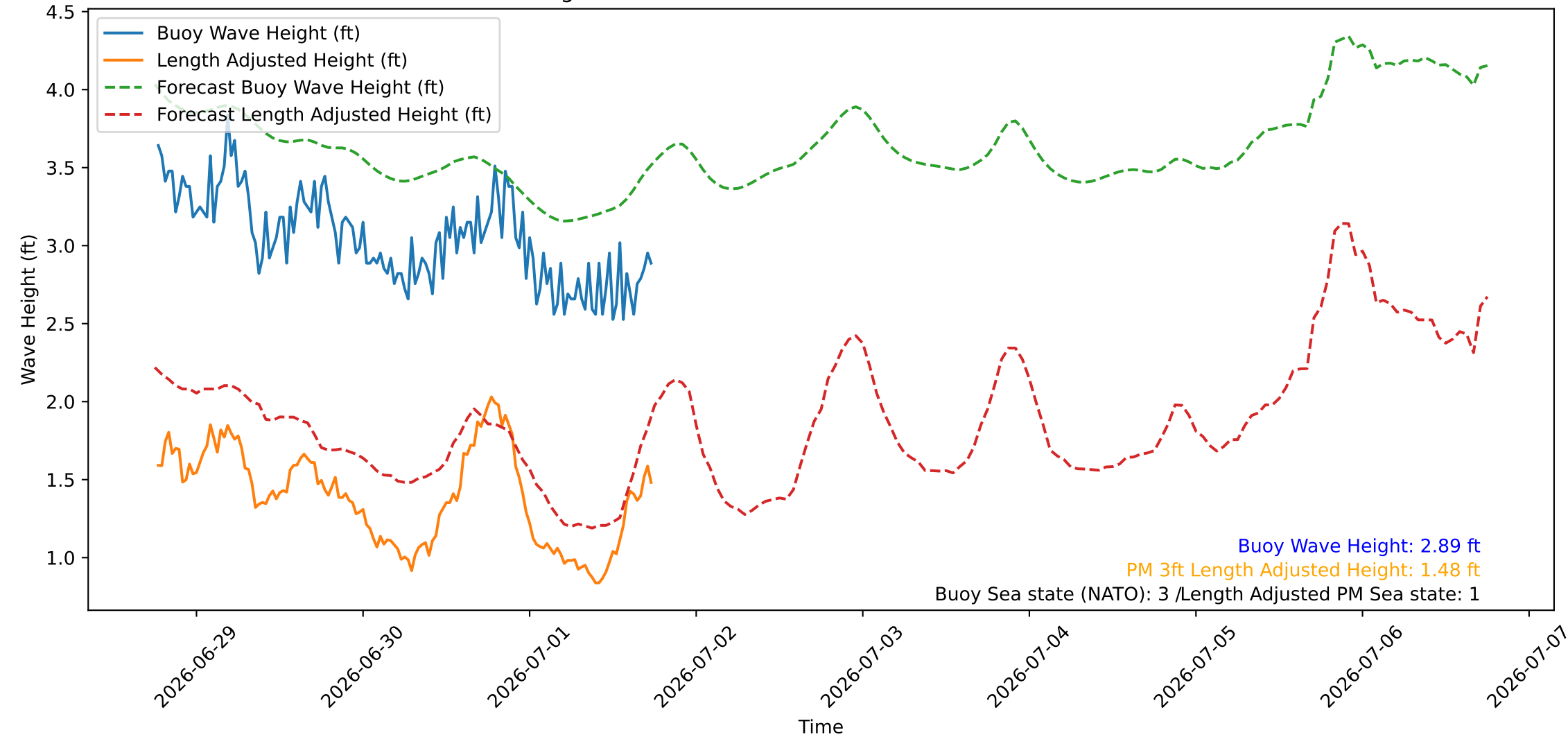
Wave Heights over Time for Green Beach at 2026-07-01 18:21:09
