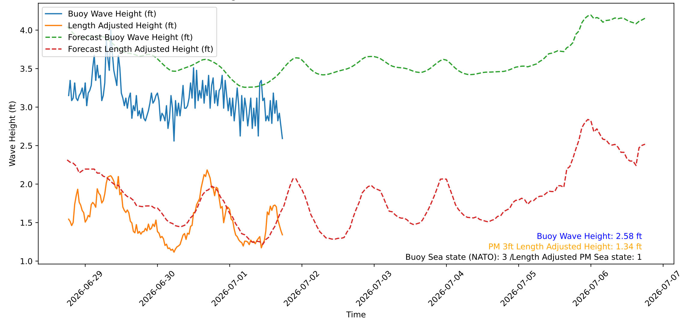
Wave Heights over Time for Oceanside Harbor at 2026-07-01 18:20:26
