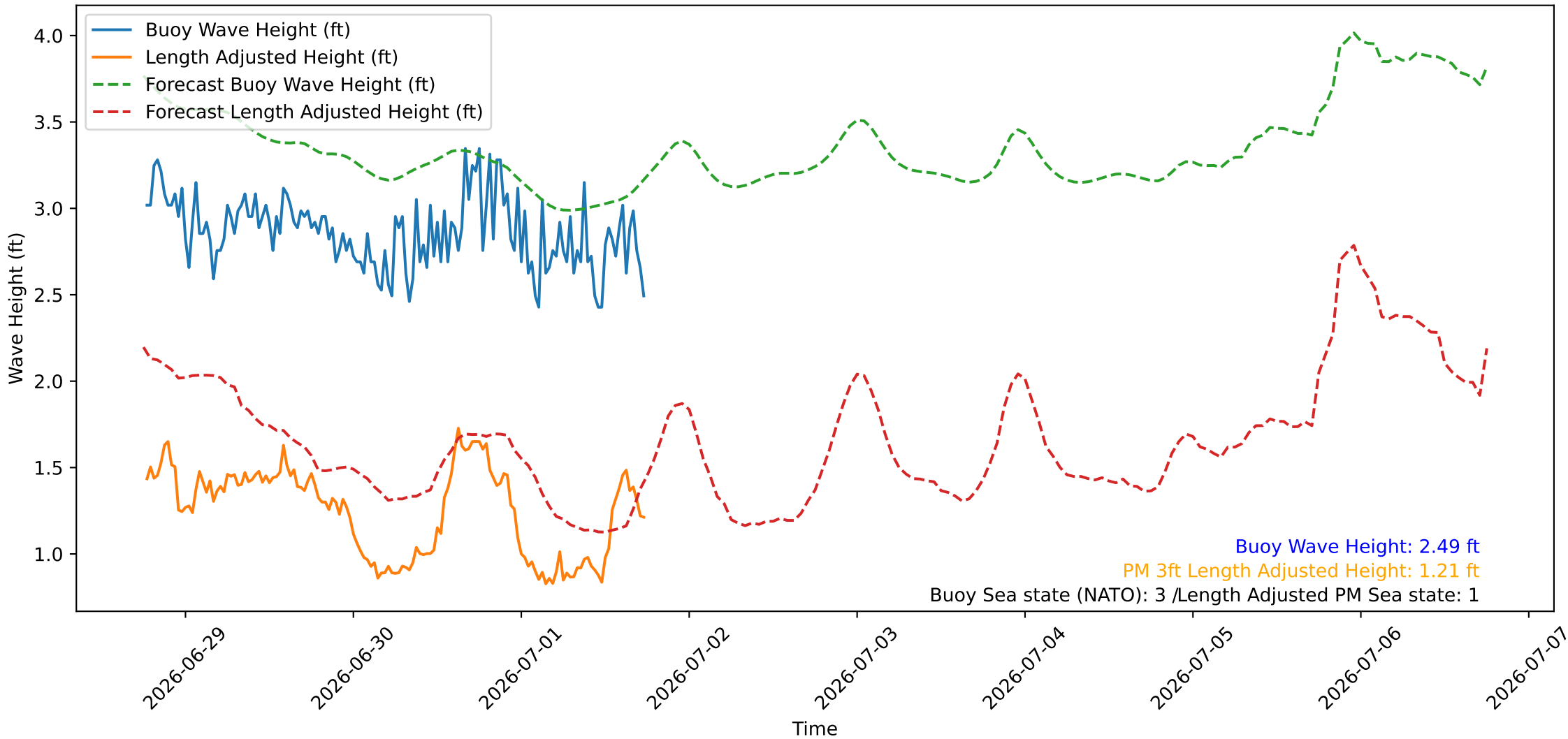
Wave Heights over Time for Red Beach at 2026-07-01 18:20:46
