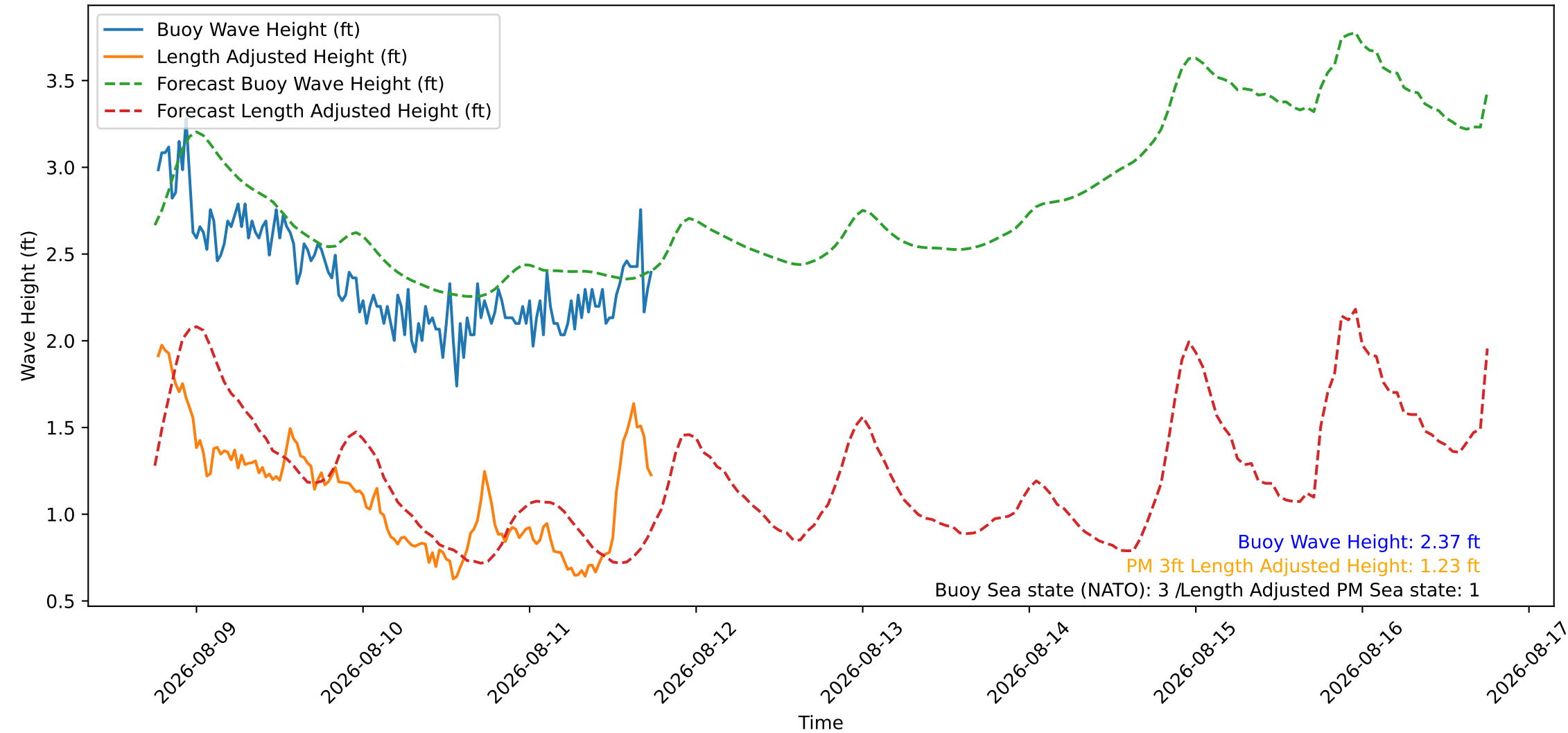
Wave Heights over Time for Red Beach at 2026-08-11 18:10:45
