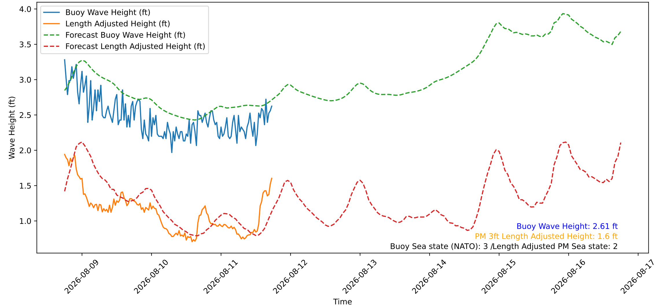
Wave Heights over Time for Oceanside Harbor at 2026-08-11 18:10:26
