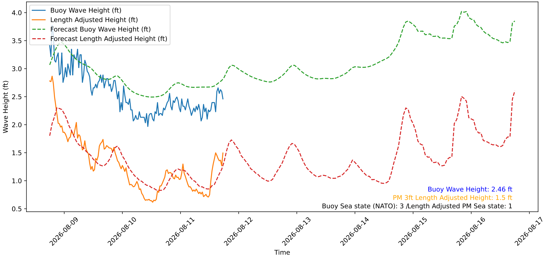
Wave Heights over Time for Green Beach at 2026-08-11 18:11:08
