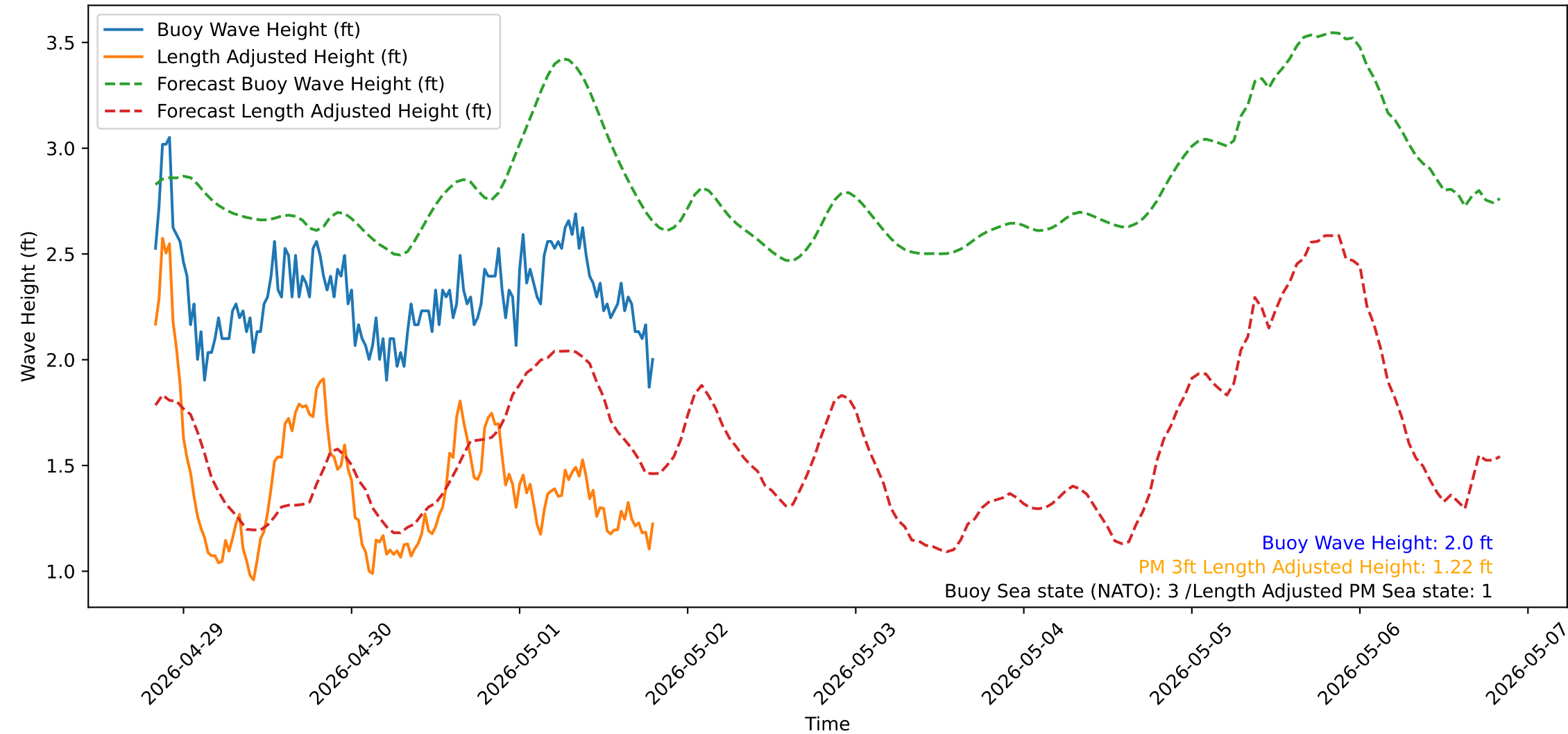
Wave Heights over Time for Oceanside Harbor at 2026-05-01 19:50:33
