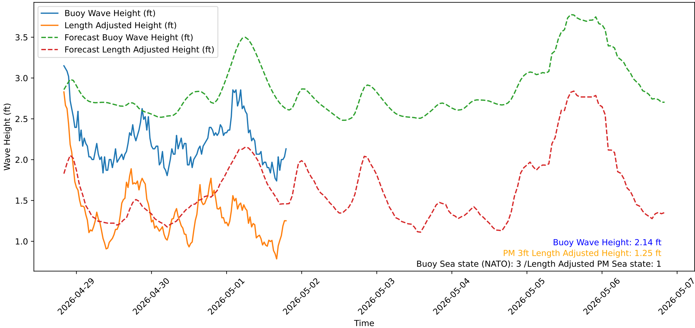
Wave Heights over Time for Green Beach at 2026-05-01 19:51:16
