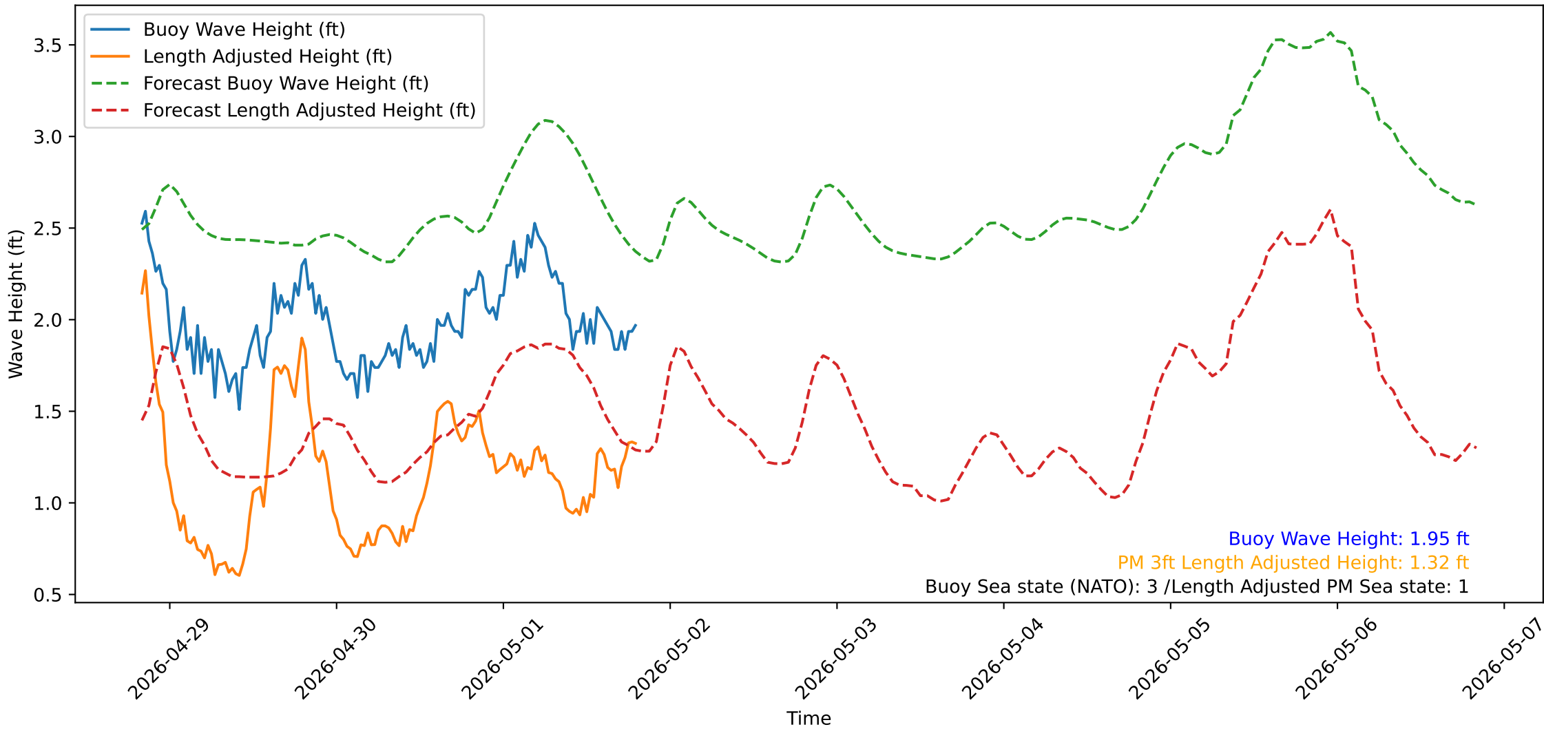
Wave Heights over Time for Red Beach at 2026-05-01 19:50:53
