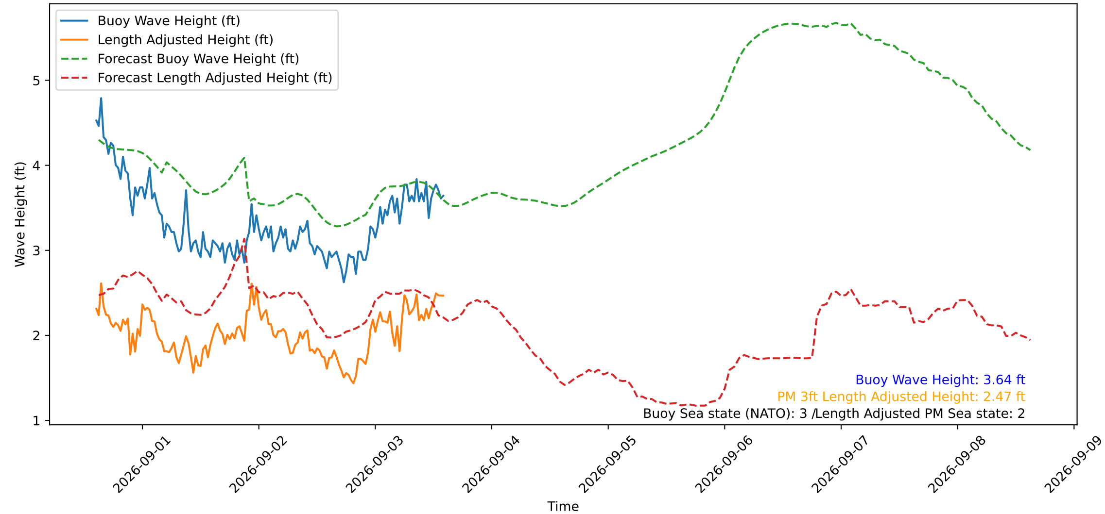
Wave Heights over Time for Oceanside Harbor at 2026-09-03 14:40:30
