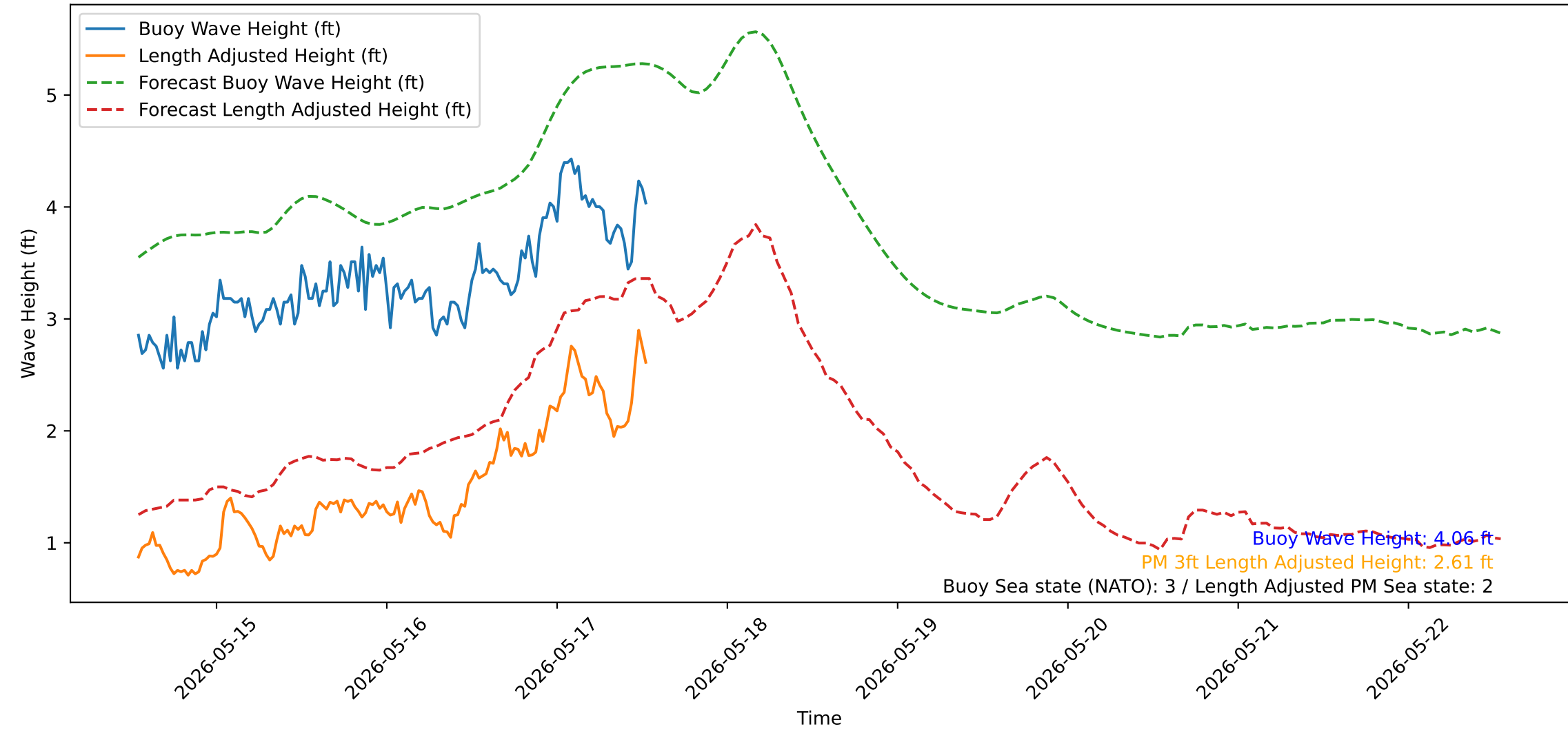
Wave Heights over Time for Green Beach at 2026-05-17 13:11:14
