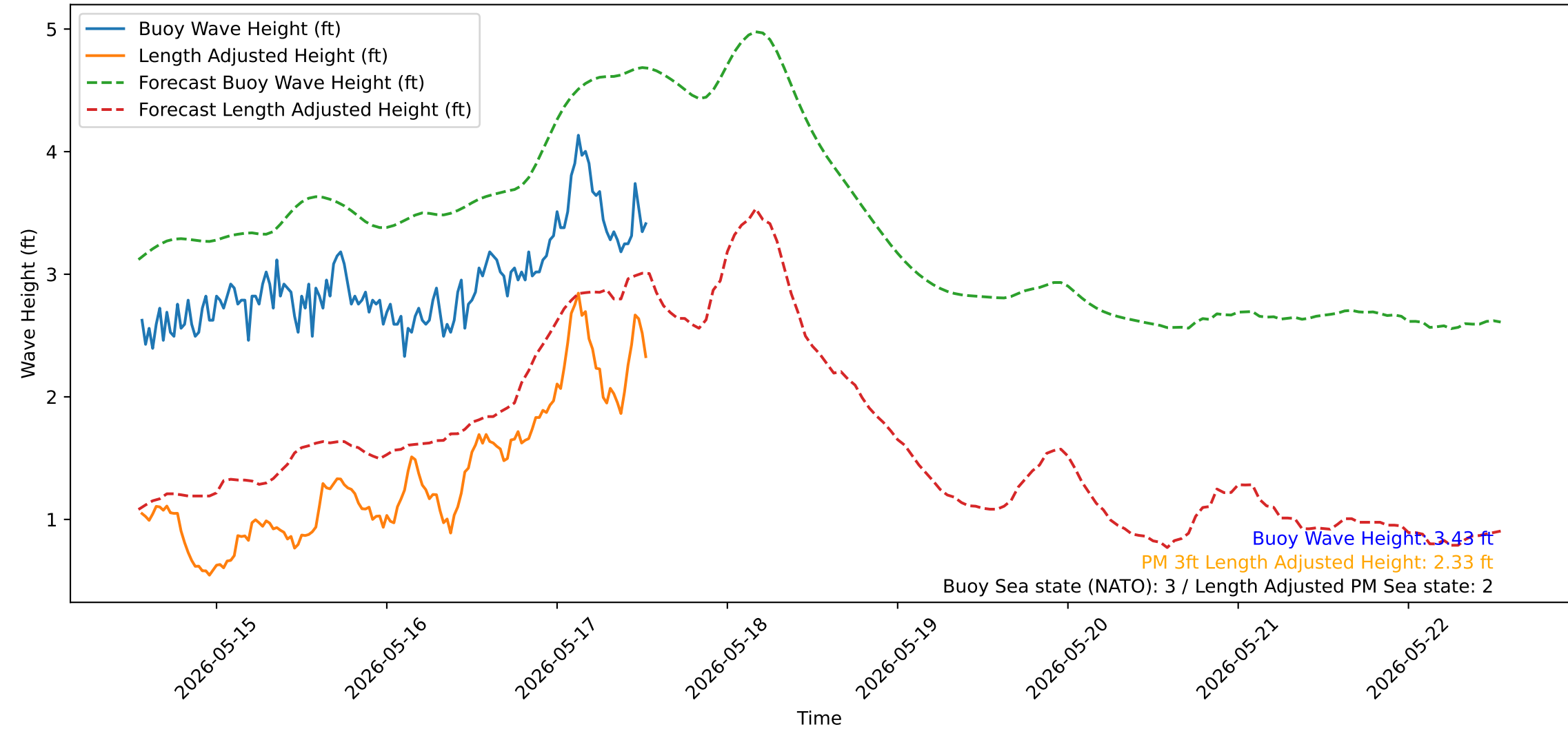
Wave Heights over Time for Red Beach at 2026-05-17 13:10:51
