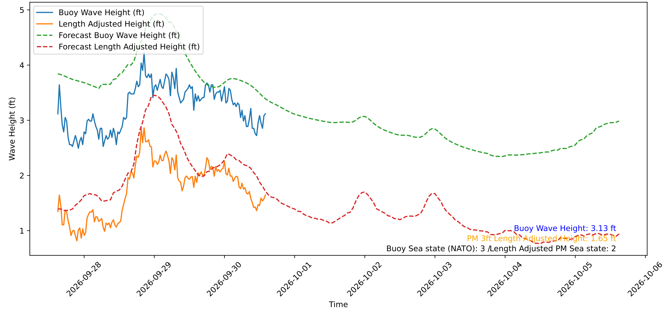
Wave Heights over Time for Oceanside Harbor at 2026-09-30 14:50:29
