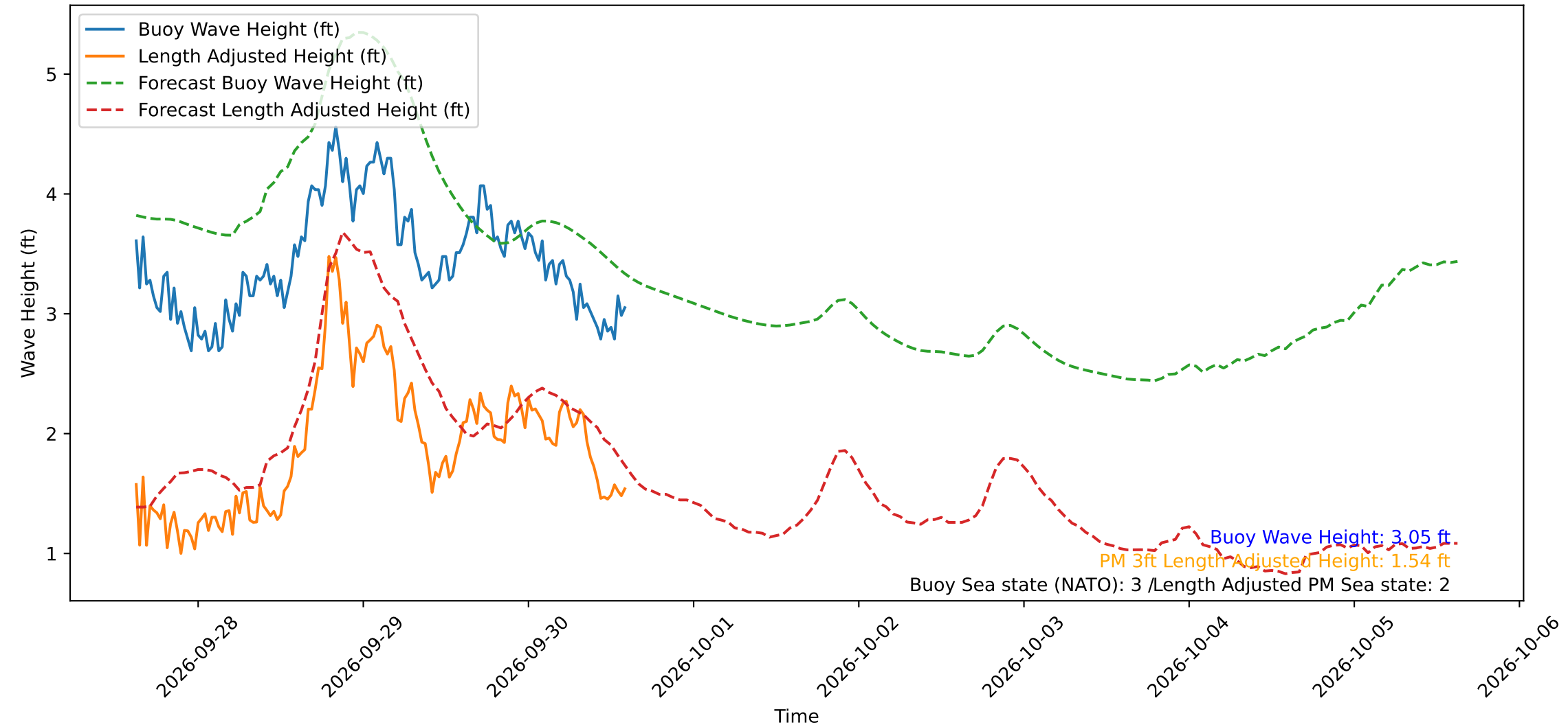
Wave Heights over Time for Green Beach at 2026-09-30 14:51:14
