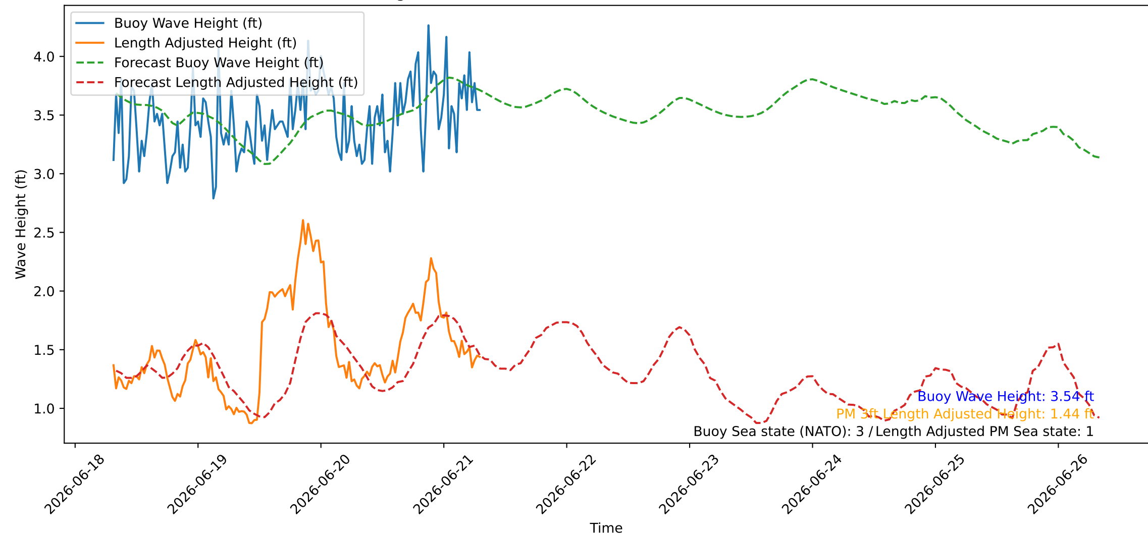
Wave Heights over Time for Oceanside Harbor at 2026-06-21 07:40:26
