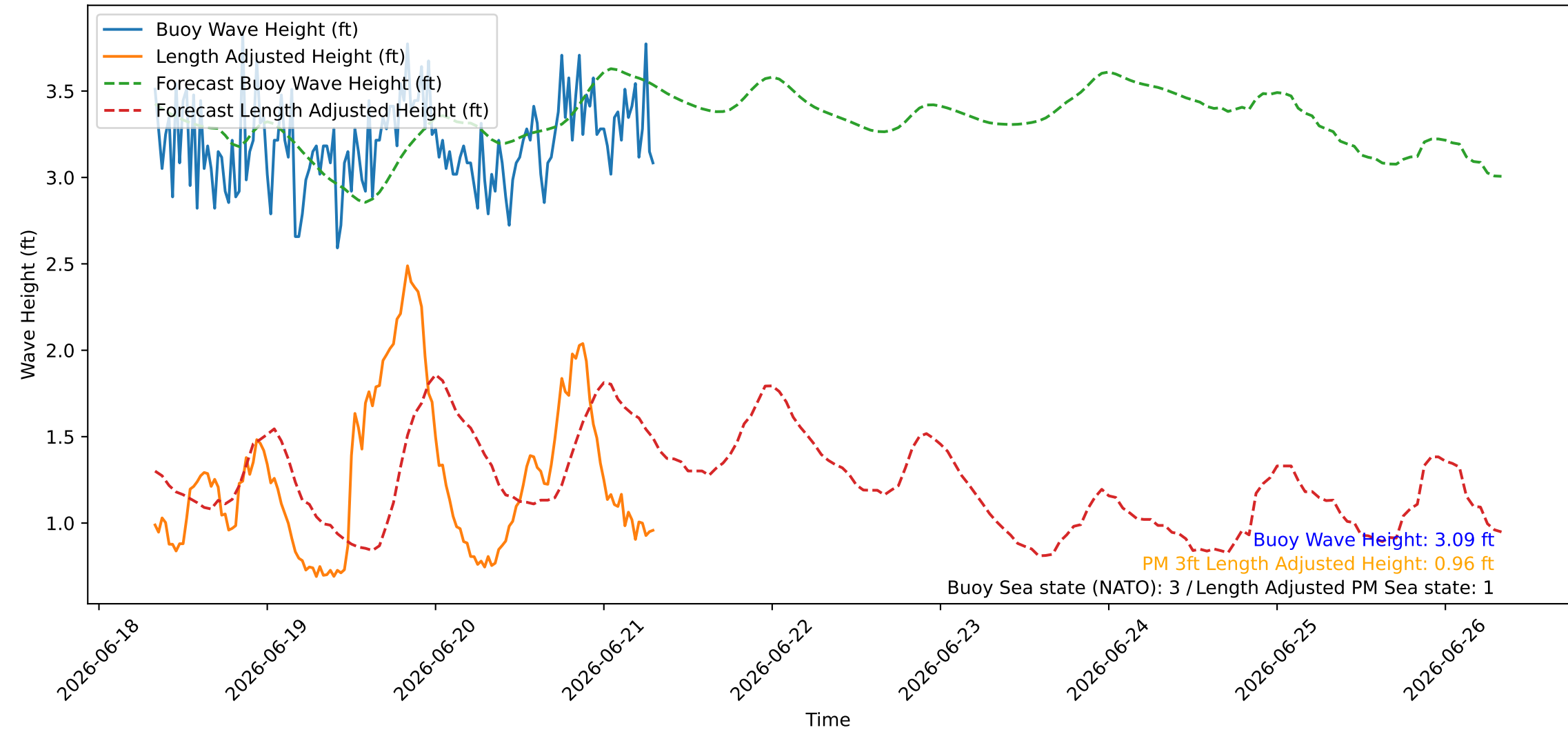
Wave Heights over Time for Red Beach at 2026-06-21 07:40:46
