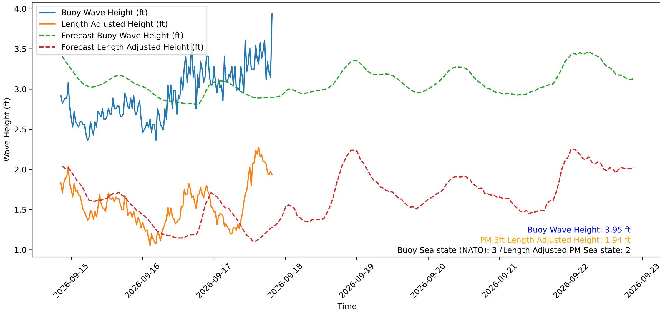
Wave Heights over Time for Oceanside Harbor at 2026-09-17 20:30:29
