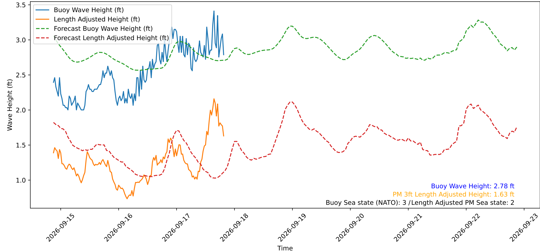
Wave Heights over Time for Red Beach at 2026-09-17 20:30:49
