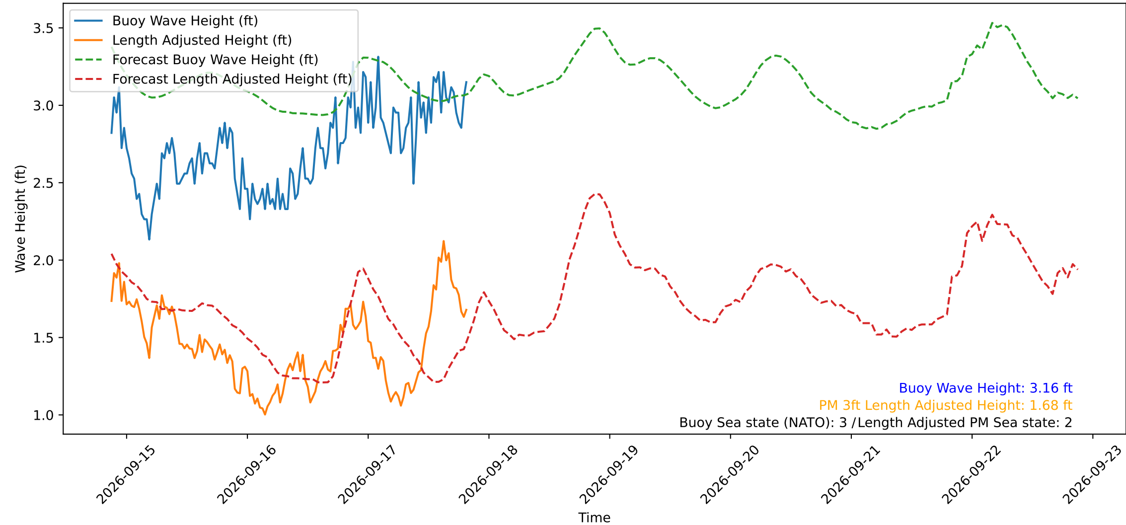
Wave Heights over Time for Green Beach at 2026-09-17 20:31:11
