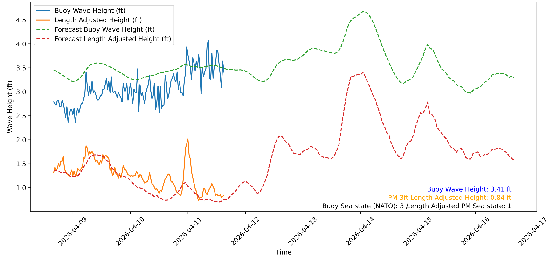
Wave Heights over Time for Green Beach at 2026-04-11 15:51:14
