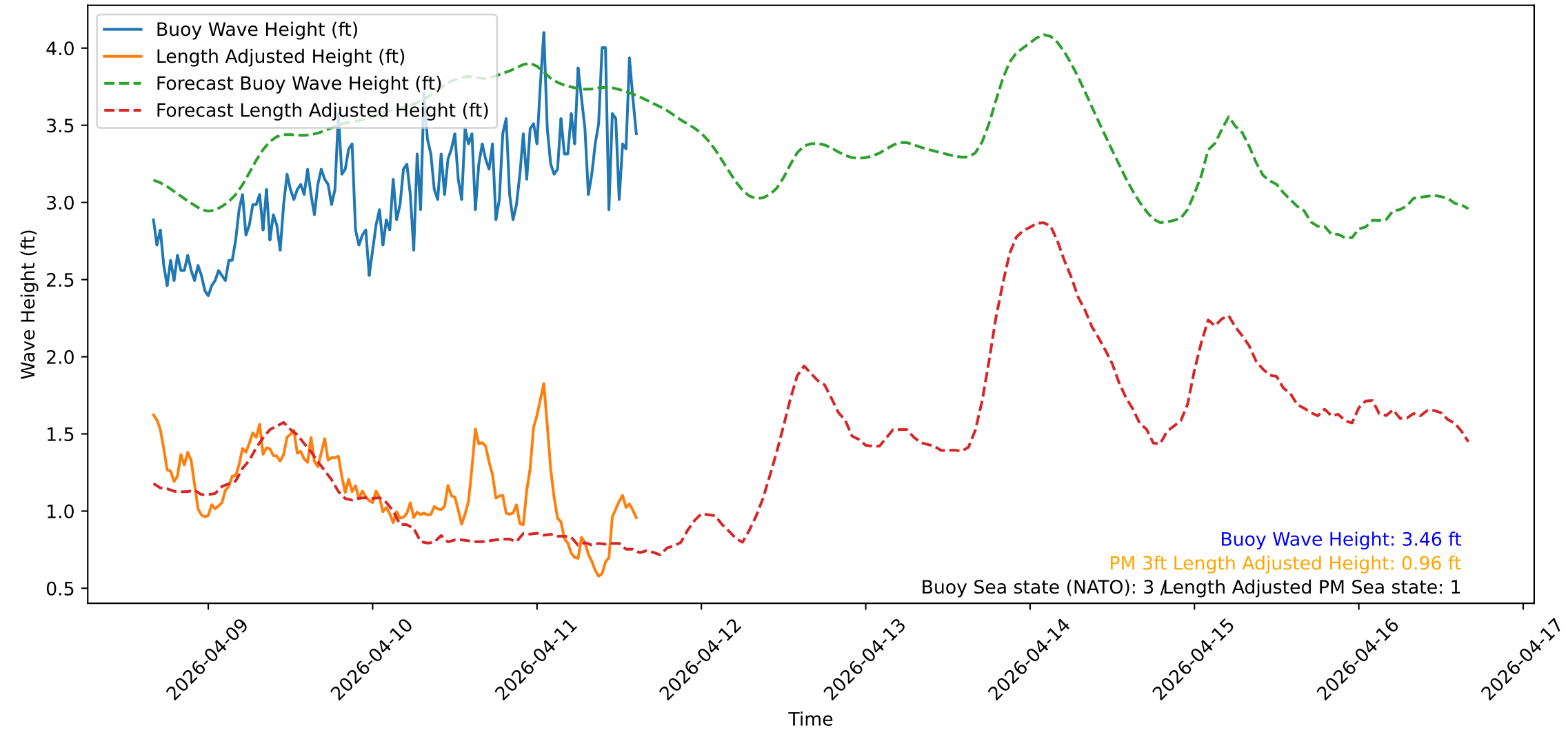
Wave Heights over Time for Red Beach at 2026-04-11 15:50:51
